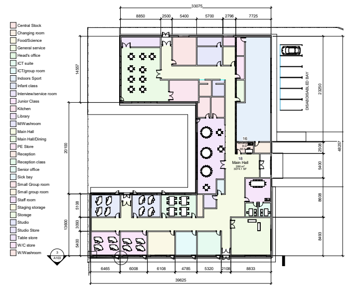
Ground floor 1 : 250
