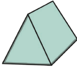
prism trionglog
