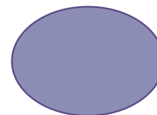
hirgrwn
