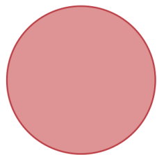
cylch
