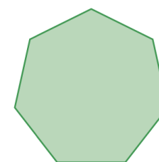
heptagon
