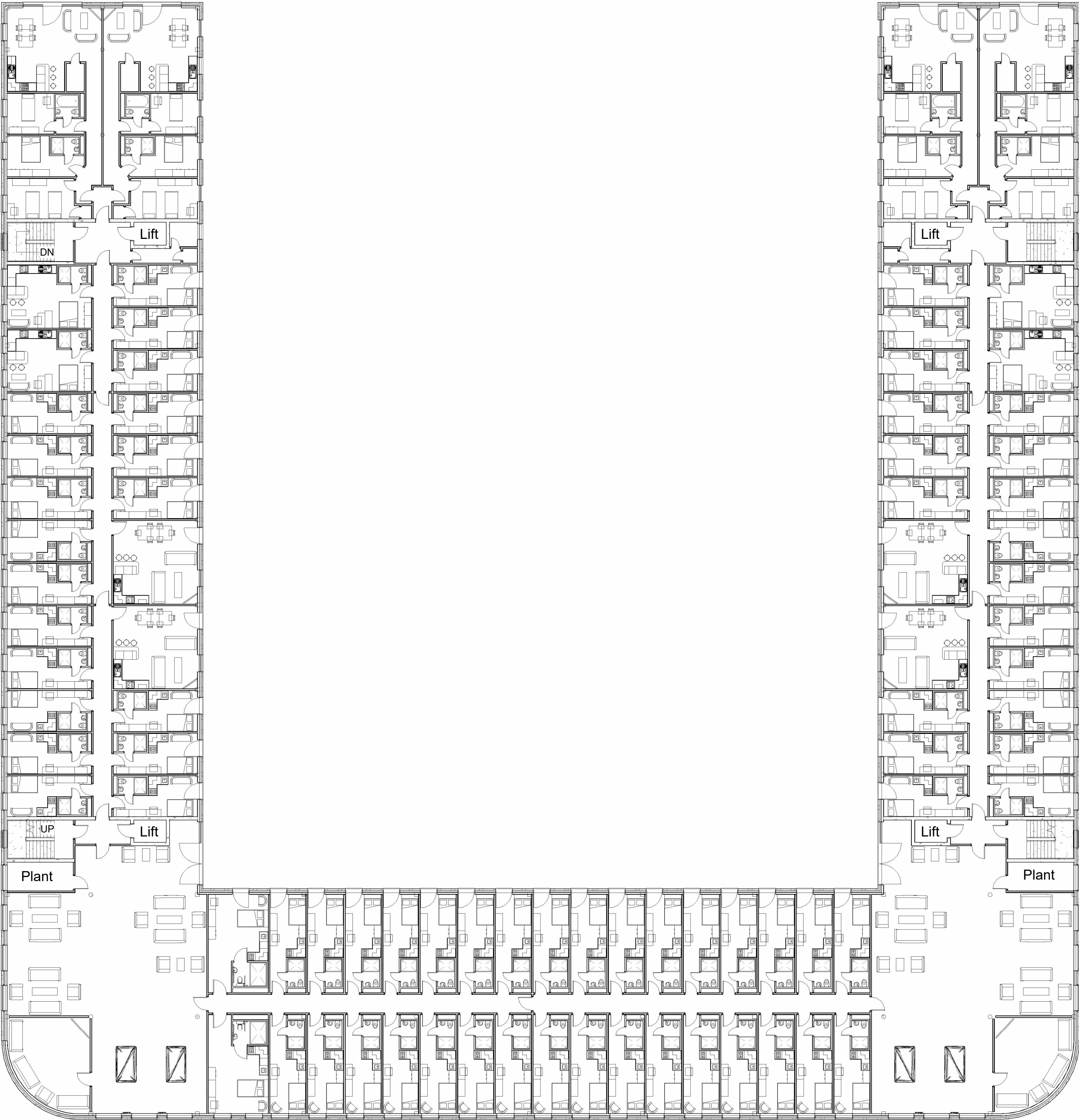
Second Floor Plan 1 : 200
