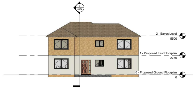
② North Elevation 1 : 100
