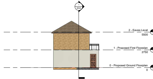
④ West Elevation 1 : 100
