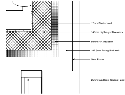
1 Proposed Section Callout Detail 1:5
