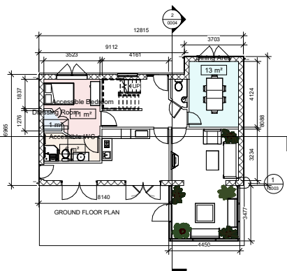
① 0 - Proposed Ground Floorplan 1 : 100
