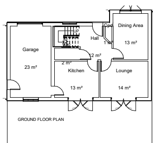
① 0 - Ground Floor 1 : 100
