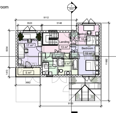
② 1 - Proposed First Floorplan 1 : 100
