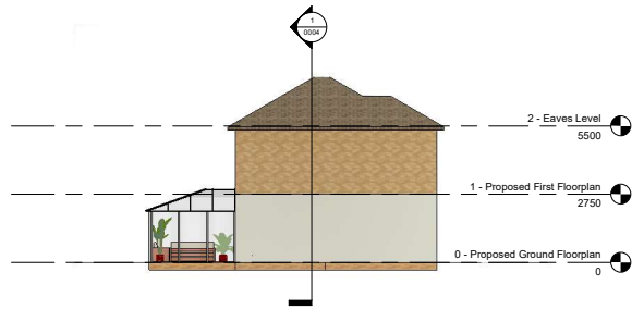
① East Elevation 1 : 100
