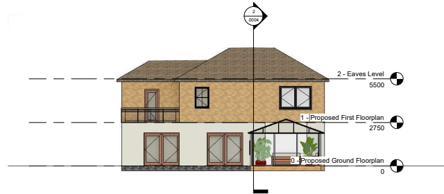
③ South Elevation 1 : 100
