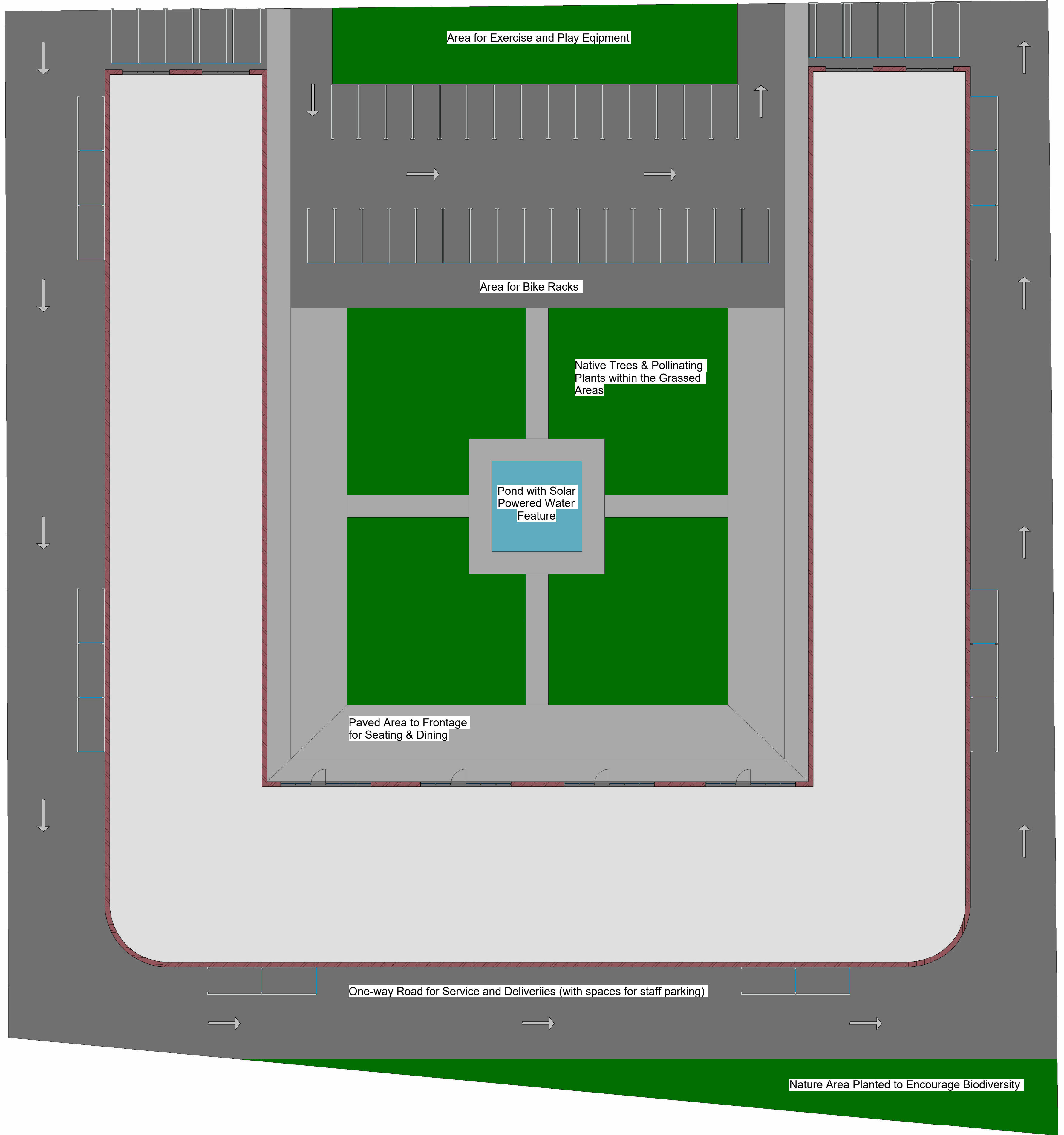
Detailed Site Layout Plan 1 : 200
