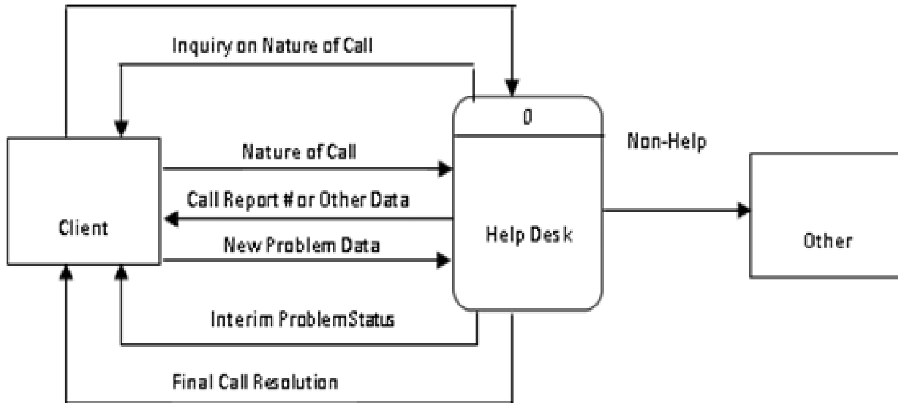
Context Diagram
