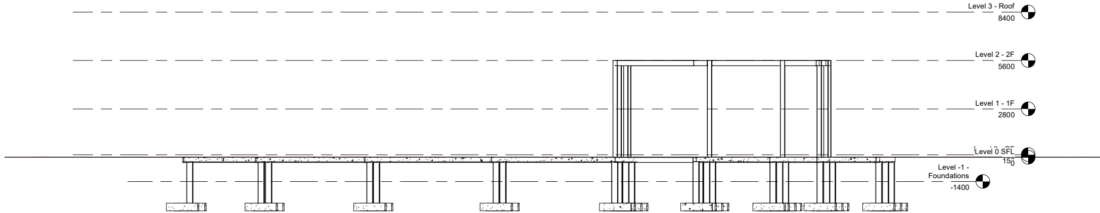
1 East (Structural) 1 : 100
