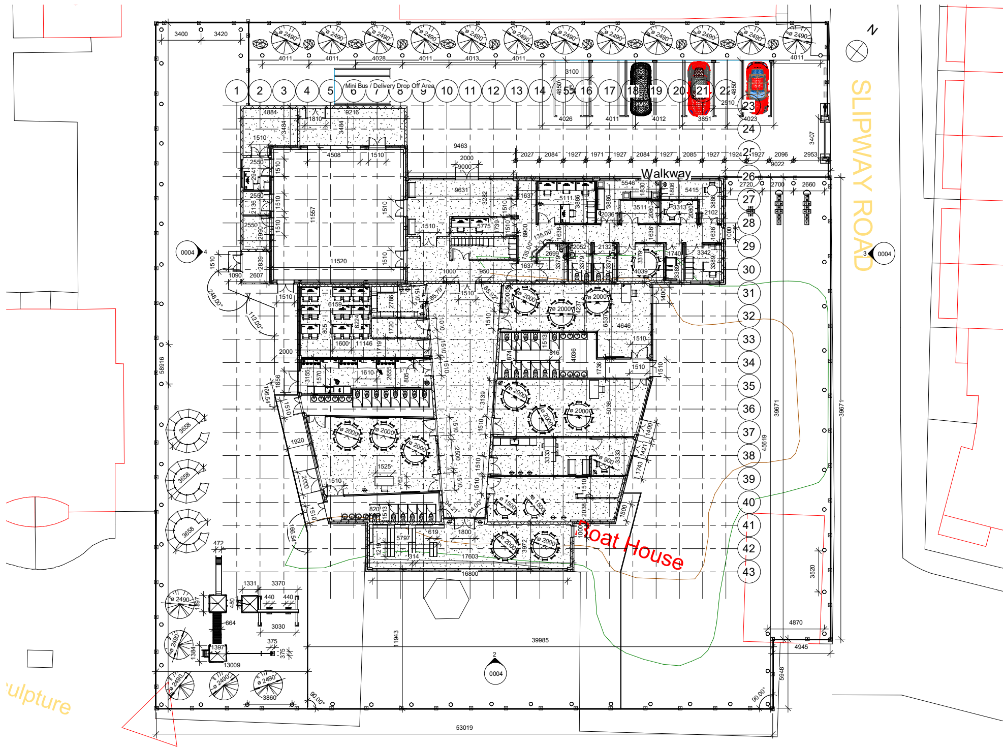
1 Level 0 - SFL & DATA 1 : 150 (Surface Floor Level)
