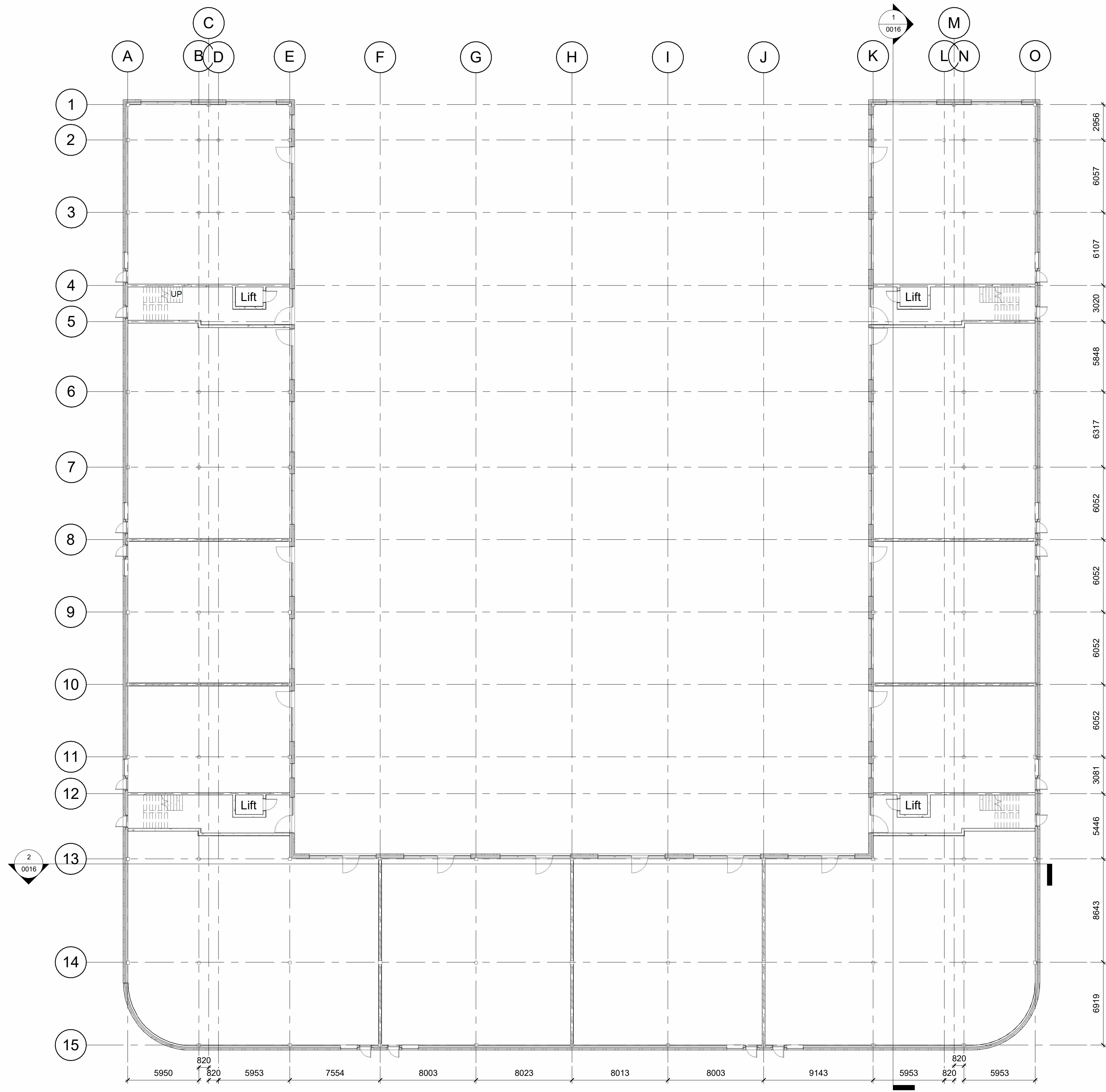
Ground Floor Plan 1 : 200
