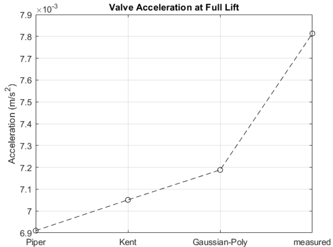
Figure 10.7 Acceleration at full lift for commercial and Gaussian-Poly (3600 x 3600), measured (360x360).
