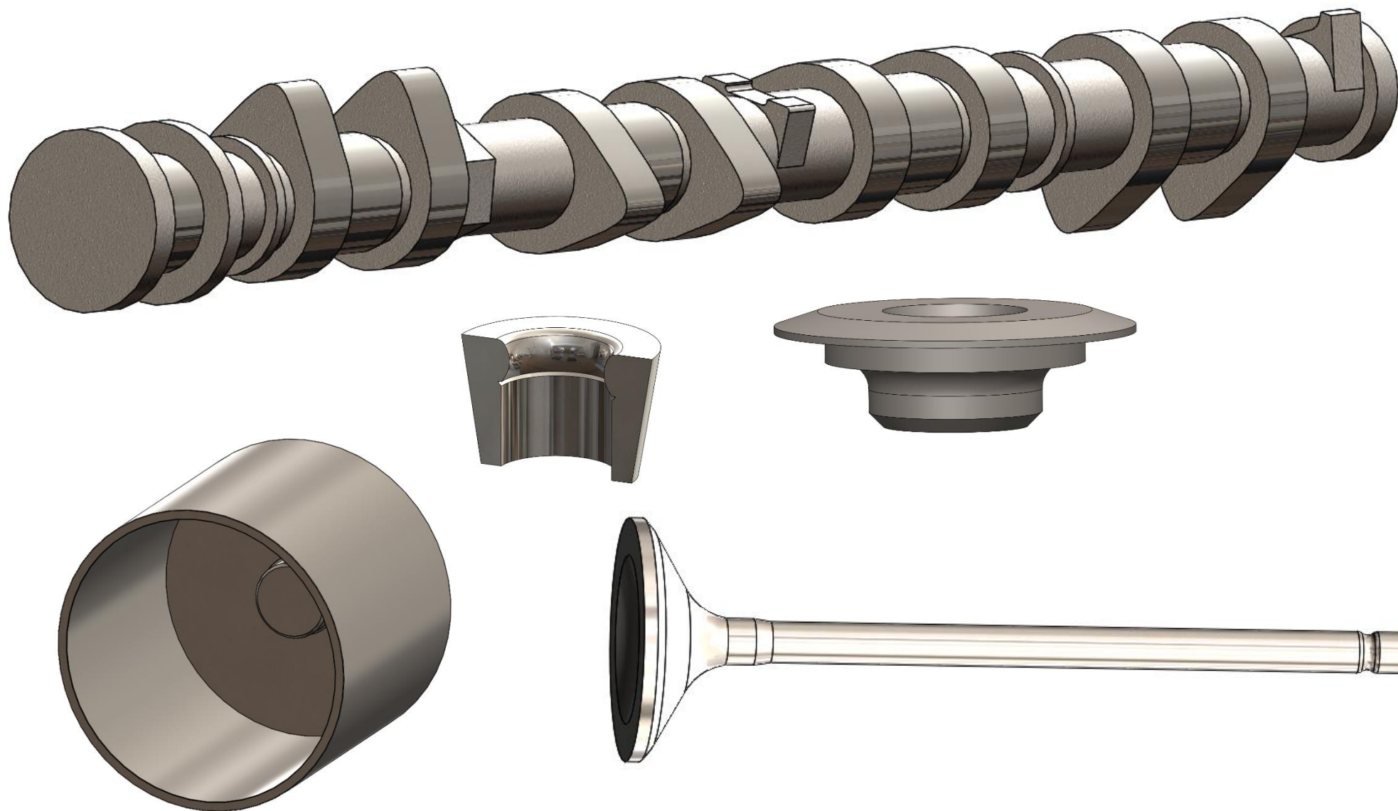
figure 16.23 Duratec camshaft, tappet bucket, collet, valve cap, inlet valve modelled in Solidworks
