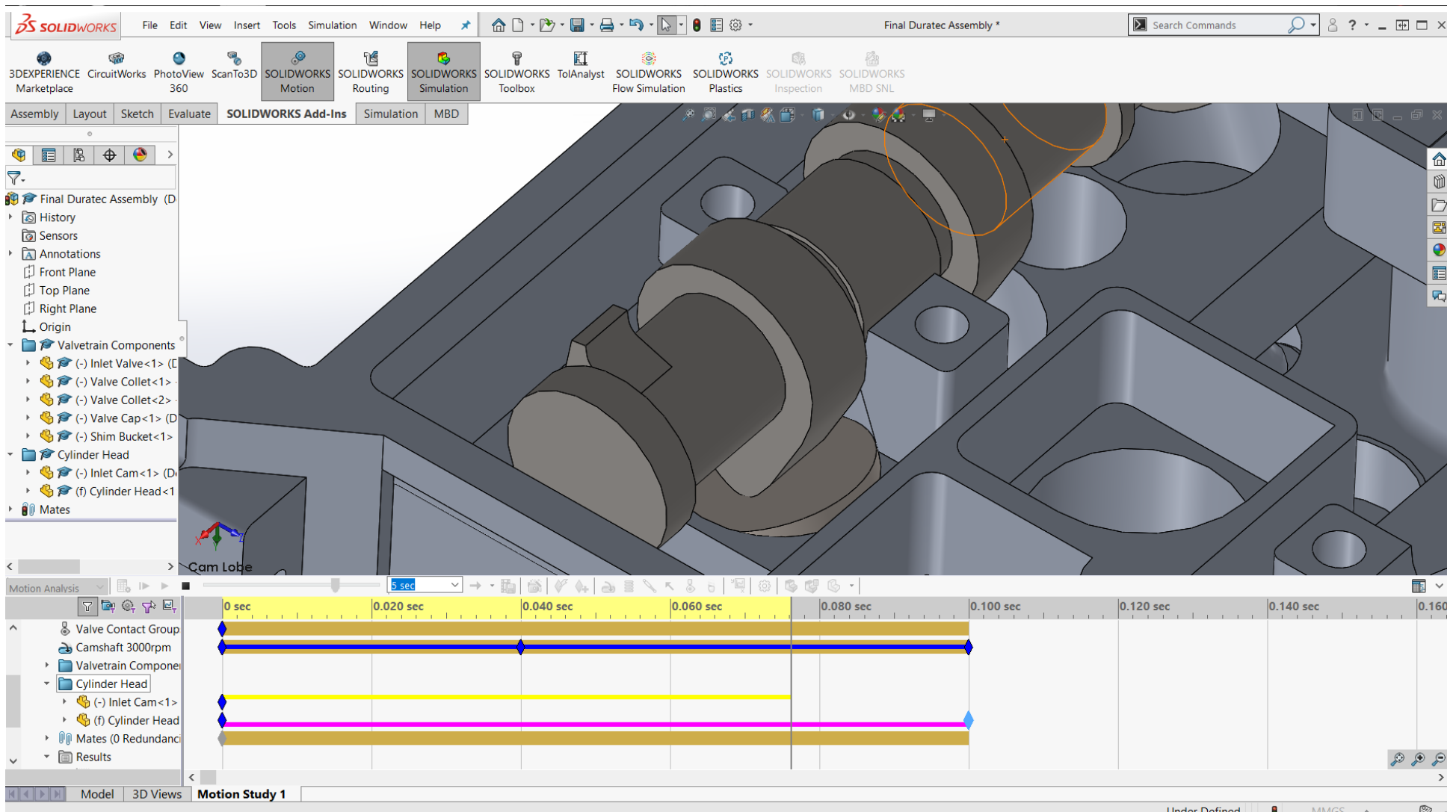
Figure 16.24 Cylinder head motion simulation set up to conduct FEA in Solidworks.
