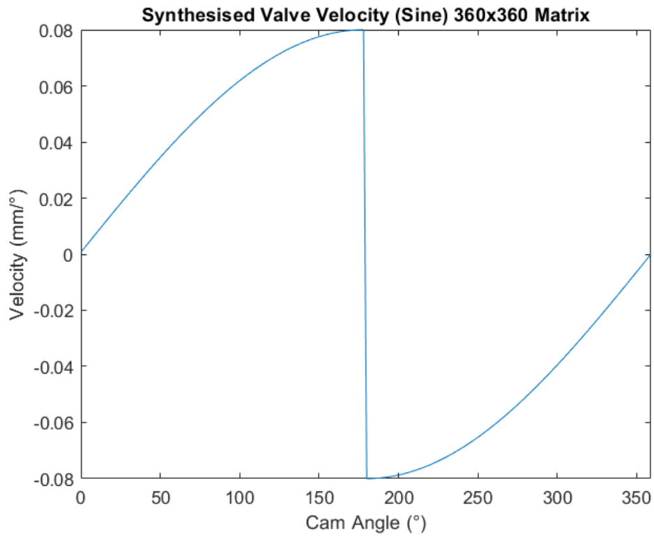
Figure 16.3 Synthesised valve velocity proves the pure valve lift matrix does not introduce noise.
