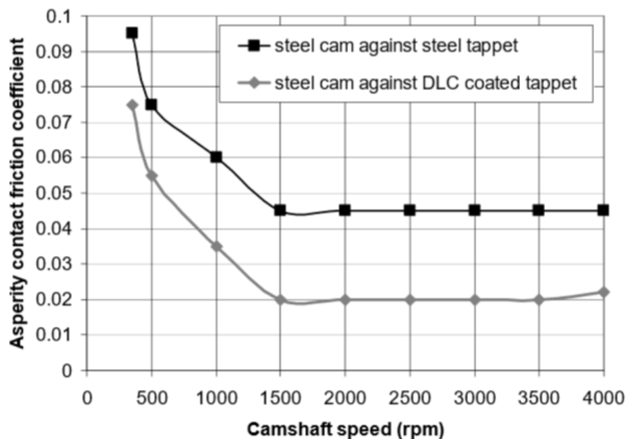
Figure 2.10 Change in friction coefficient (asperity contact) with different surface finishes (Calabretta and Cacciatore, 2010).
