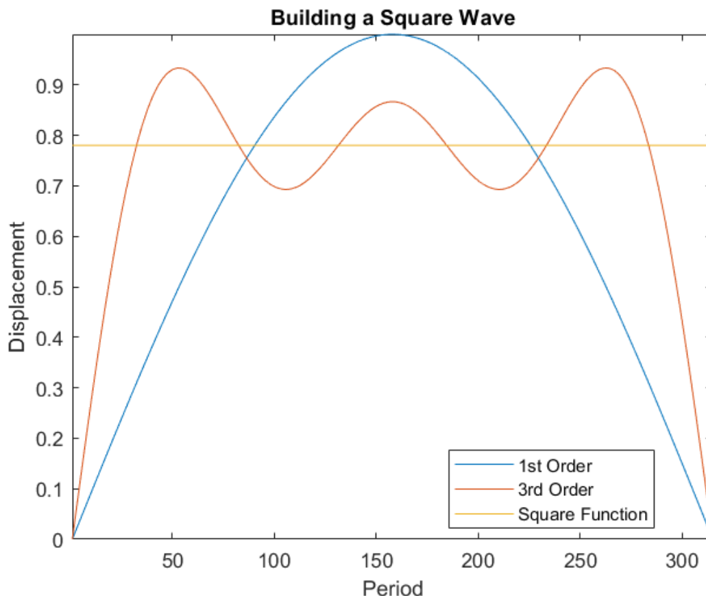
Figure 16.31 Building a square wave.
