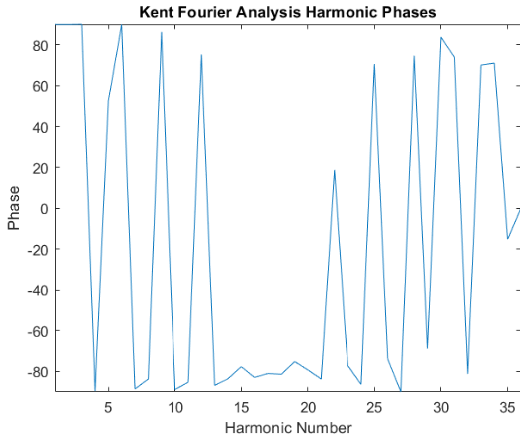
Figure 16.17 Phase plot of Fourier Series.
