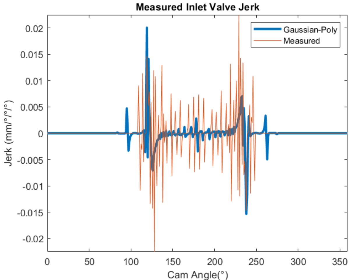
Figure 10.4 Comparison between Kent Cams and Piper Cams inlet valve jerk and jounce.
