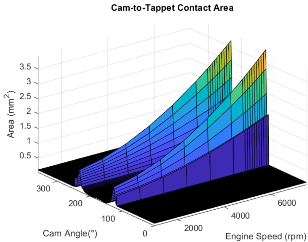
Figure 16.29 Area of contact.
