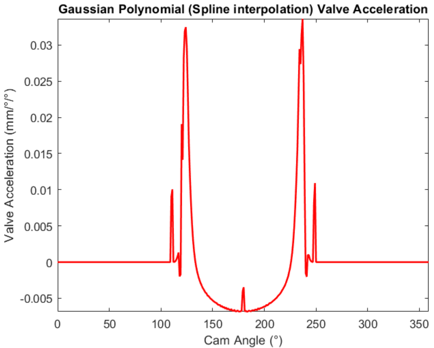
Figure 16.10 Gaussian Polynomial (3,600 x 3,600) with spline interpolation (non-shape-preserving). Yields improvement in noise over PCHIP.
