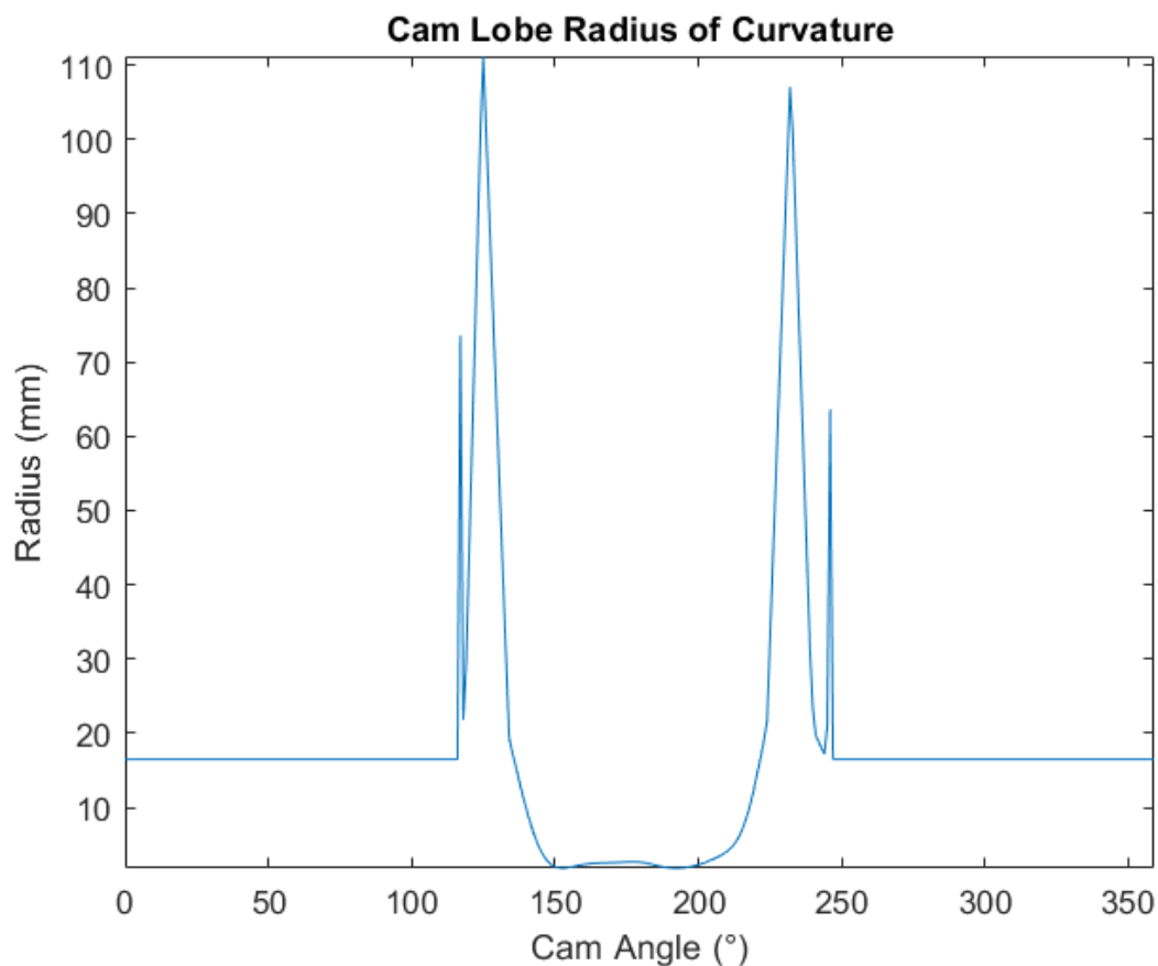
Figure 16.28 Radius of curvature (cam lobe).
