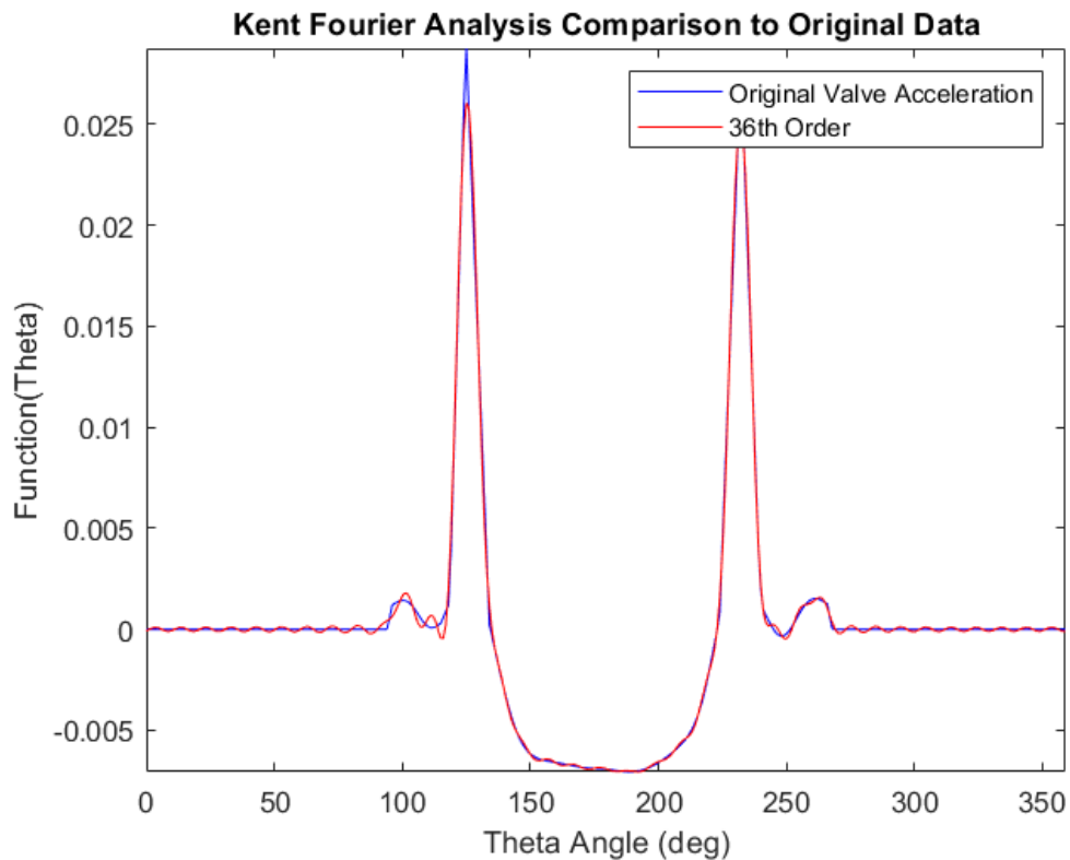
Figure 16.17 36 th order of acceleration convergence (requires higher order, more complex function).
