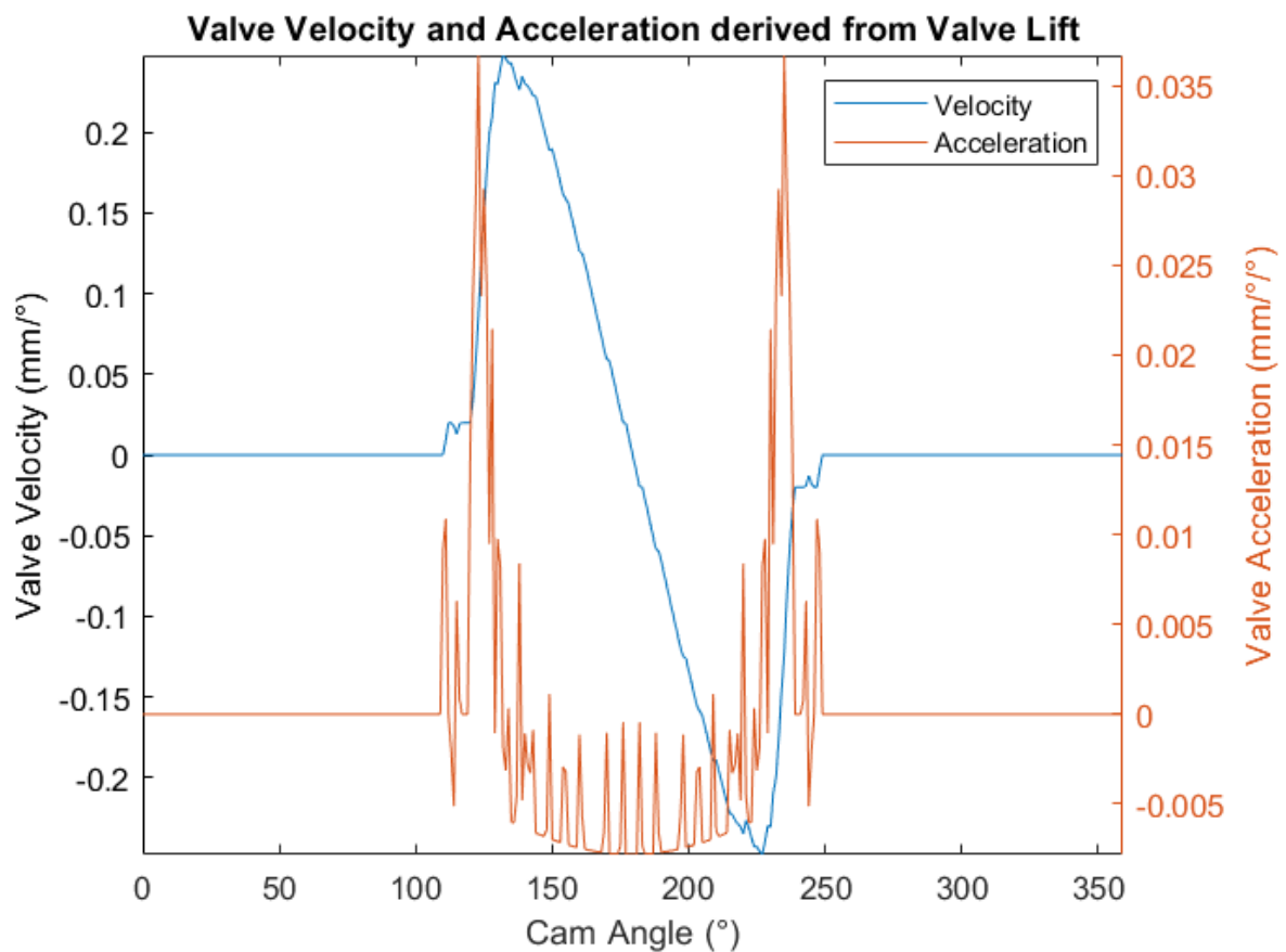
Figure 4.4 Valve velocity and valve acceleration derived from measured cam profile.
