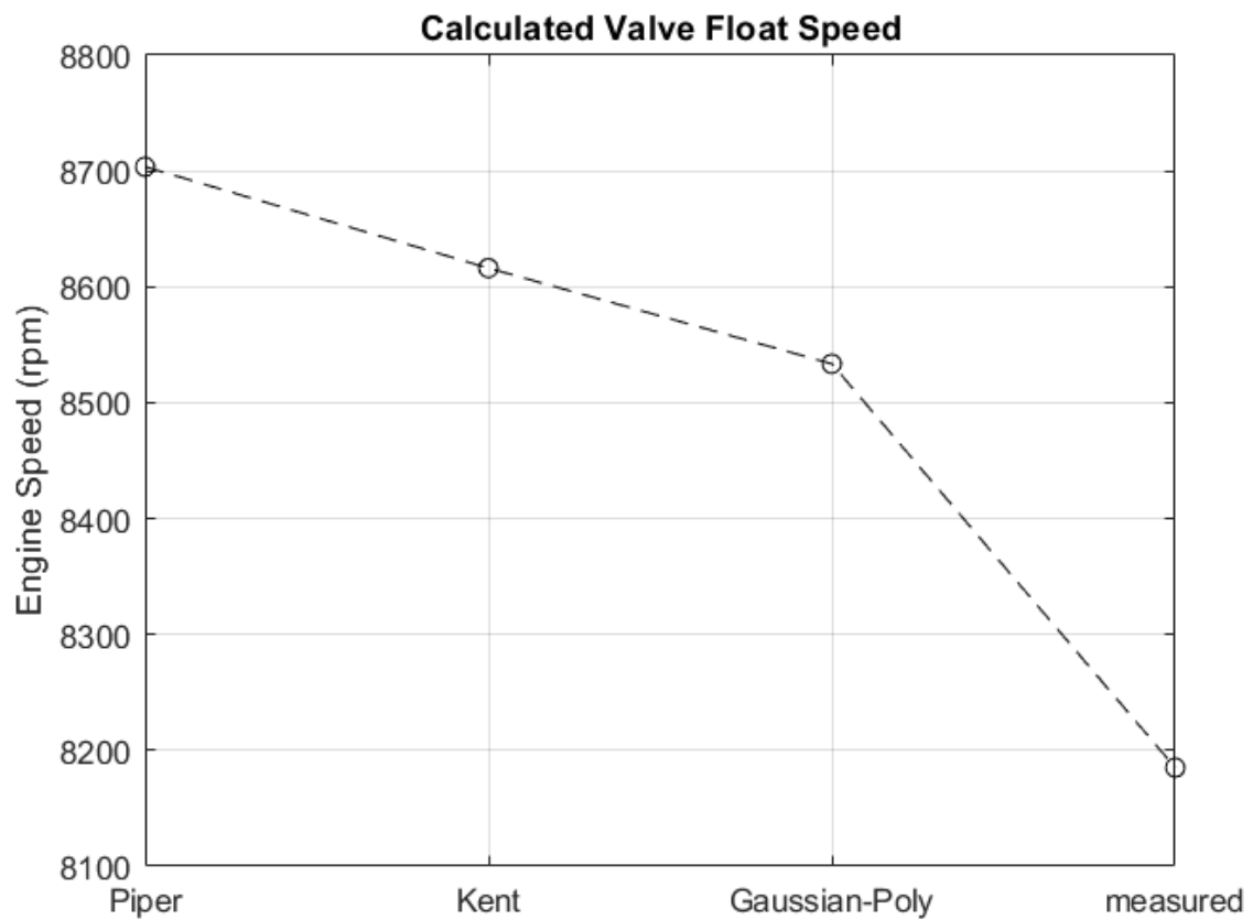
Figure 10.8 Valve float speed for commercial and Gaussian-Poly (3600 x 3600), measured (360x360).
