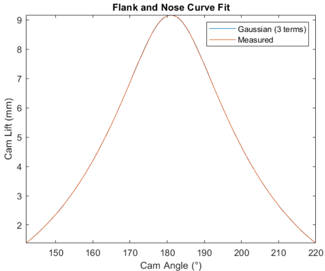
Figure 6.6 The flanks and nose of the cam profile. 3 term Gaussian curve-fit, fully converged.
