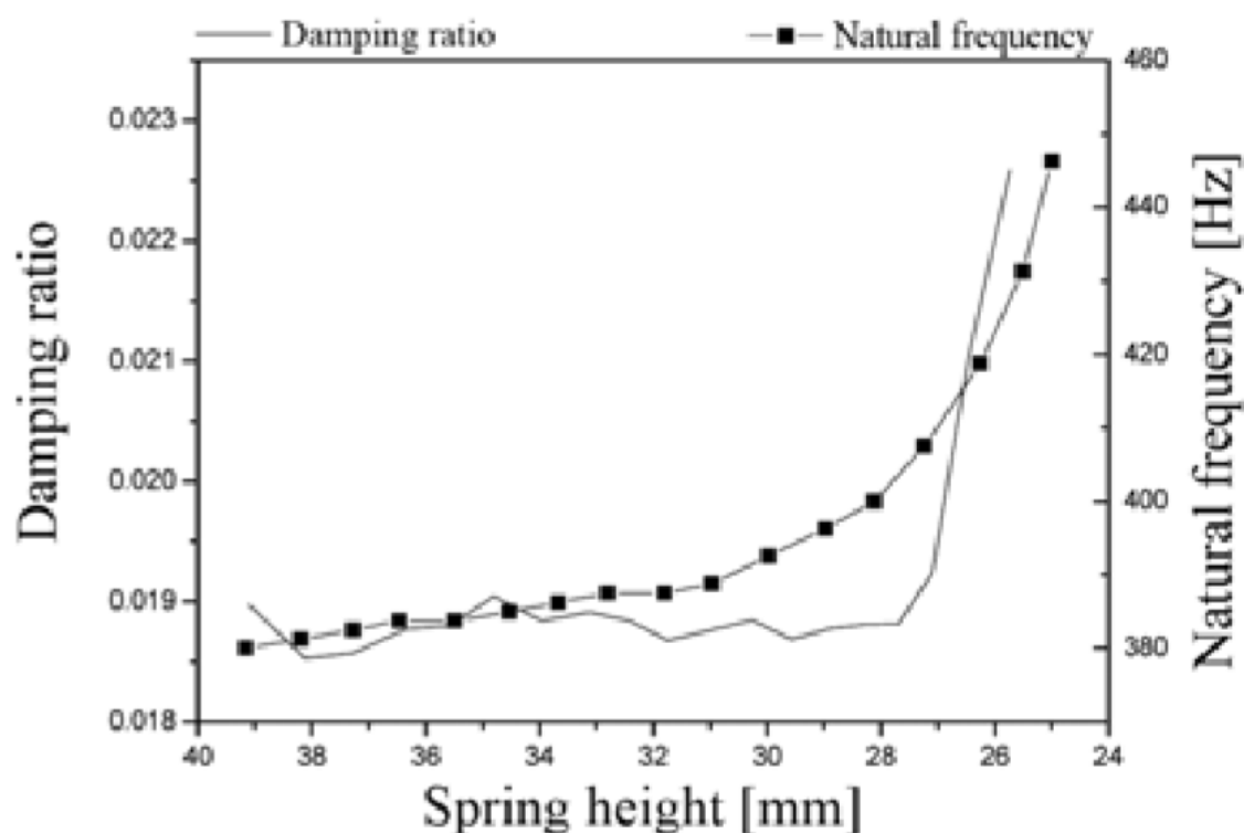
Figure 12.5 Compression spring natural frequency and damping ratio comparison (Liu and Kim, 2011).
