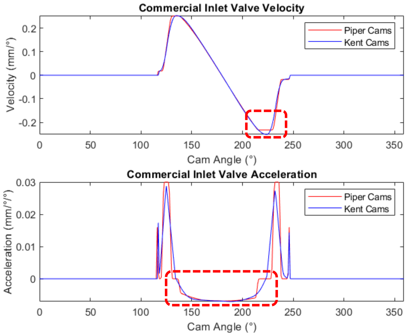
Figure 10.2 Comparison between Kent Cams and Piper Cams inlet valve velocity and acceleration.
