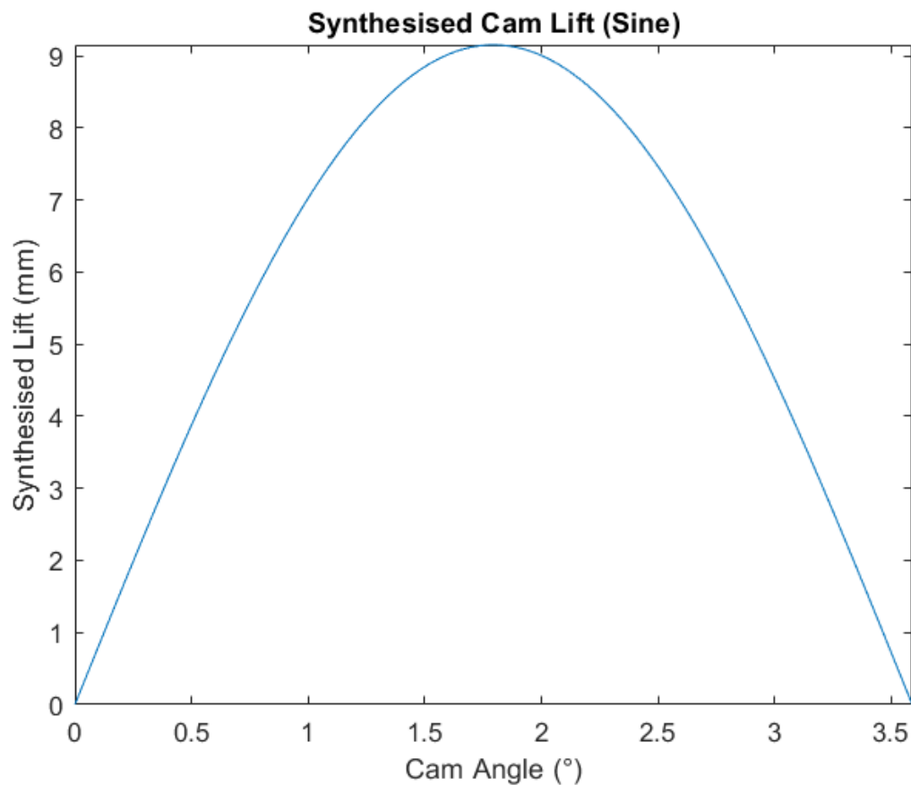
Figure 16.2 Sine Wave Plot for replicating cam Lift (before valve lift matrix).
