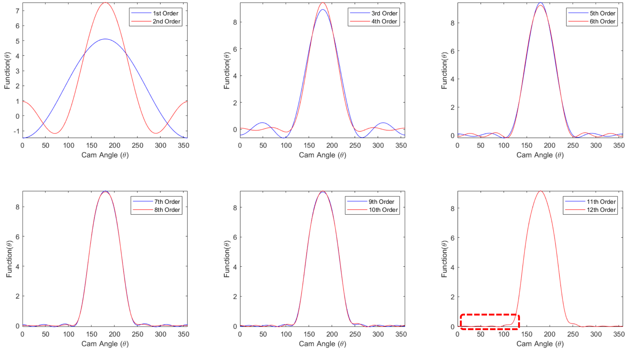
Figure 11.1 - Kent Cams Fourier series (1st to 12th order)
