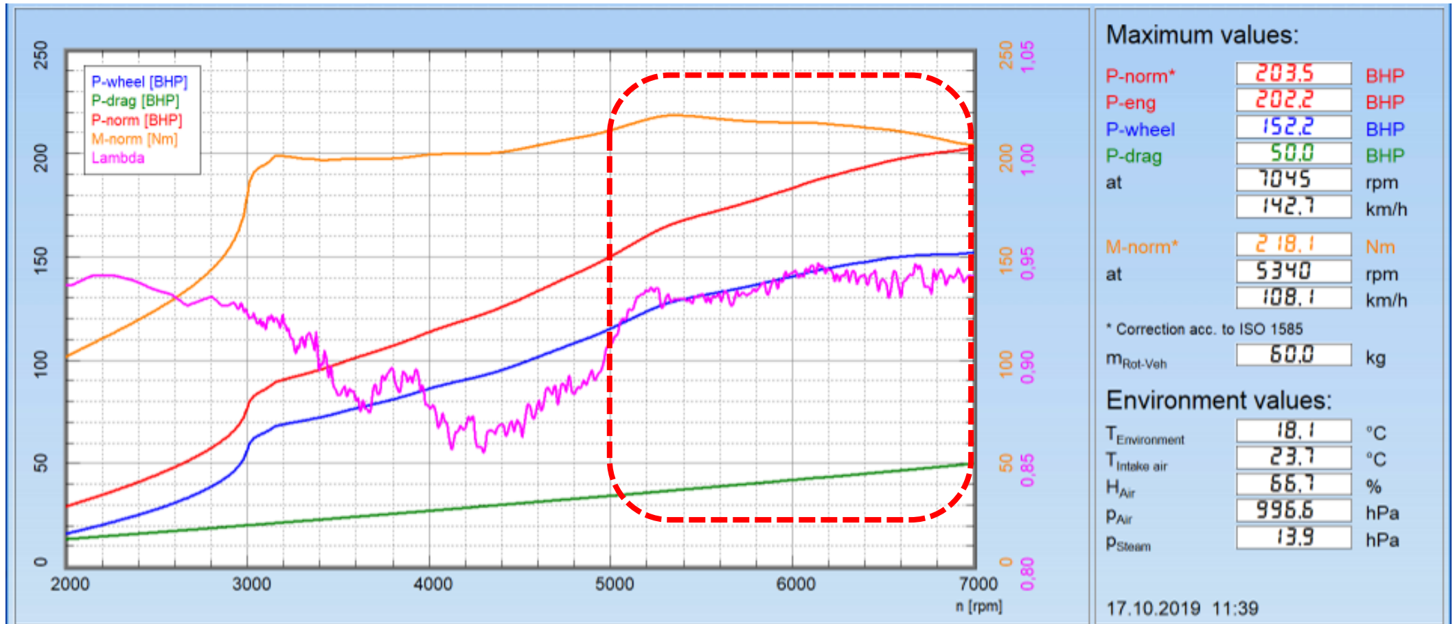
Figure 16.7 Chassis dynamometer print out of UWTSD MCR Race Car, where the lambda switches after 5,000rpm, indicating mapped engine speed range.
