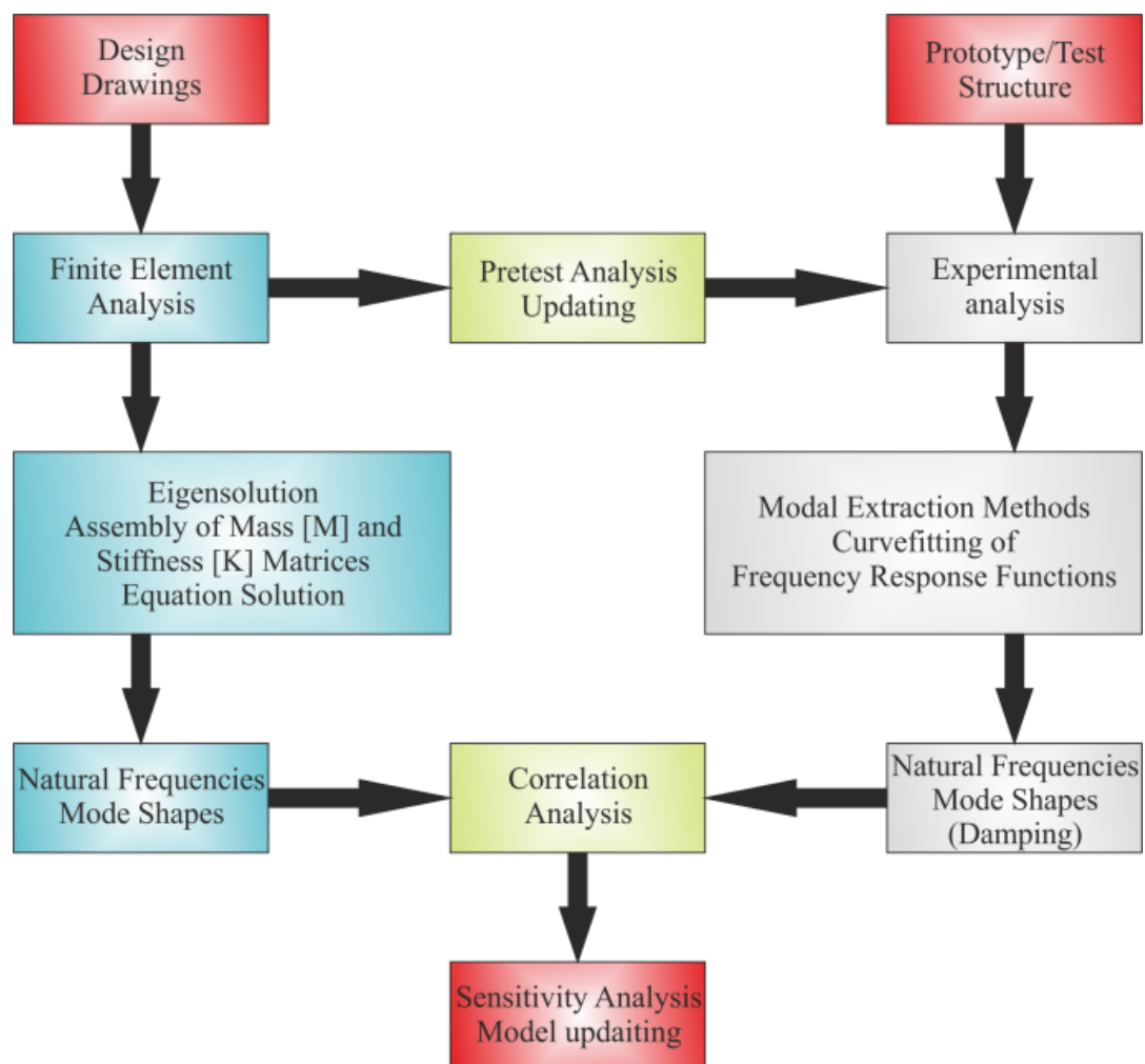
Figure 2.6 A typical flowchart for commercial modal analysis combining theoretical Finite Element Analysis (FEA) and Experimental Modal Analysis (EMA) (Lengvarský and Bocko, 2013).
