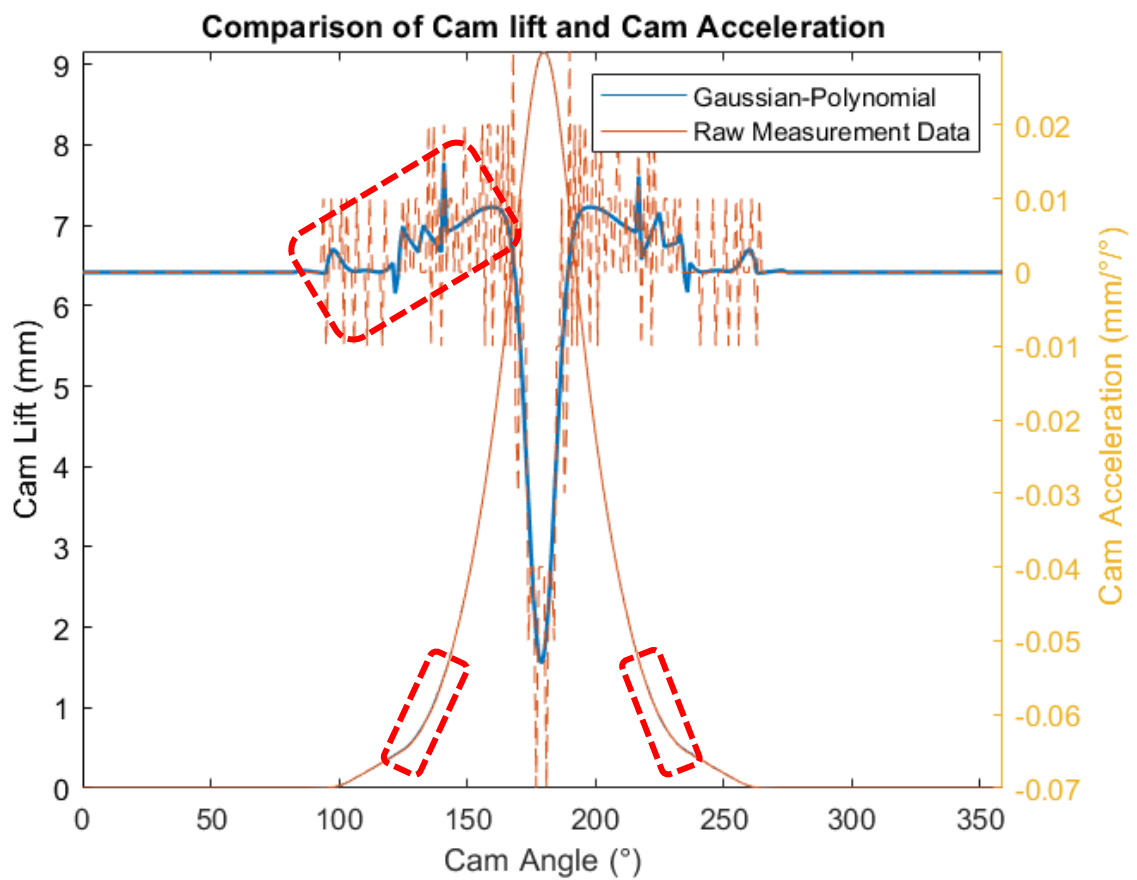
Figure 6.8 Final curve fit with good definition after “data patch” was applied to the highlighted sections.
