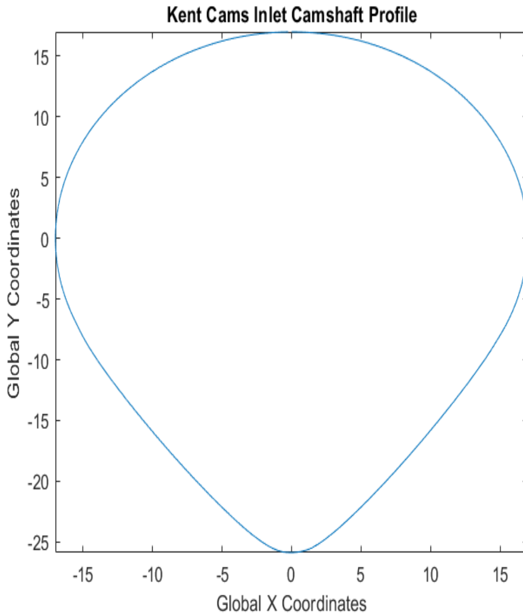
Figure 9.5 Cam lobe profile in polar form, given from the rotation of axes method.
