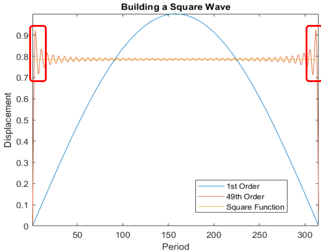
Figure 16.32 Building a square wave (49 th order).
