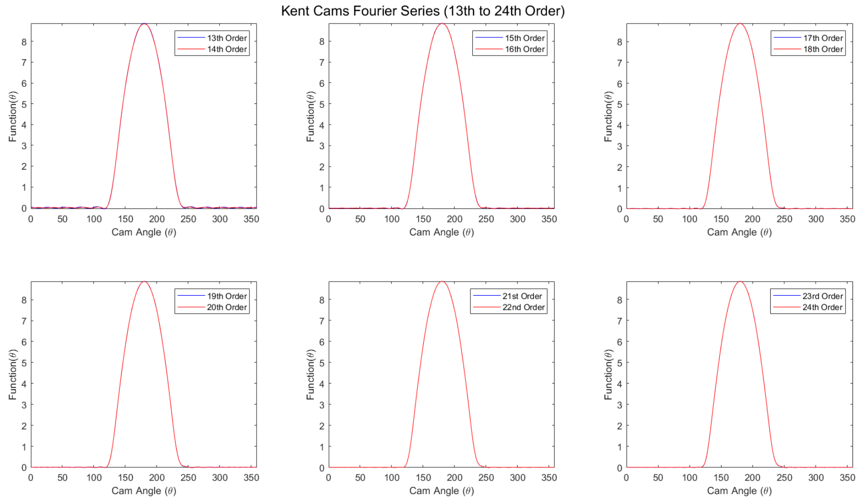
Figure 16.11 Convergence of Fourier series (orders 13 to 24).
