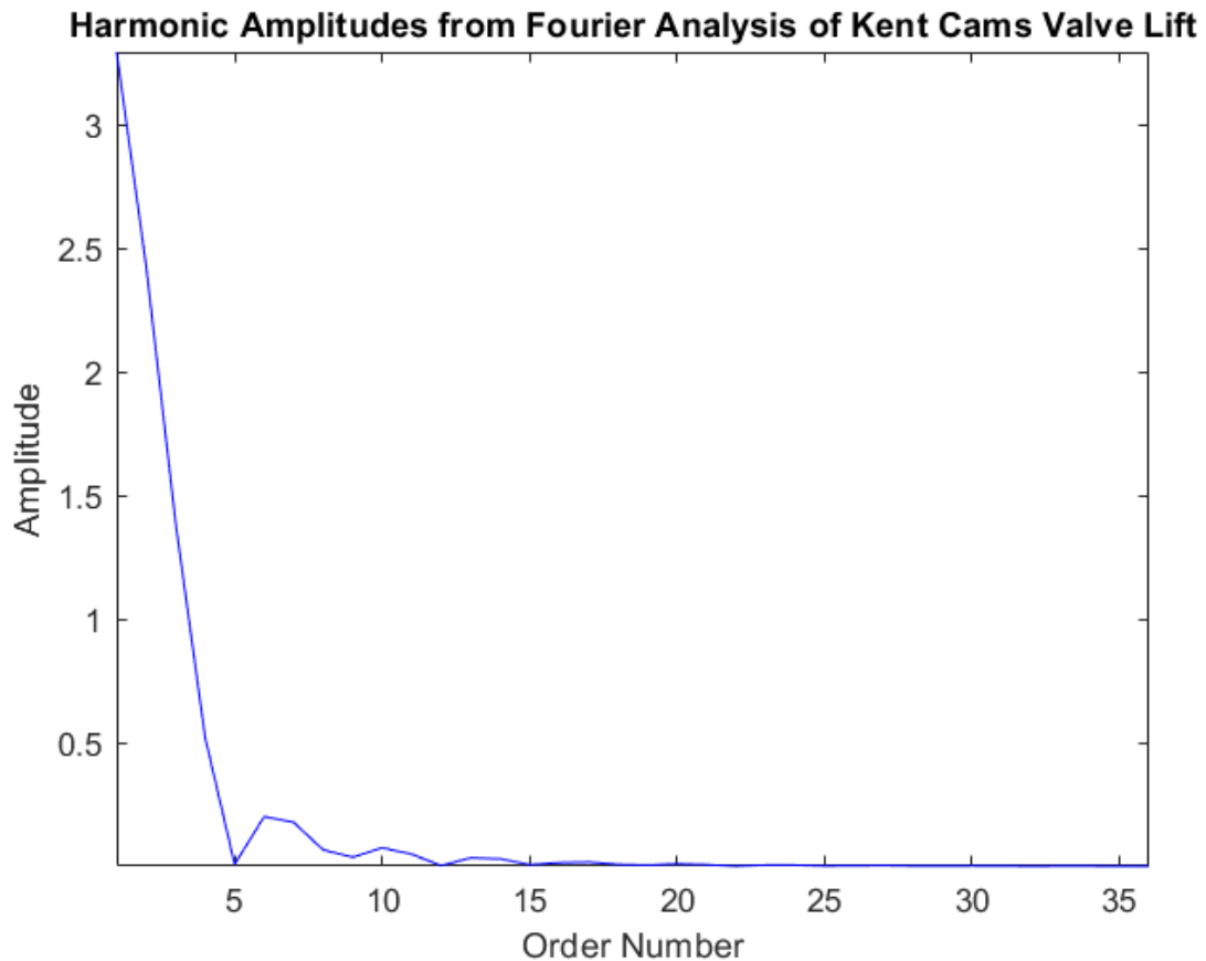
Figure 11.5 Harmonic amplitudes from Fourier analysis of Kent cams valve lift.
