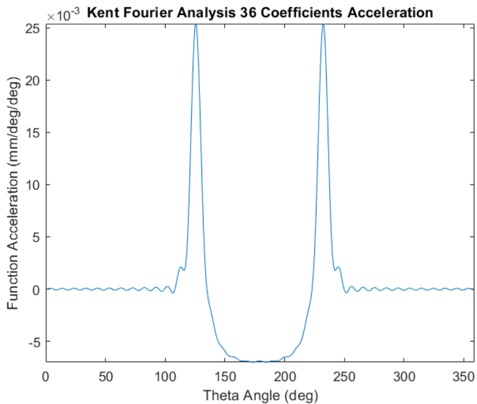
figure 16.14 2 nd order differential of Fourier series for valve lift. Shows little noise where measured does.
