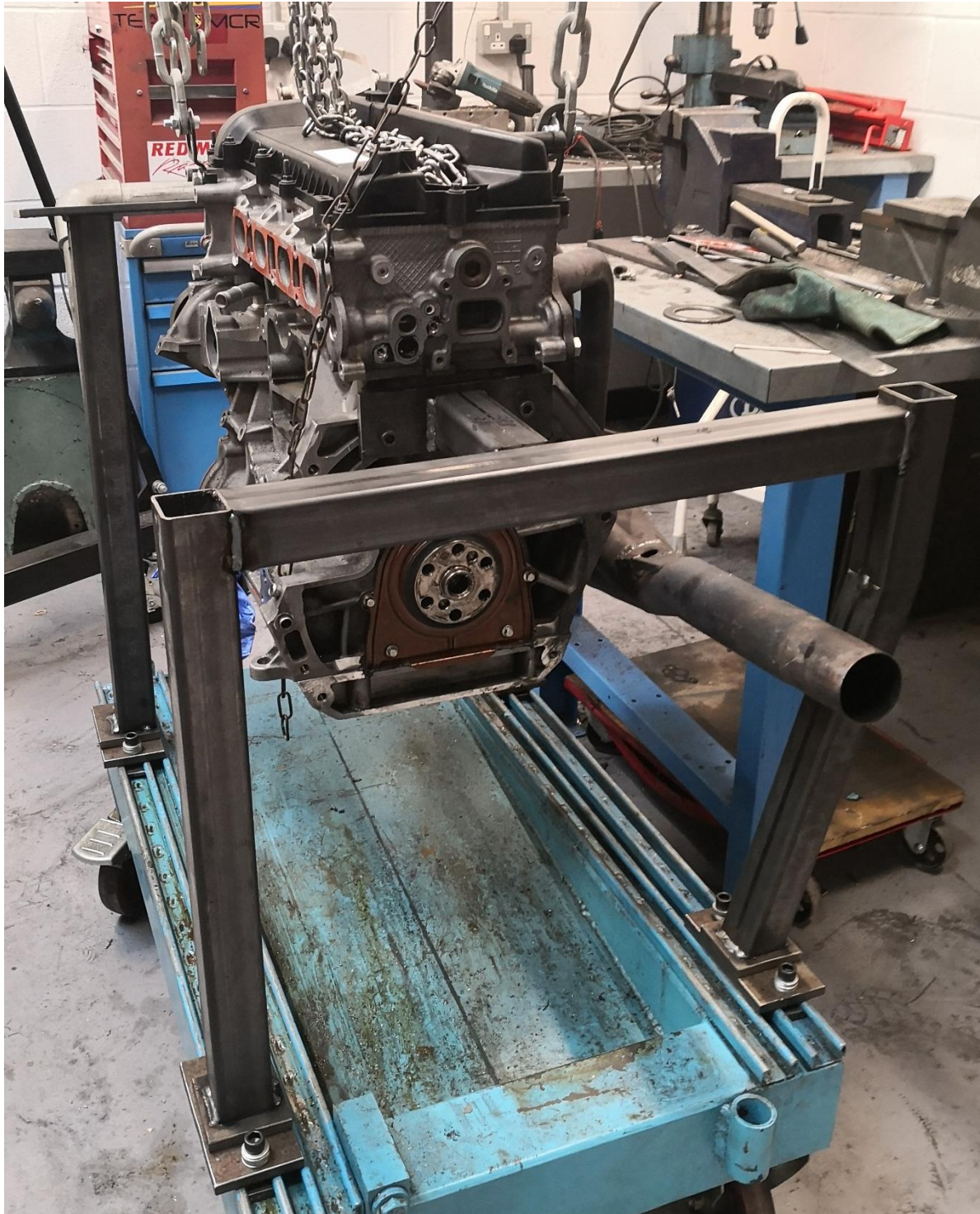
Figure 16.19 preparing the Duratec engine for future use on a dynamometer, rear of engine trolley.
