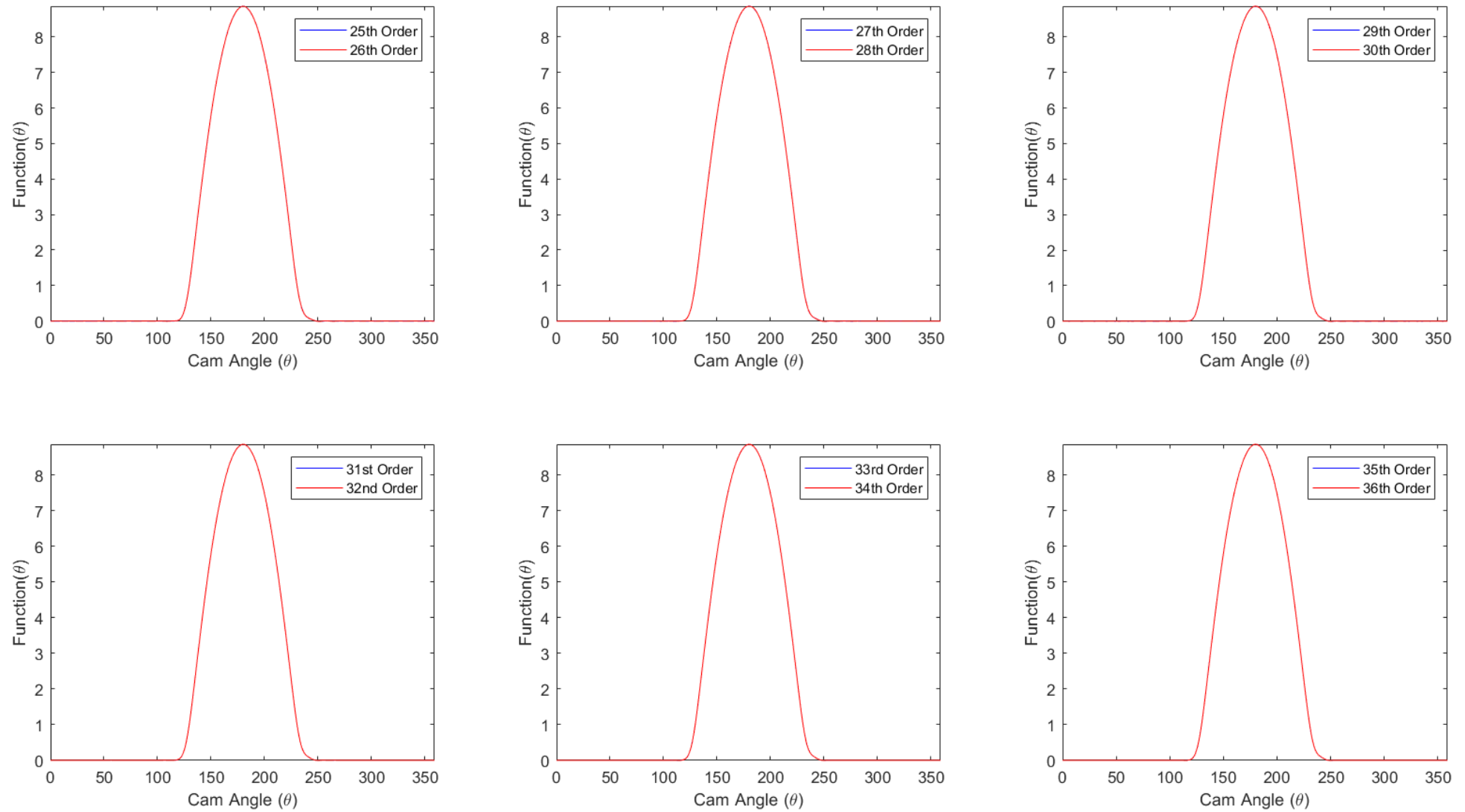
figure 16.12 Convergence of Fourier series (orders 25 to 36).
