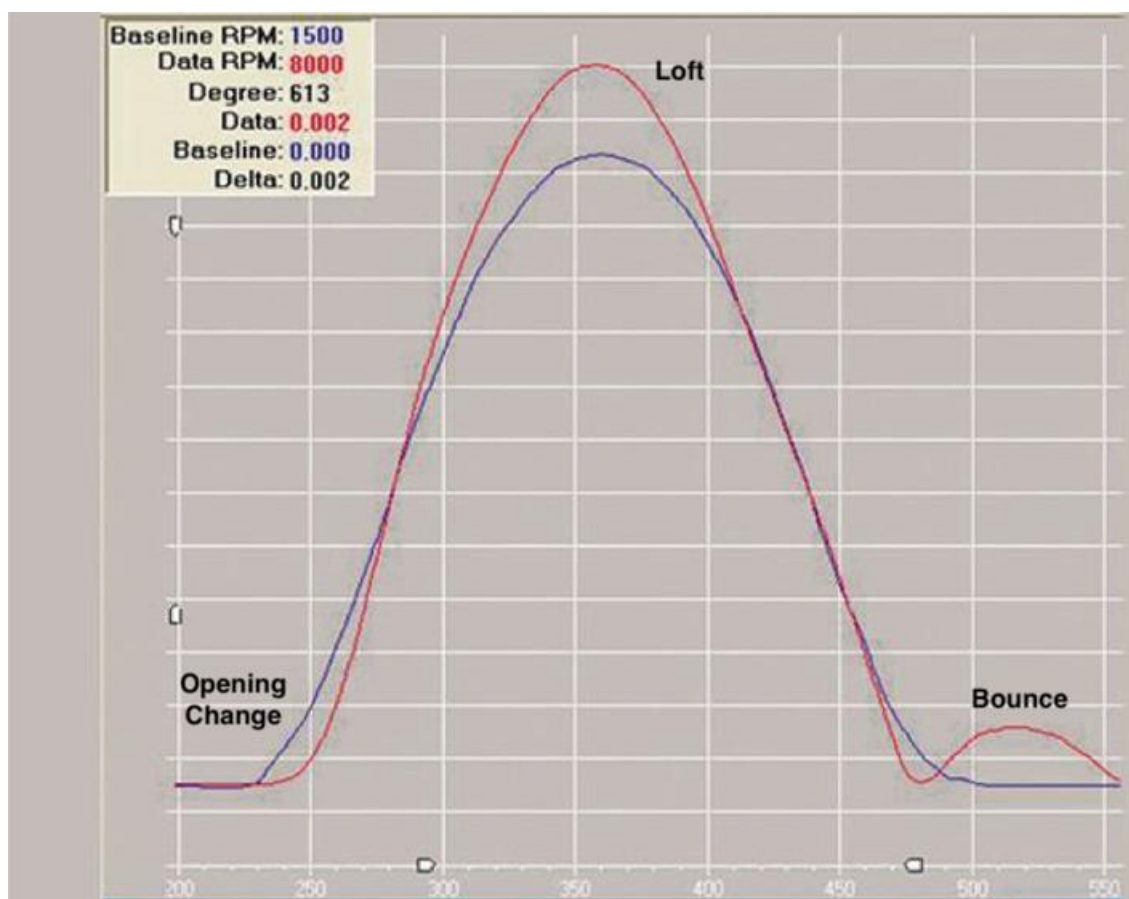
Figure 2.5 Depiction of valve loft and valve bounce in terms of valve displacement (Heeps, 2018).
