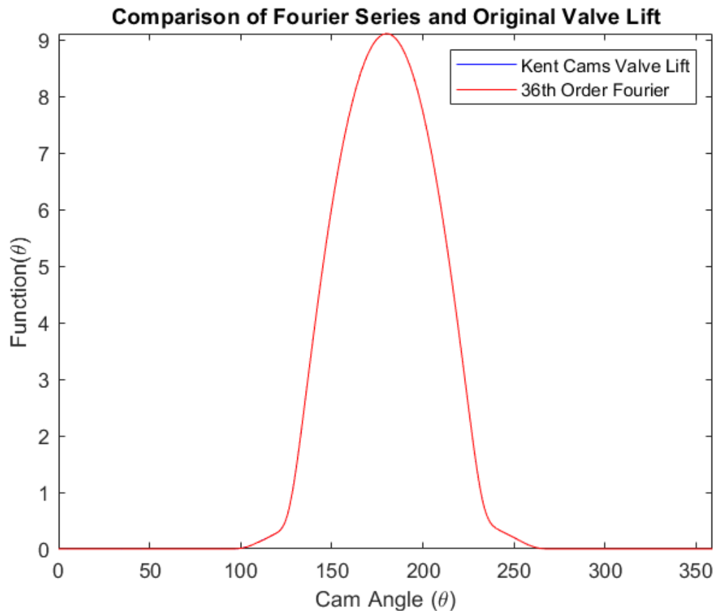
Figure 11.2 36th order Fourier series from Kent Cams valve lift data.
