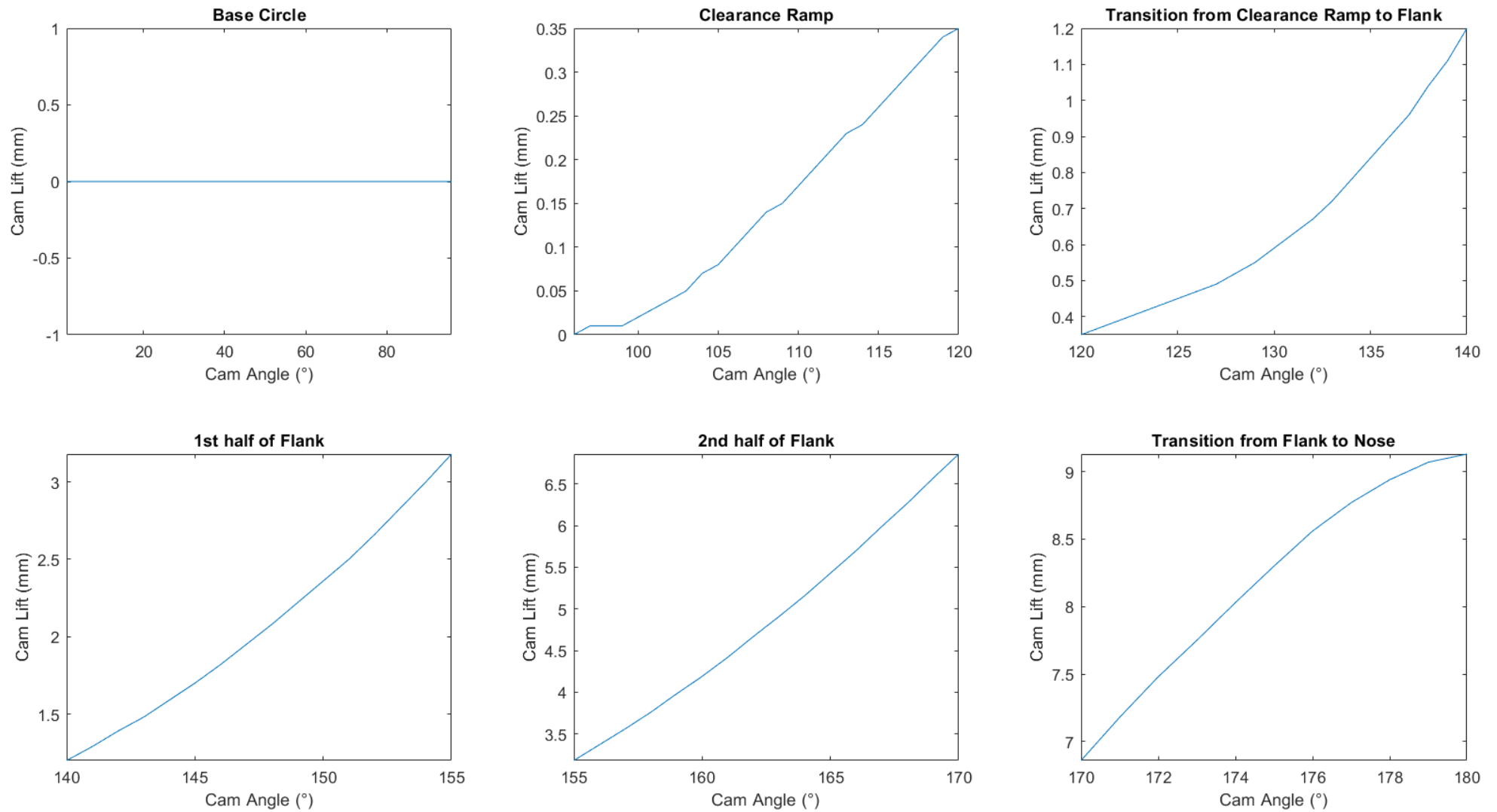
Figure 6.1 Cam lobe measurement error detection.
