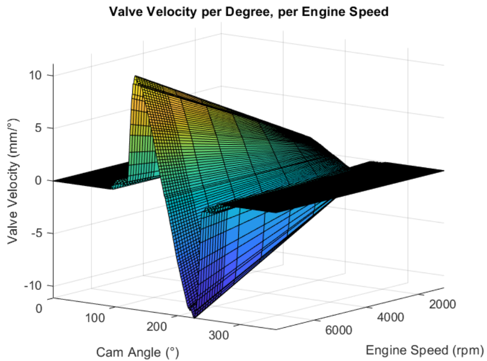
Figure 16.8 Valve velocity from raw measured data, per engine speed.
