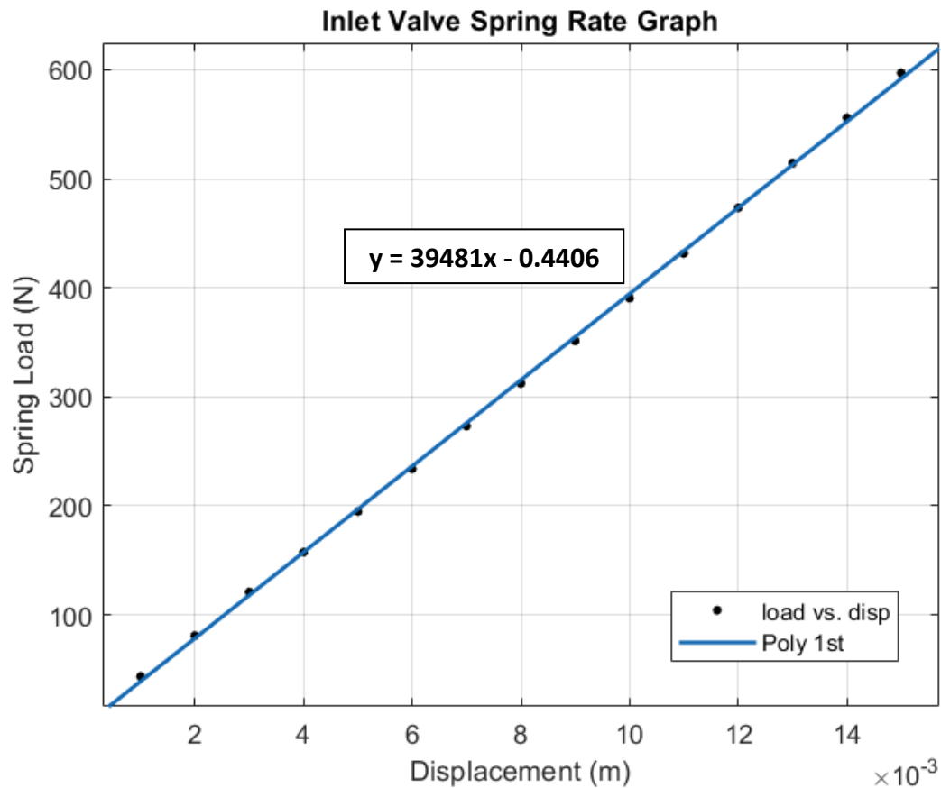
Figure 3.4 Force Displacement graph for the OEM Ford Duratec inlet valve spring.
