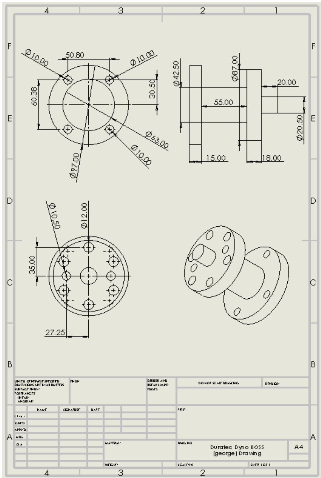
Figure 16.21 Dynamometer to Duratec adaptor boss, created in Solidworks from engine measurements.
