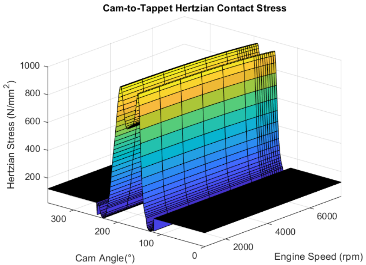
Figure 16.30 Hertzian stress.
