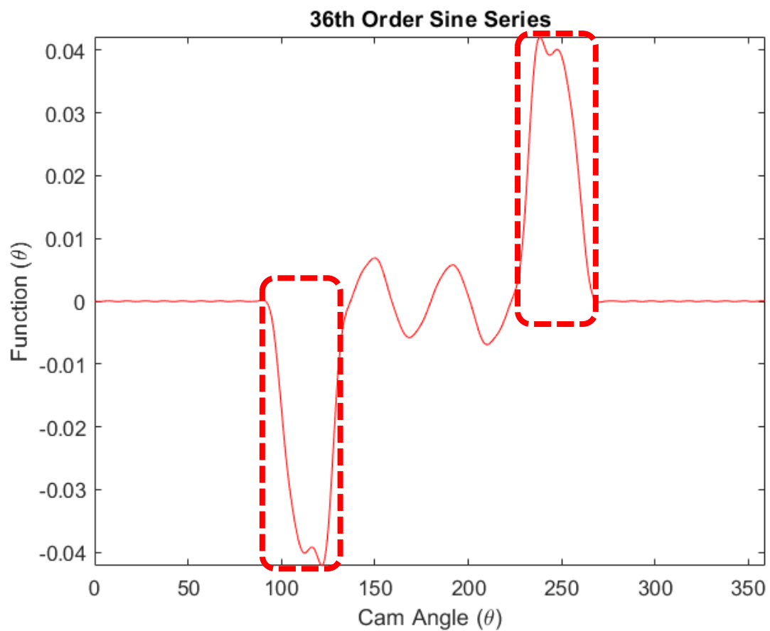
Figure 11.4 36th order Cosine series from Kent Cams valve lift data.
