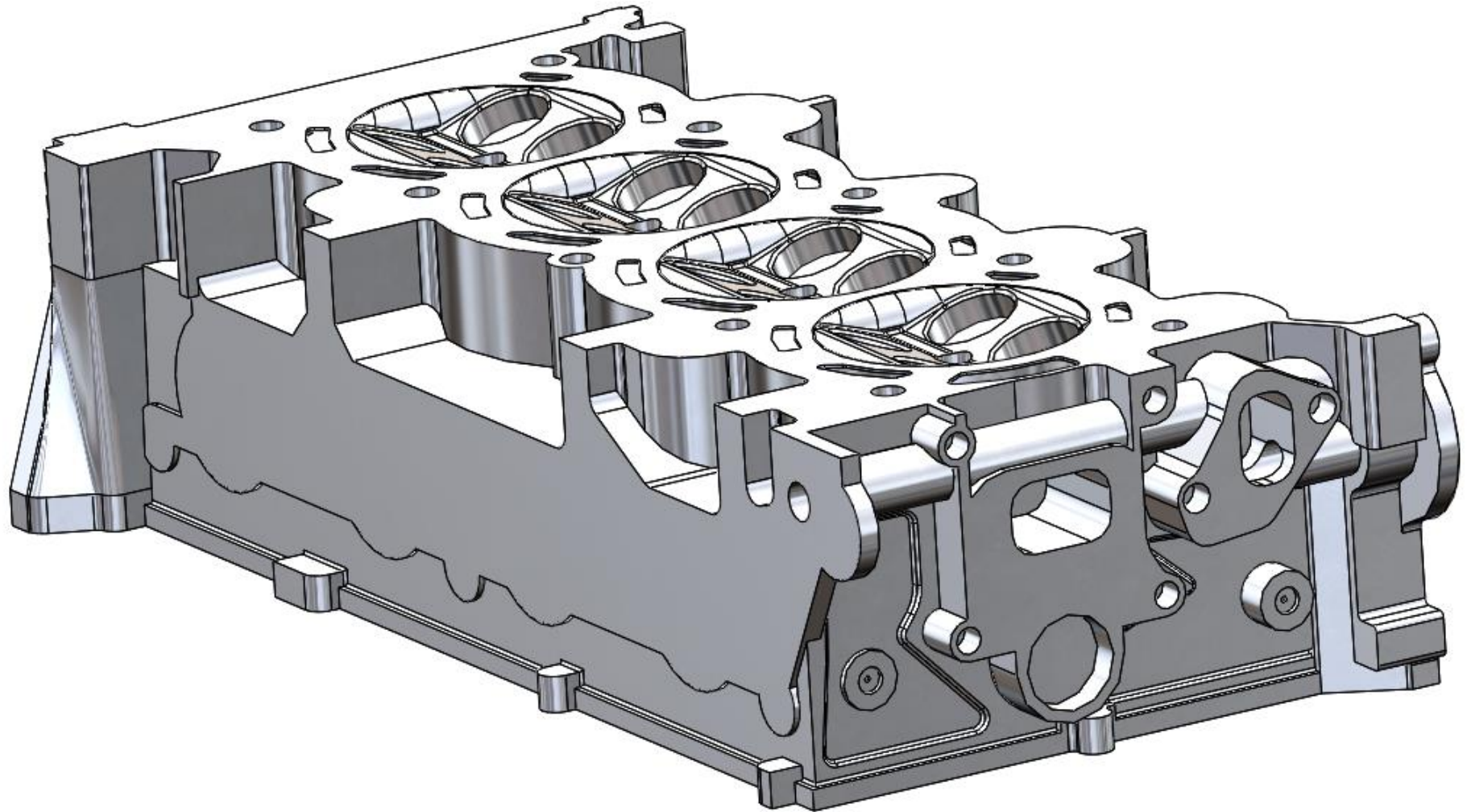
Figure 16.22 Duratec HE420 modelled Cylinder head intended for use in FEA
