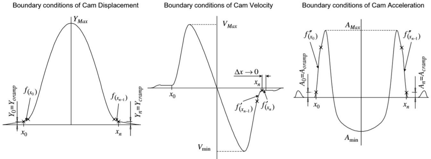
Figure 2.3 Camshaft profile design considerations through motion characteristics (Qiu, 2005).
