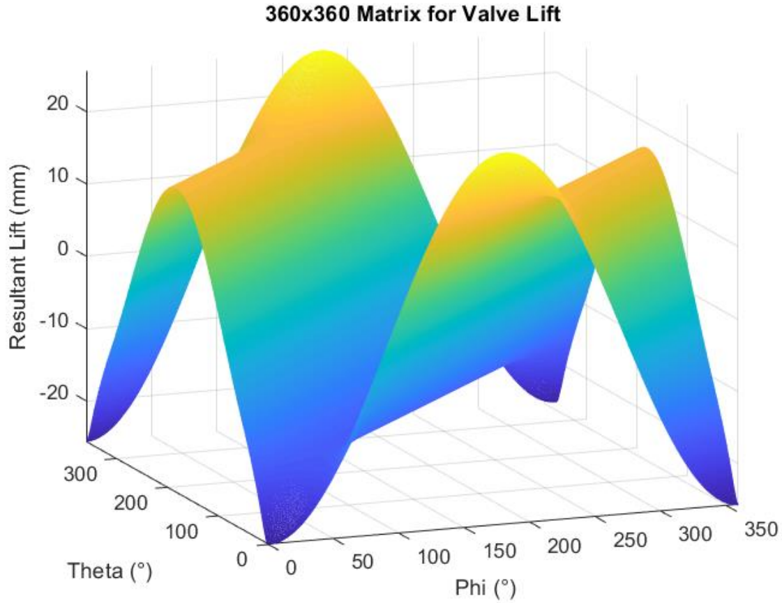
Figure 4.2 3D representation of 360 x 360 valve lift matrix.
