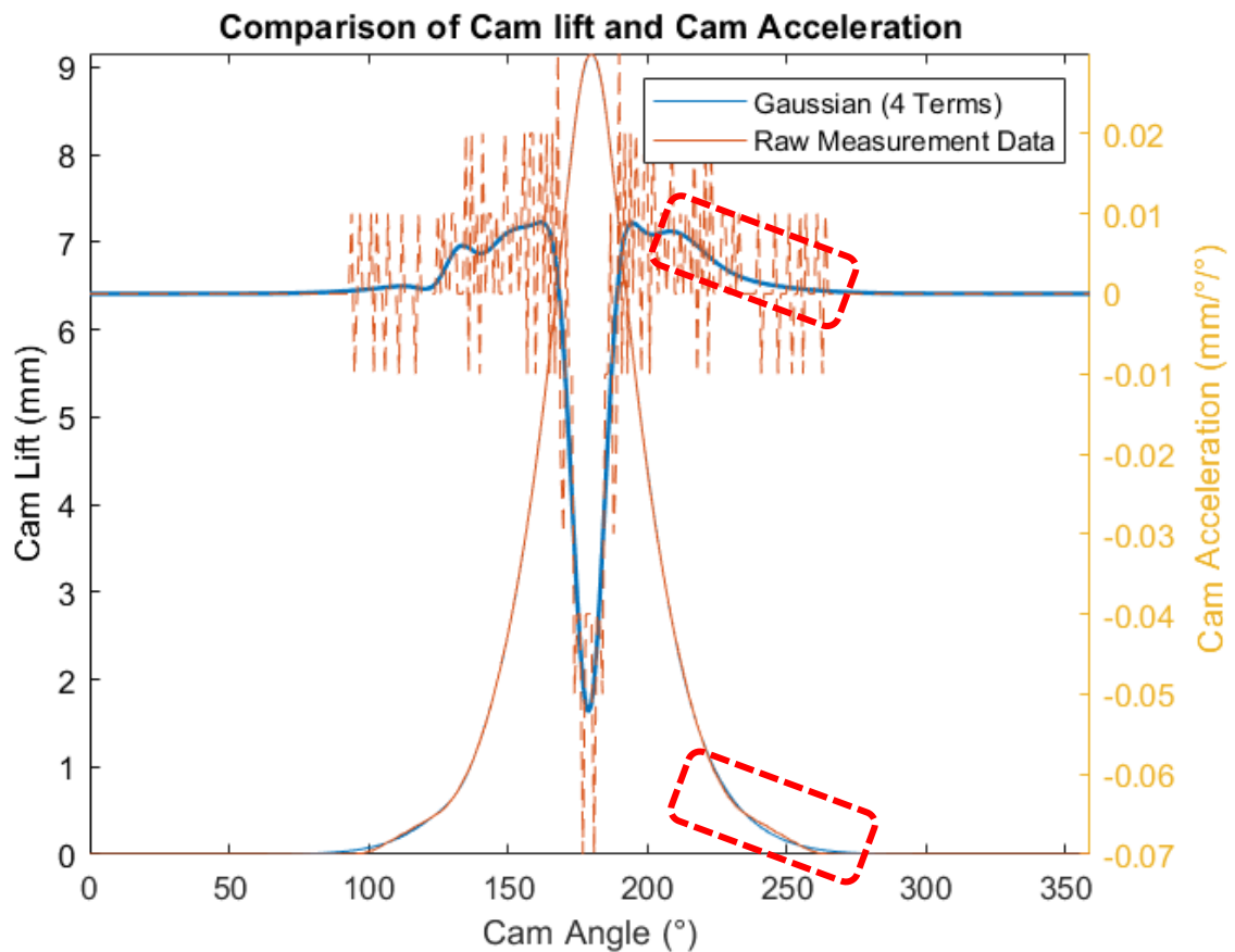
Figure 6.4 Comparison of 4 term Gaussian model to measured data, highlighting divergence.
