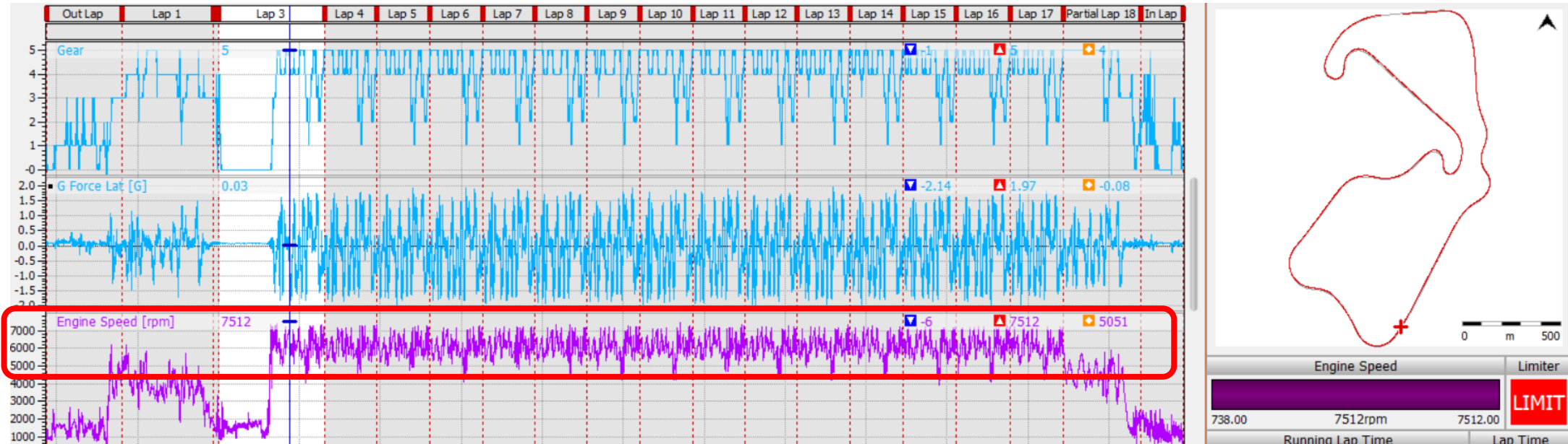
Figure 16.5 MoTeC data acquisition for the UWTSD MCR Race Car at Silverstone GP circuit, shows peak engine speed at 7,512rpm with aggressive downshift into Stowe corner. Also shows average lap engine speed between 5000rpm and 7500rpm.
