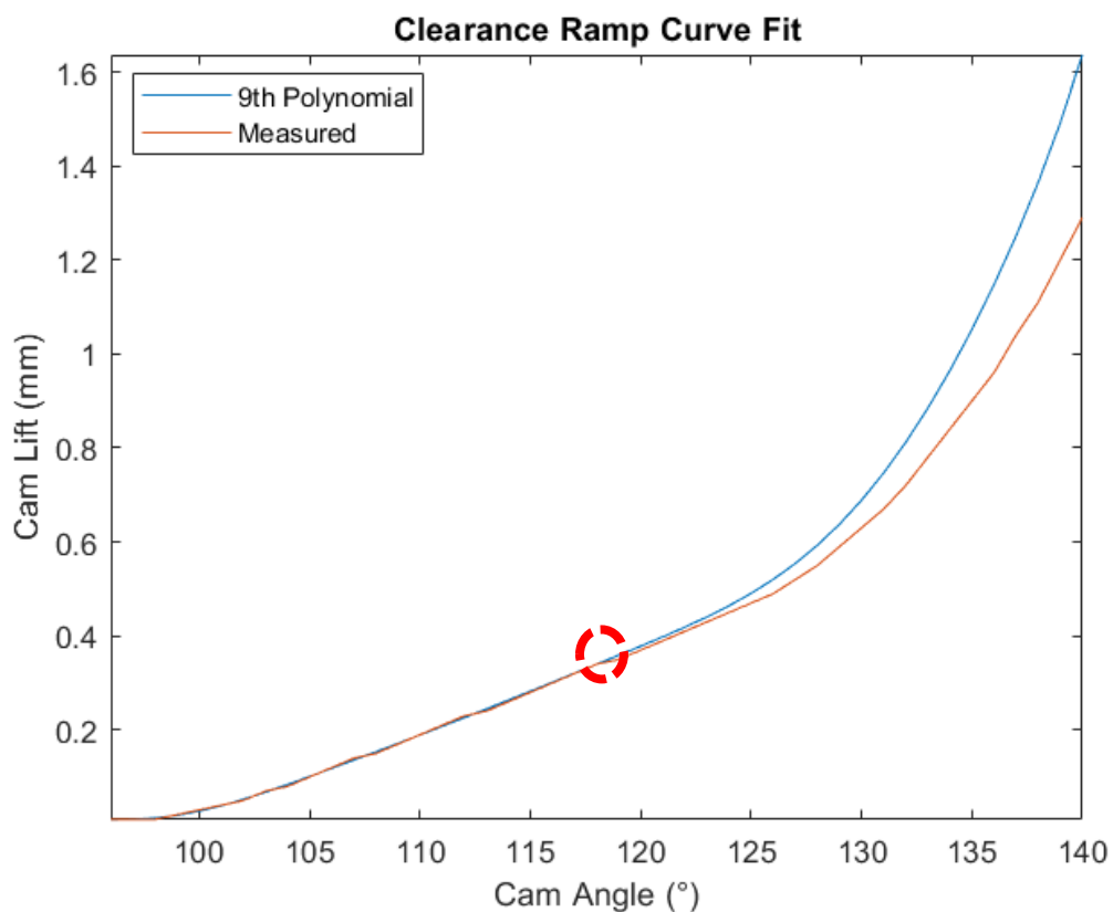
Figure 6.5 Clearance ramp of the cam profile. The 9th degree polynomial can be seen to converge until approximately 118°.
