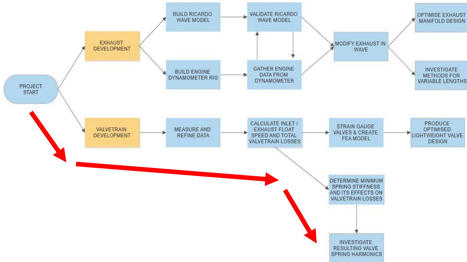
Figure 1.2 The initial project concept to explore the Duratec engine, with final outcome..
