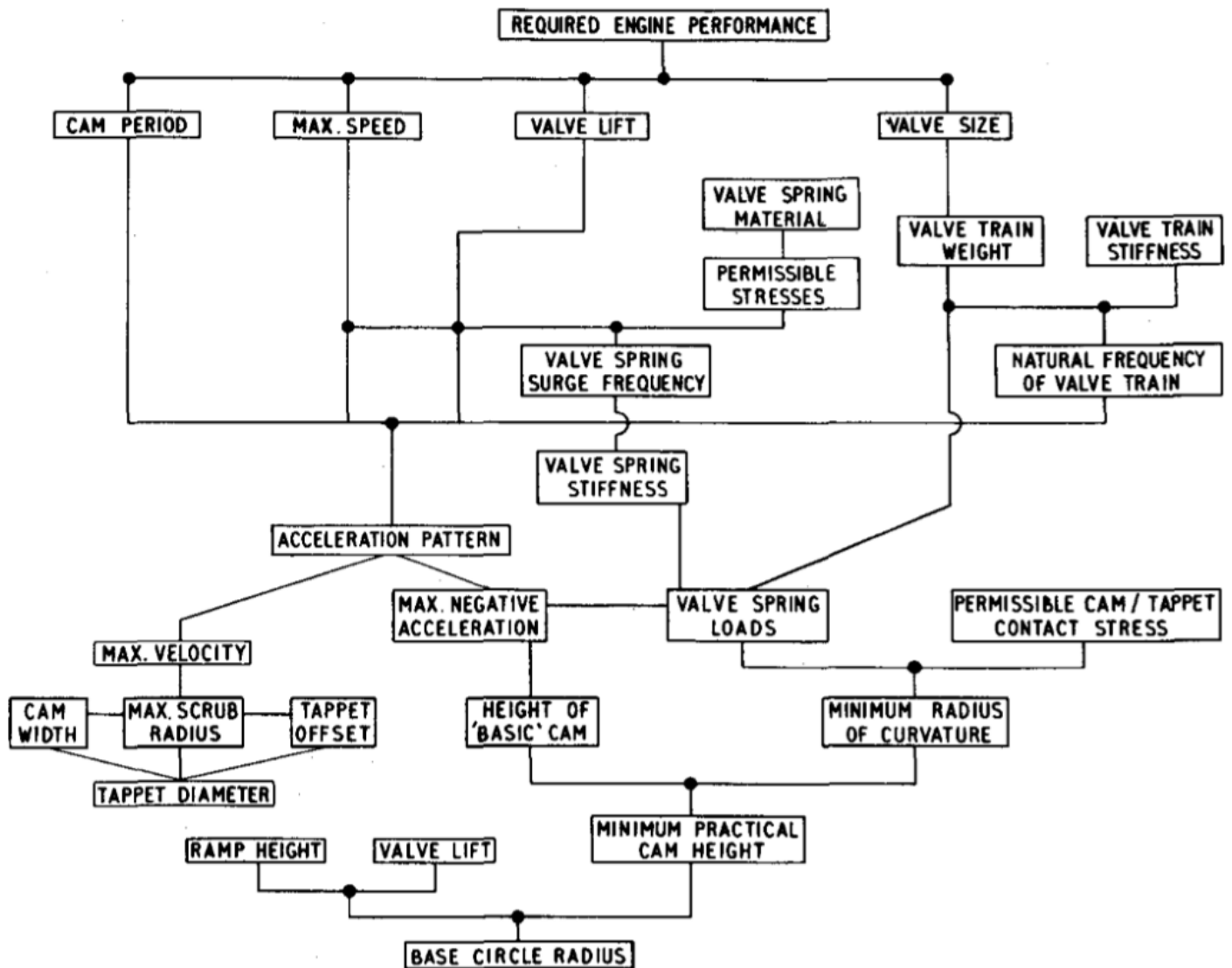
Figure 2.2 Factors to be considered in valve gear design (Beard and Hempson, 1962).
