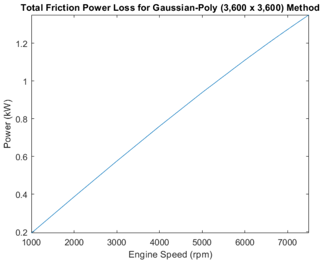
Figure 7.4 Total friction power loss through the engine speed range.
