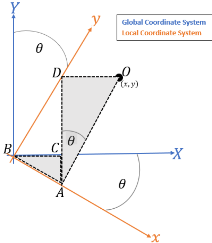
Figure 9.3 Diagram for finding global coordinate X .
