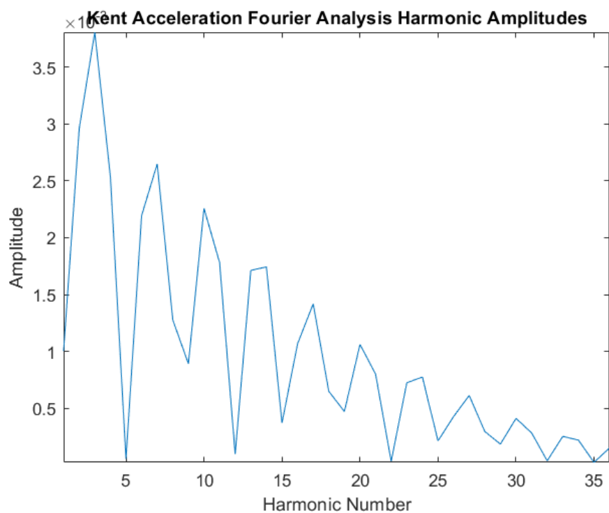
Figure 16.18 36 th order of Fourier acceleration harmonic amplitudes.
