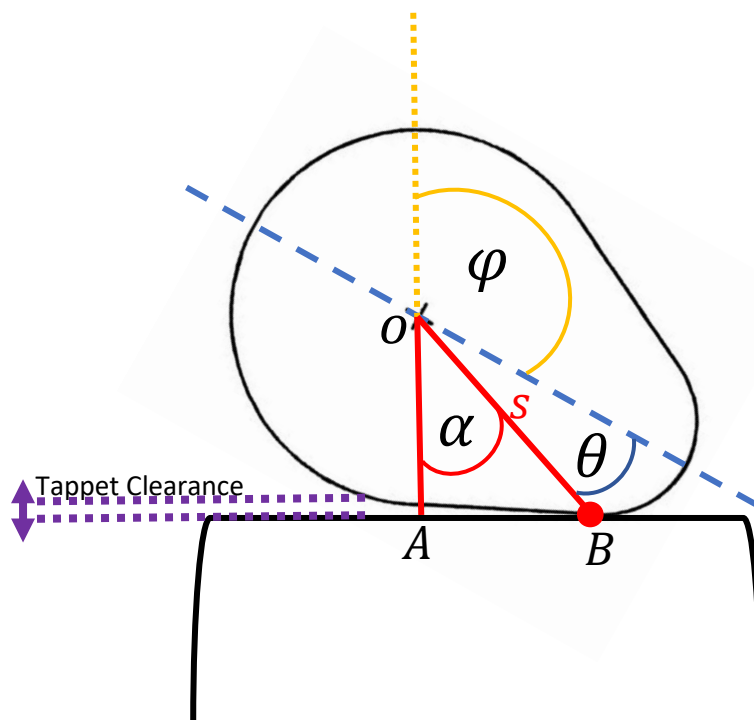
Figure 4.1 Diagram of cam-to-tappet interface with reference to contact point and valve lift.
