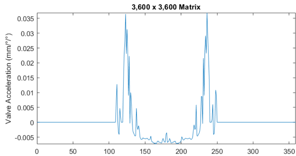
Figure 5.3 Valve lift matrix study for measured cam profile – acceleration plots.
