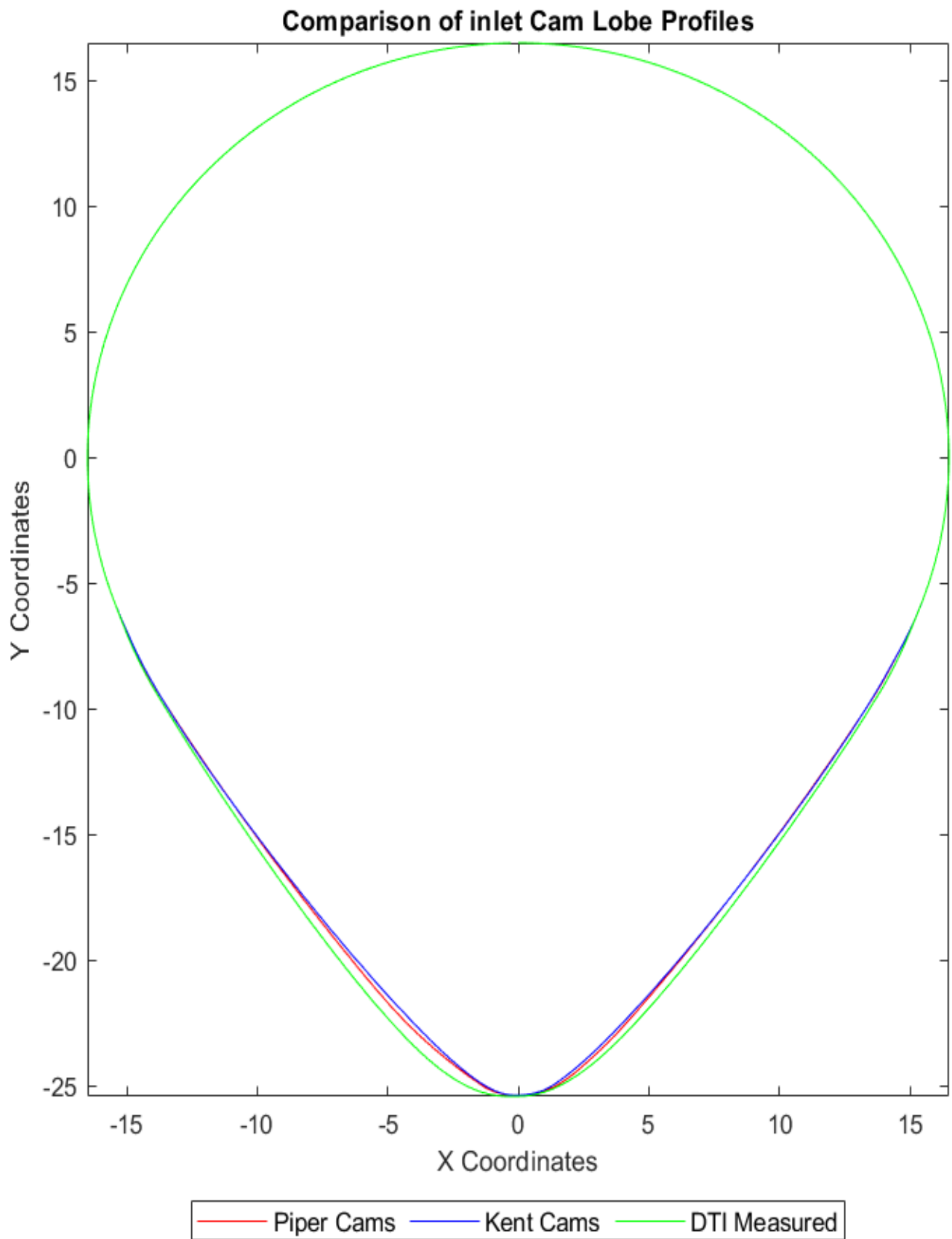
Figure 12.3 Inlet cam lobe profiles generated from rotation of axes conversion method.
