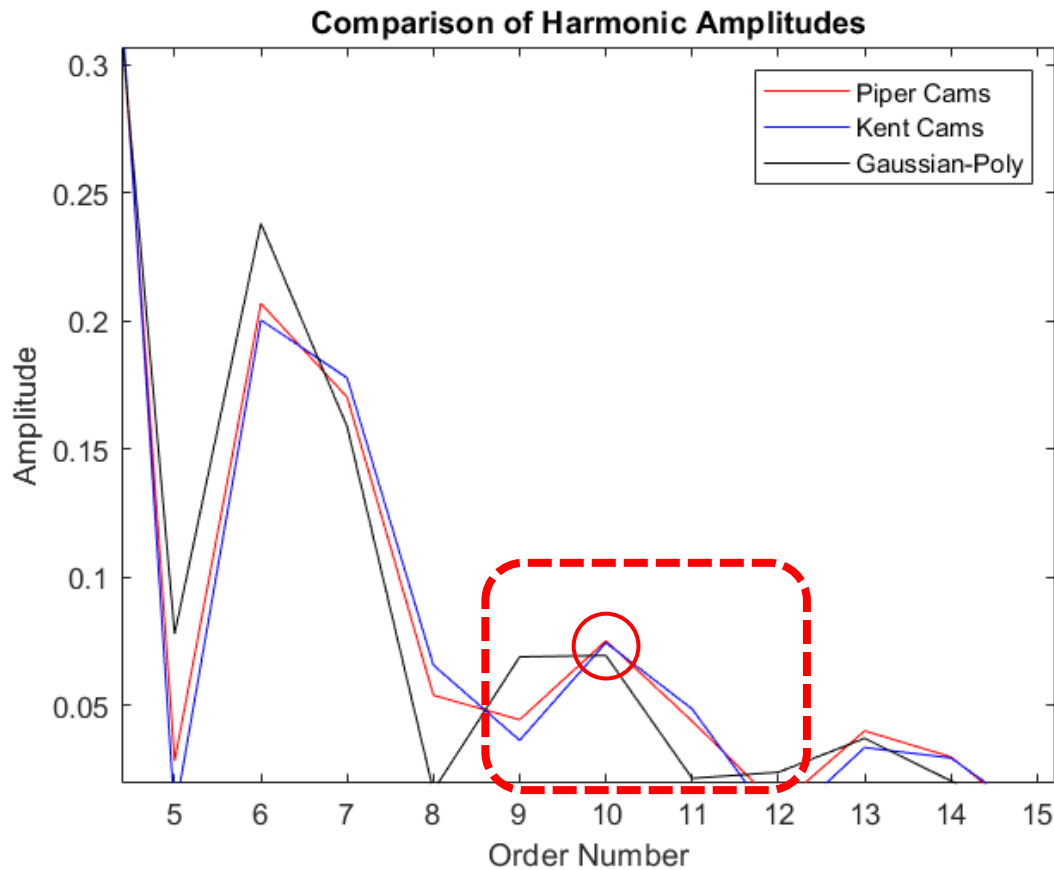
Figure 11.6 Comparison of harmonic amplitudes from all methods, highlighted engine speed range.
