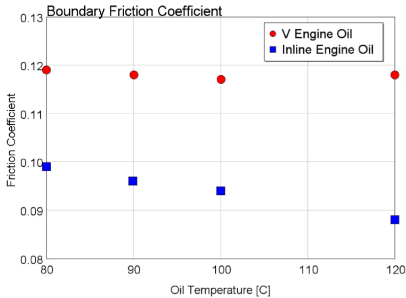
Figure 2.9 Cam-to-tappet boundary friction coefficient for “V” and “Inline” configurations, using two different variants of SAE 5W-20 oil (Okarmus and Keribar, 2015).
