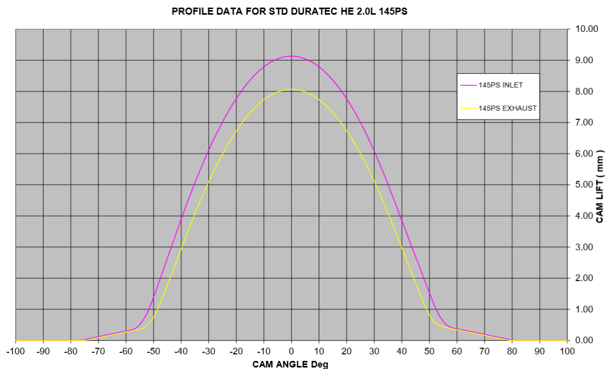
Figure 8.1 Kent Cams interpretation of original Ford Duratec inlet and exhaust valve profiles.
