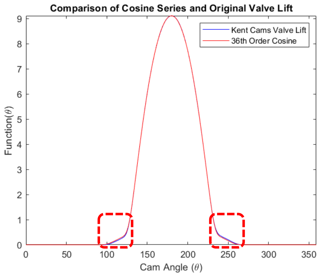
Figure 11.3 36th order Cosine series from Kent Cams valve lift data.
