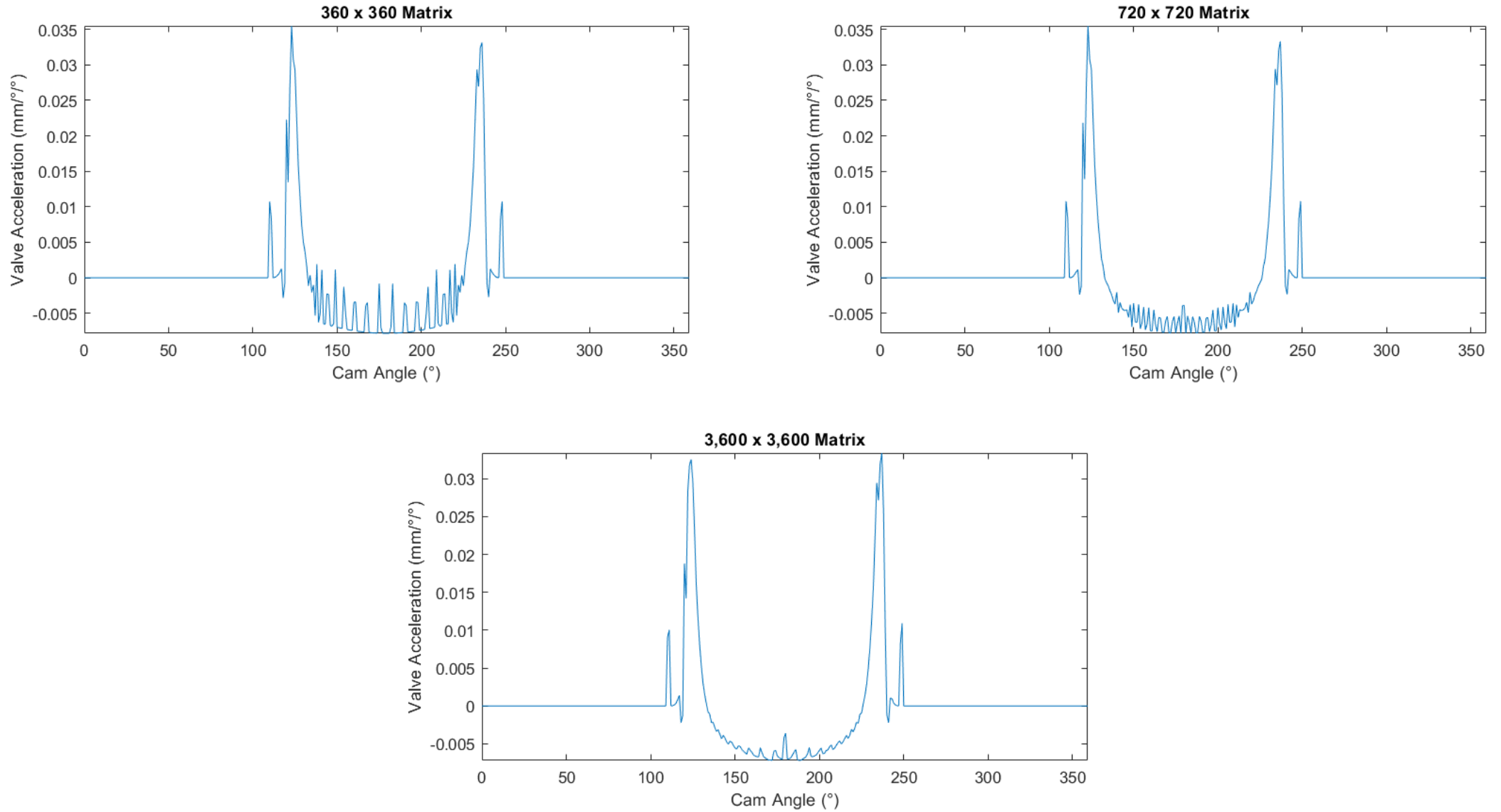
Figure 6.9 Valve lift matrix study for the hybrid curve fit model (Gaussian-Polynomial) – acceleration plots.
