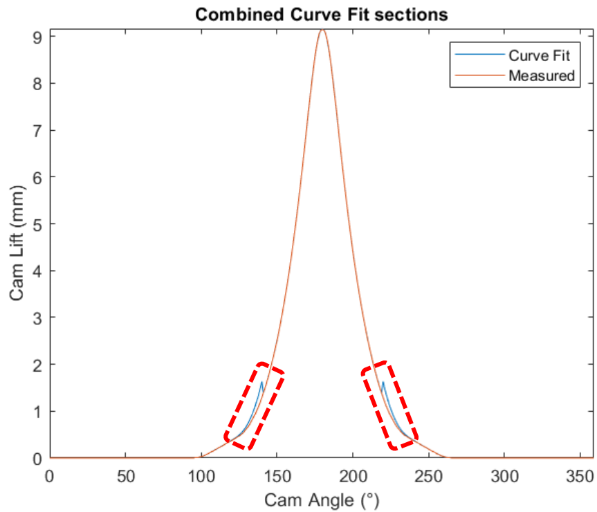
Figure 6.7 Combined curve fits before interpolation “data patch” was applied to the highlighted sections.
