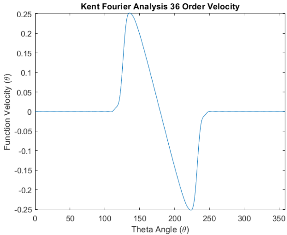
figure 16.13 differential of Fourier series for valve lift.
