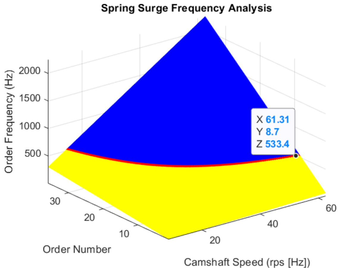
Figure 11.7 Spring surge frequency analysis.
