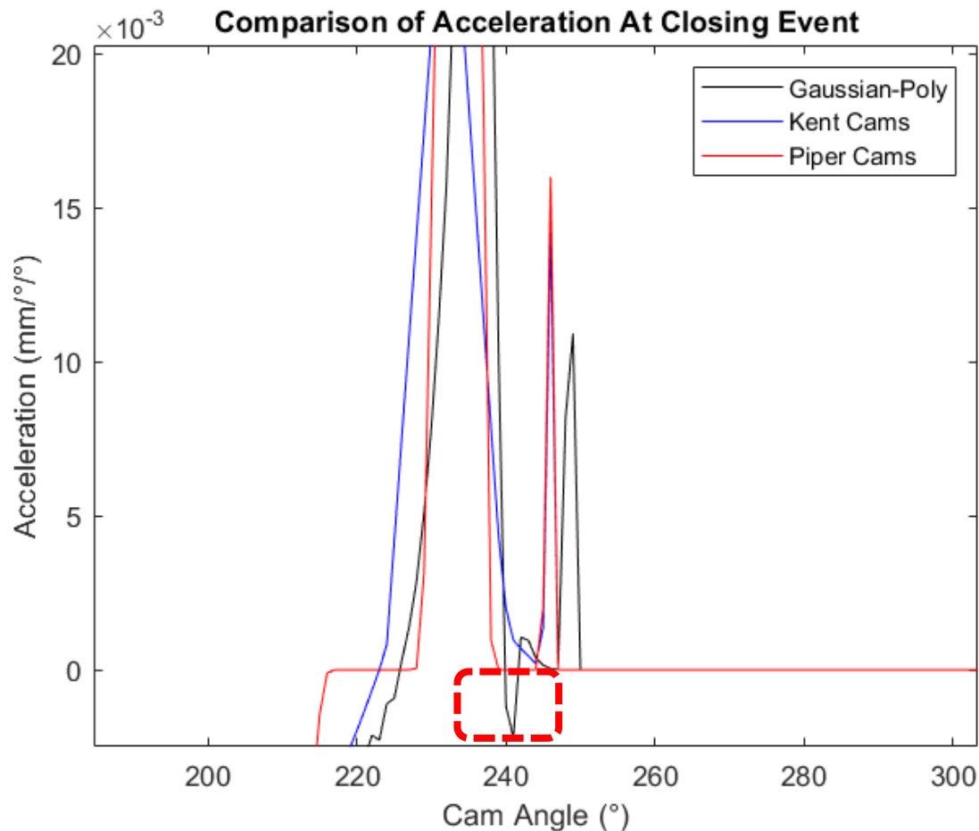
Figure 12.4 Comparison of acceleration profiles magnified to valve closing point.
