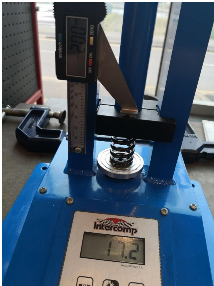
Figure 3.3 Measuring force and displacement properties - Ford Duratec inlet valve spring (Intercomp Spring tester).
