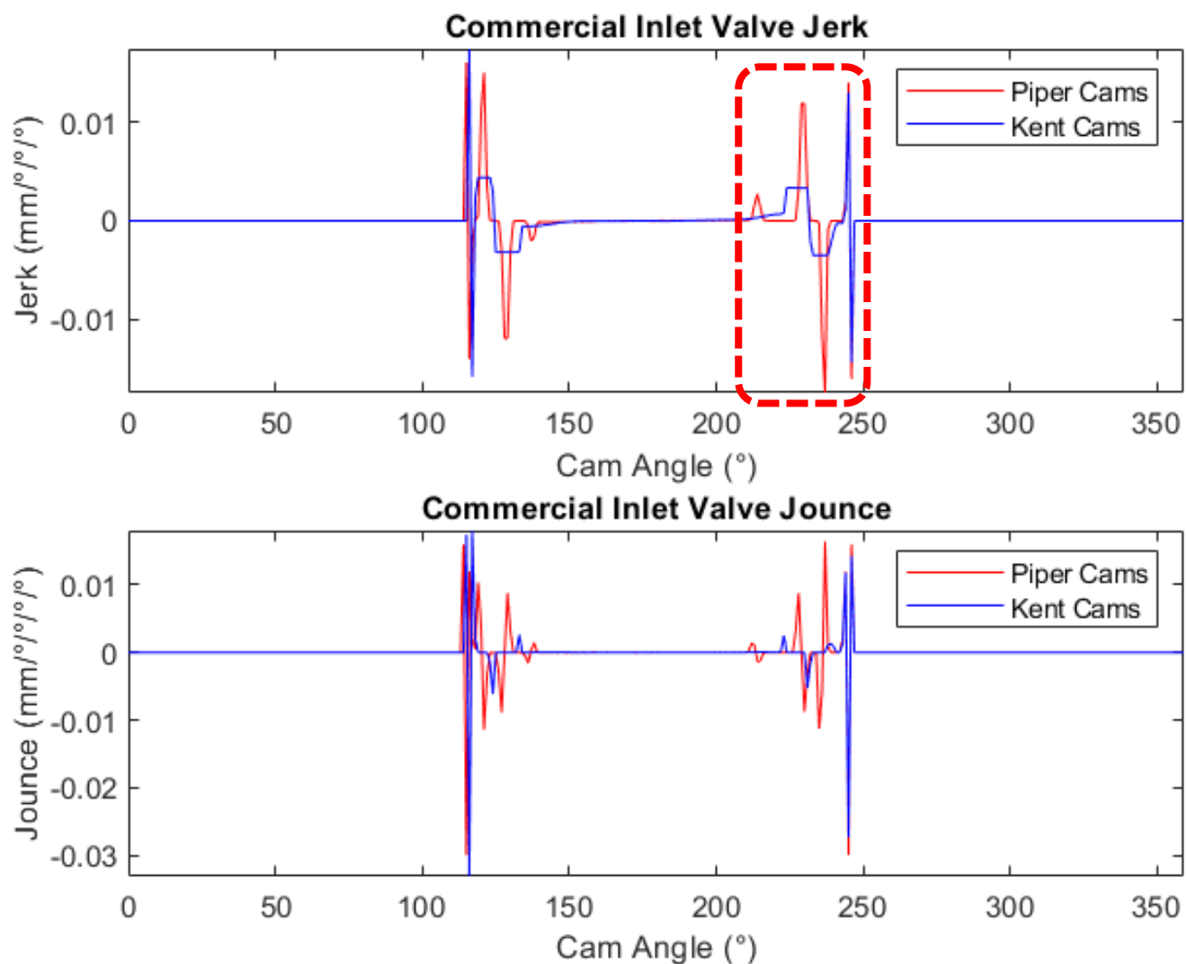
Figure 10.3 Comparison between Kent Cams and Piper Cams inlet valve jerk and jounce.
