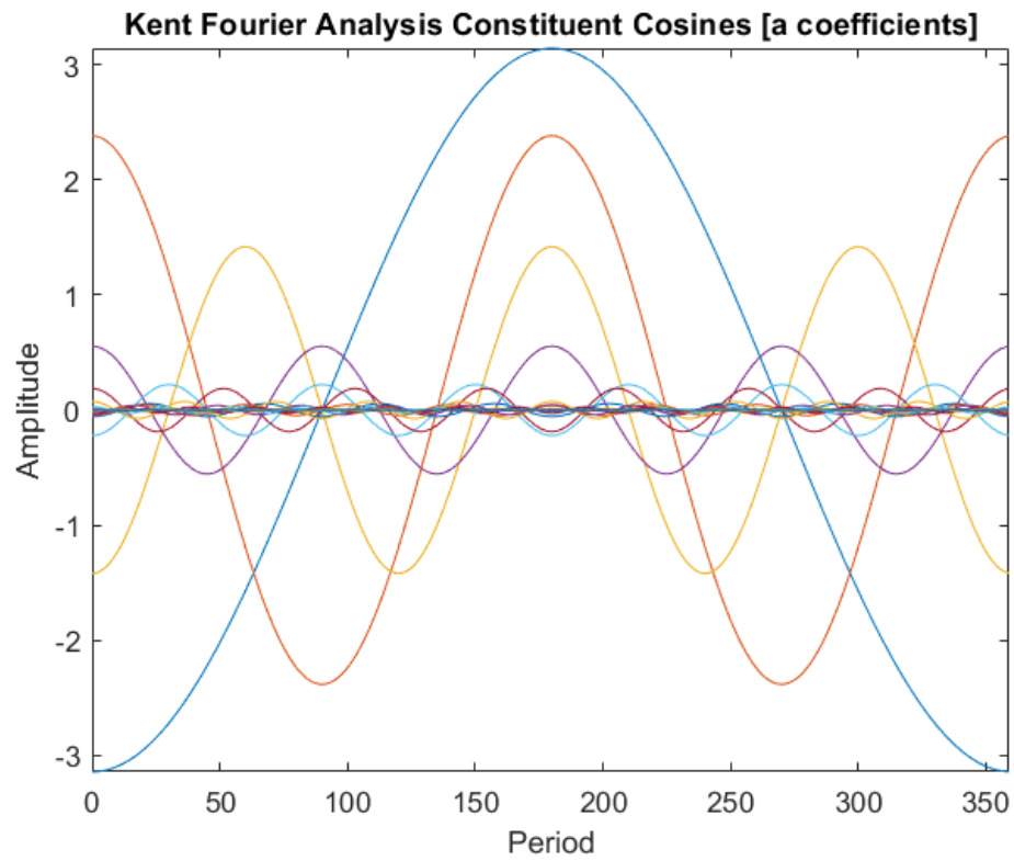
figure 16.15 Constituent cosine waves of the Fourier series.
