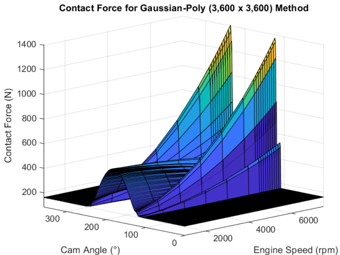
Figure 7.1 Contact force per cam angle, per engine speed for the Gaussian-Polynomial method.
