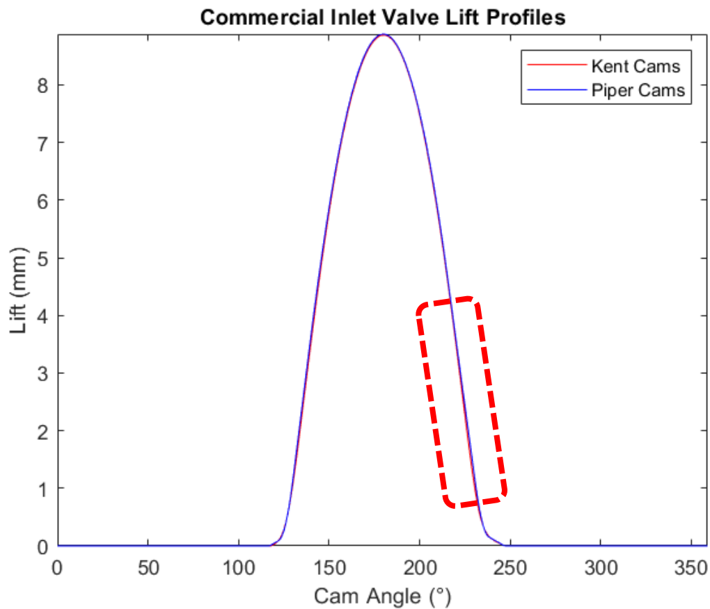
Figure 10.1 Comparison between Kent Cams and Piper Cams inlet valve lift.
