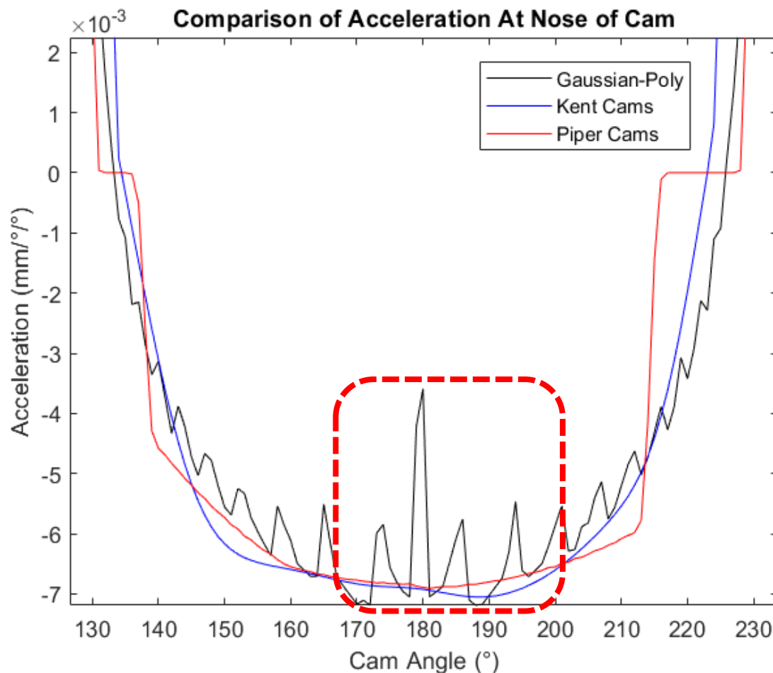
Figure 12.2 Comparison of valve accelerations for each profile, magnified at the nose of the cam.
