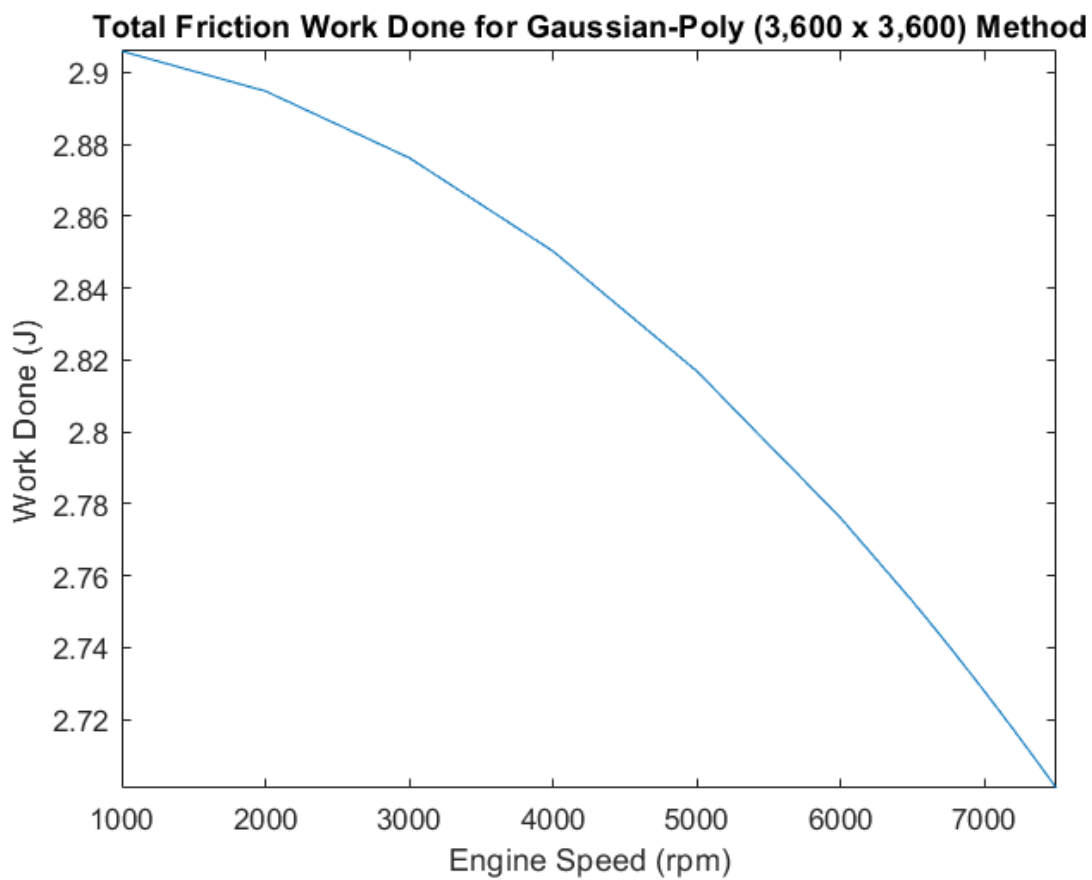
Figure 7.3 Total friction work done through the engine speed range.
