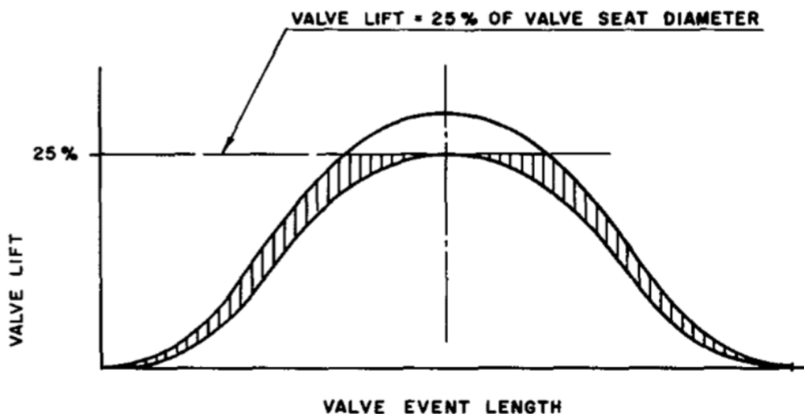
Figure 2.4 A graph to show the gain in effective valve lift area with optimised lift (Nourse, Dennis and Wood, 1961).
