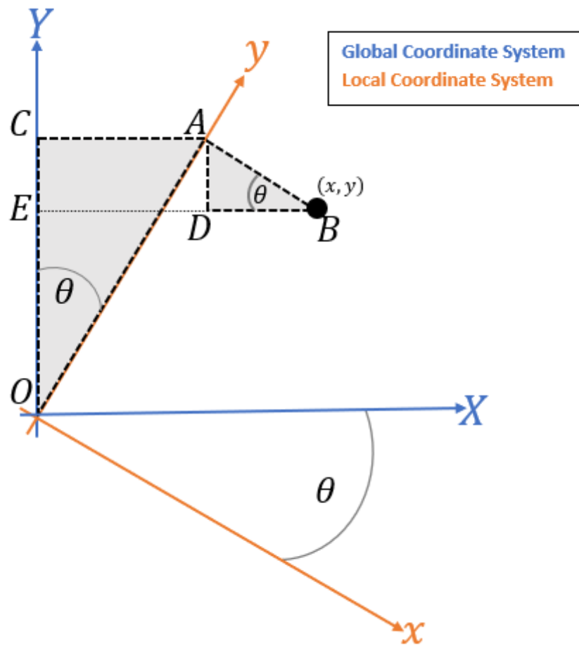
Figure 9.4 Diagram for finding global coordinate Y .
