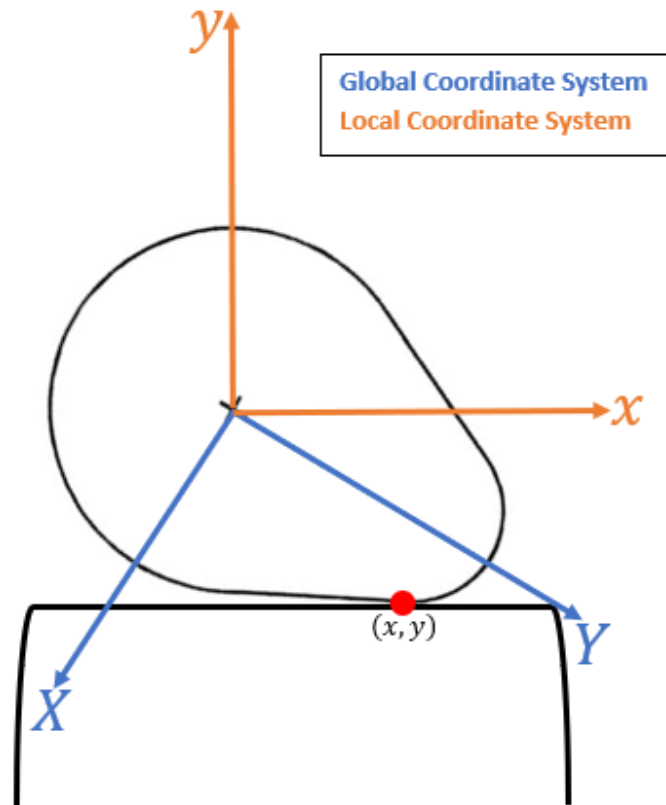
Figure 9.2 Relative coordinate system for rotation of axis. Applied to cam lobe and tappet (valve lift).
