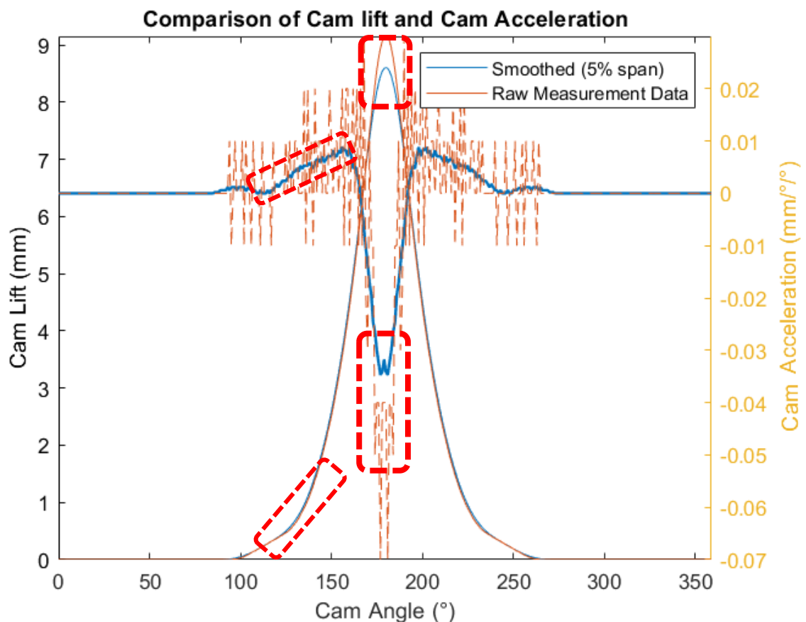
Figure 6.2 Comparison of 5% Smoothed model to measured data, highlighting inaccuracies.
