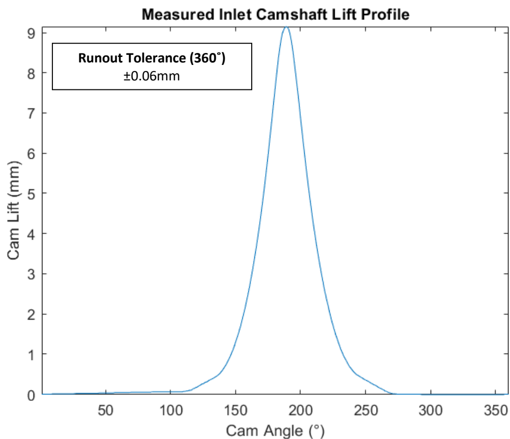
Figure 3.2 Cam lift profile from raw measurement data, using the optical dividing head and DTI.
