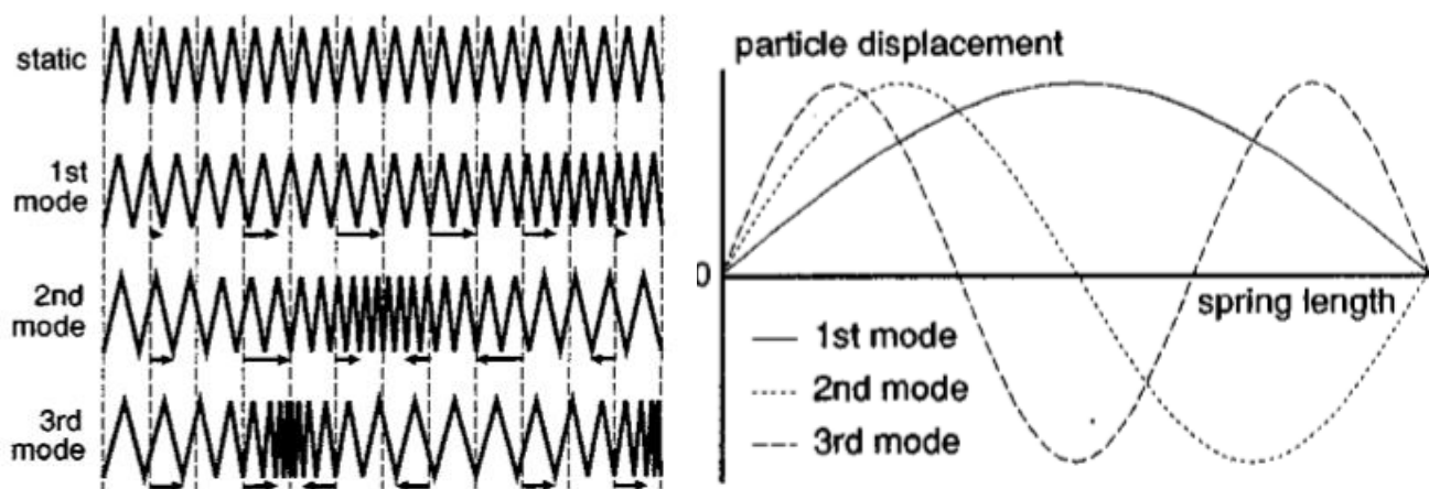
Figure 2.7 Sketch of the first three mode shapes in the valve spring with corresponding particle displacement against spring length (Schamel et al. , 1993).
