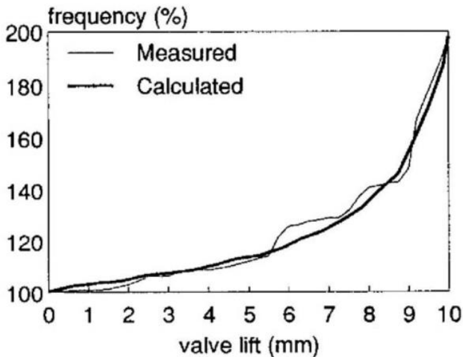
Figure 2.8 Comparison of measured and calculated spring frequency characteristics (Schamel et al., 1993).
