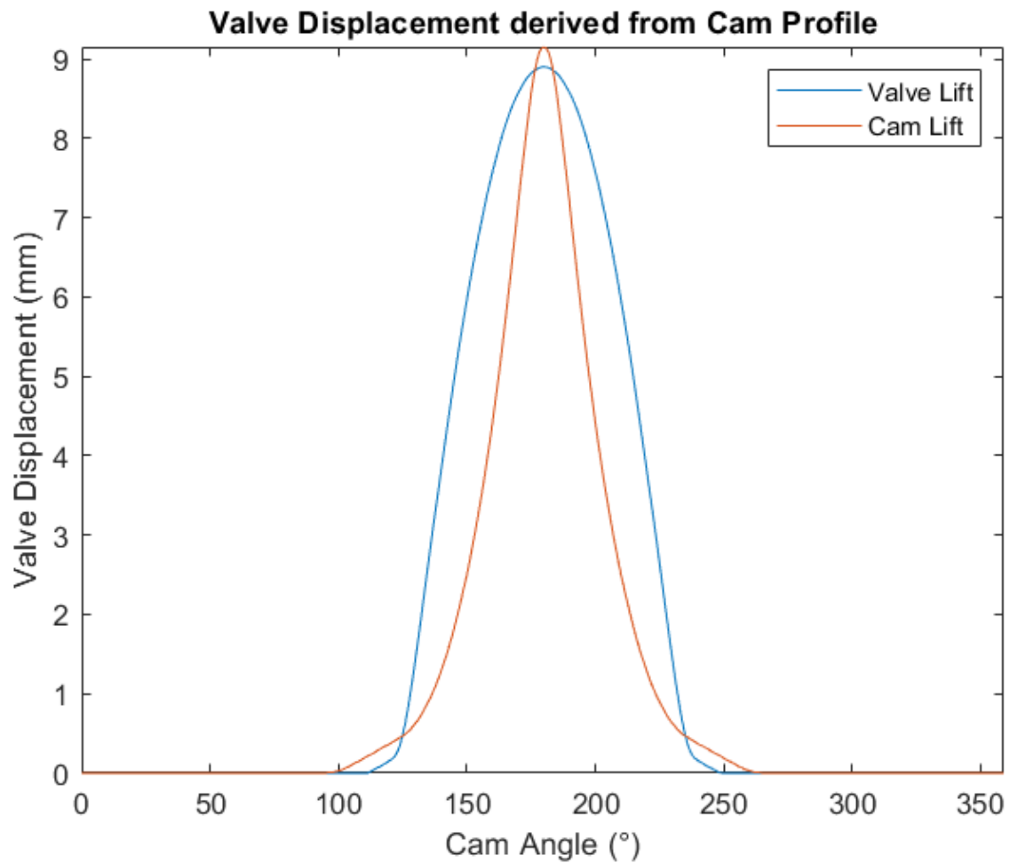
Figure 4.3 Resultant valve lift from matrix, derived from measured cam profile.
