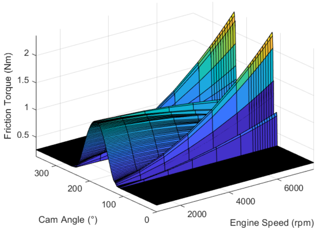
Figure 7.2 Friction torque per cam angle, per engine speed for the Gaussian-Polynomial method.
