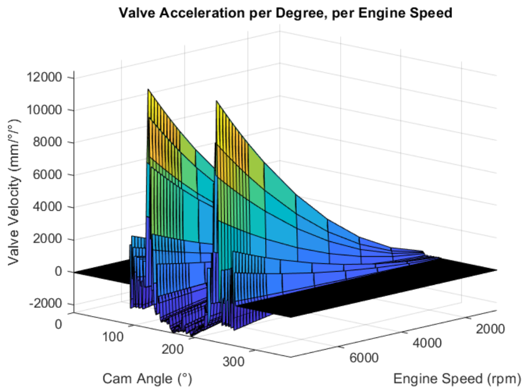
Figure 16.9 Valve acceleration from raw measured data, per engine speed.
