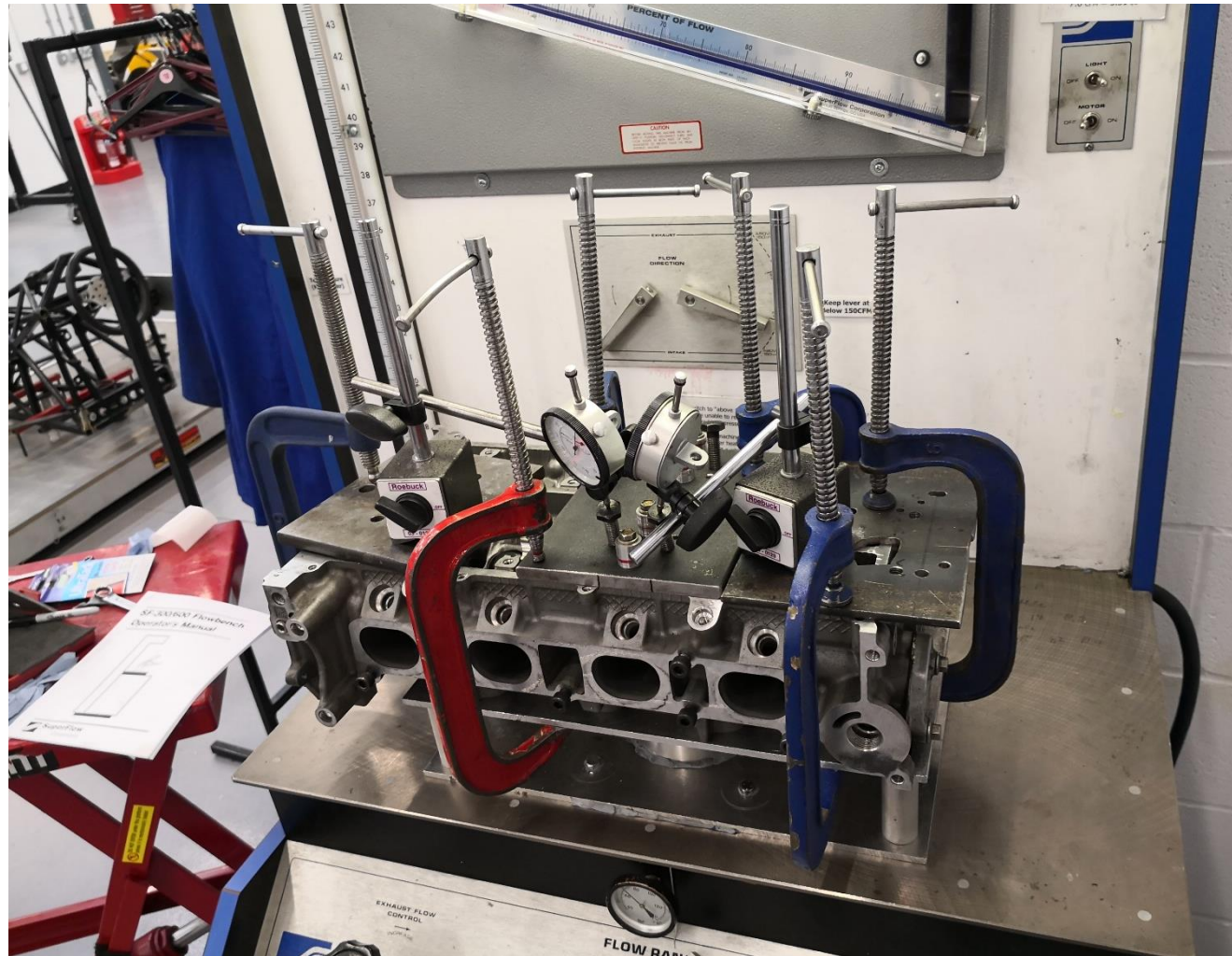
Figure 16.26 Cylinder head flow bench test setup.
