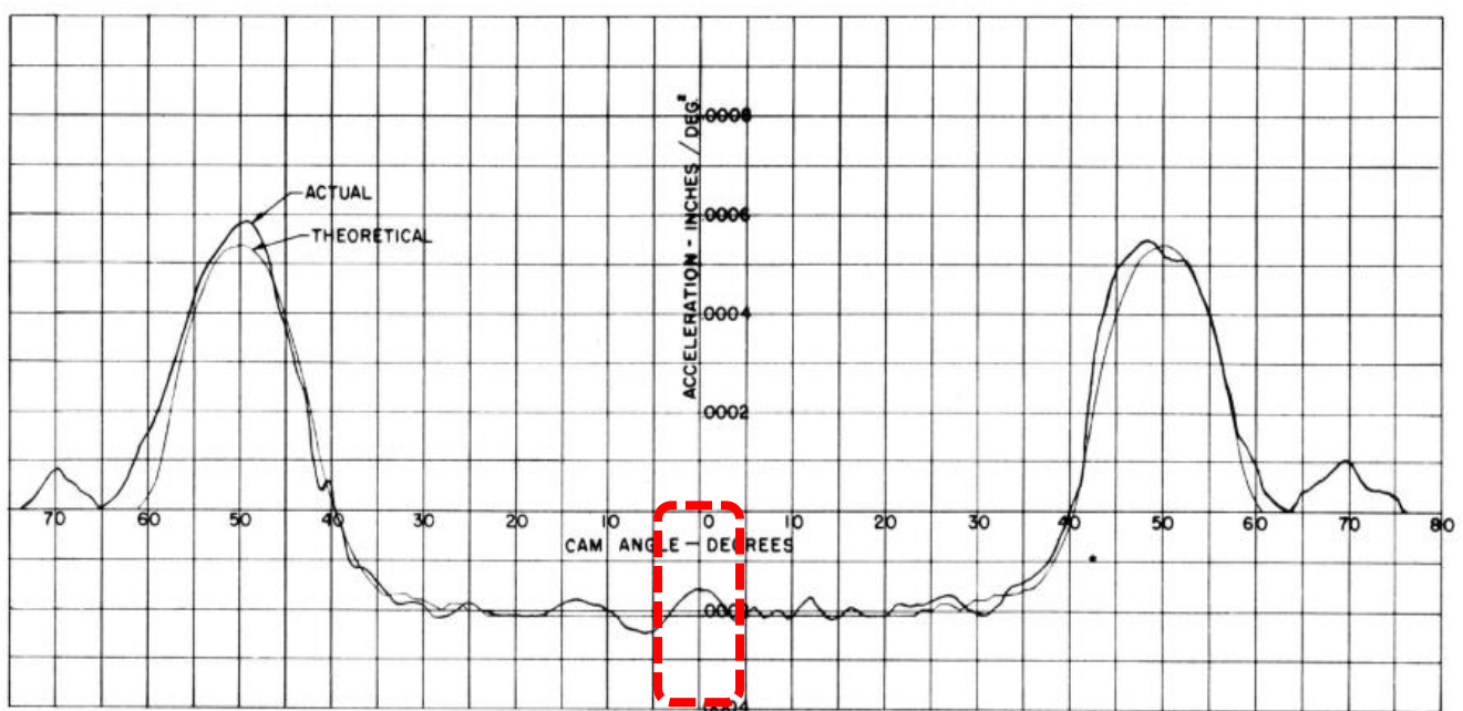
Figure 12.1 Example of valve acceleration, derived from measuring cam in lathe (Turkish, 1950).
