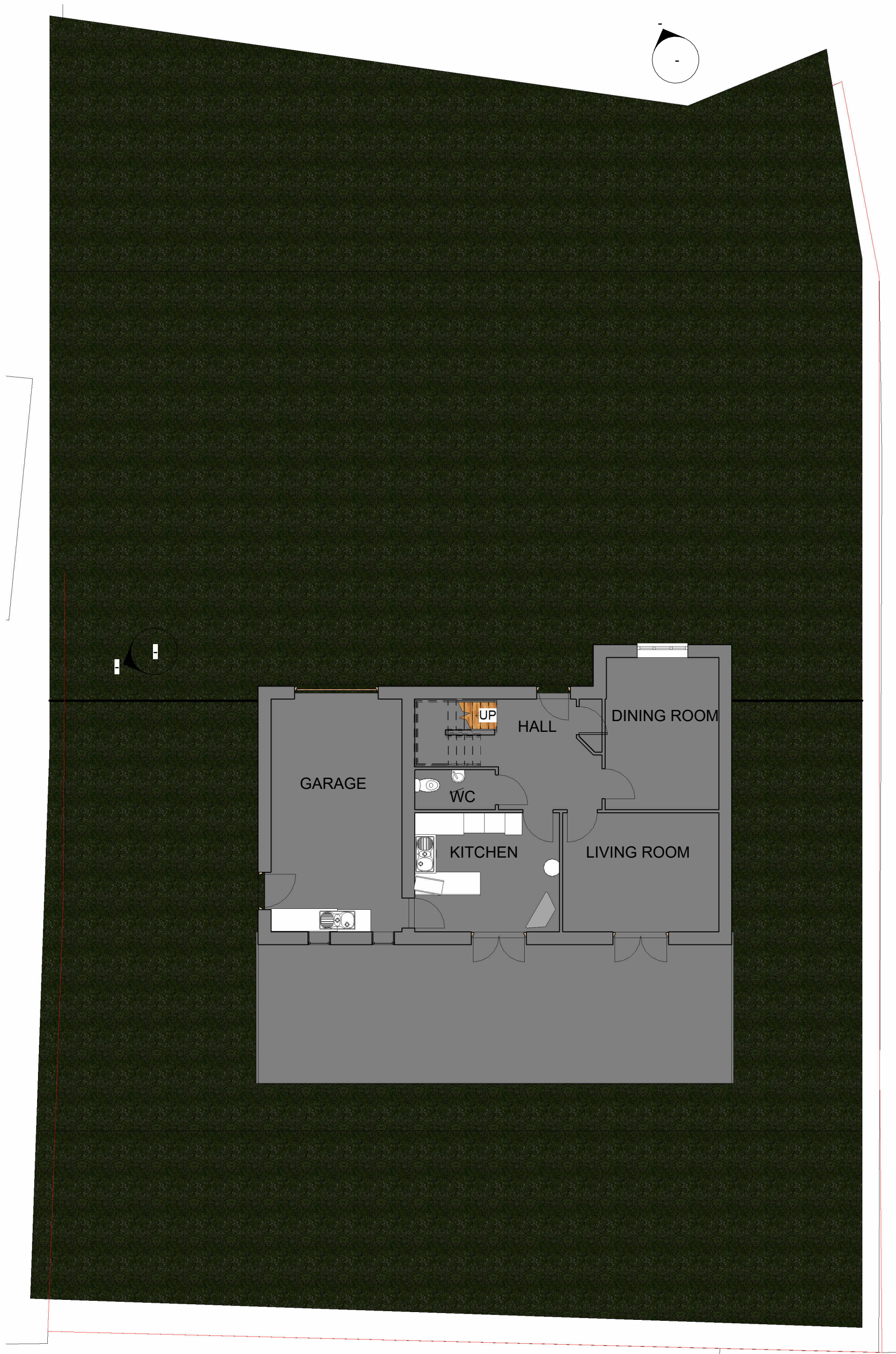
1 0 - Ground Floor Plan 1 : 100
