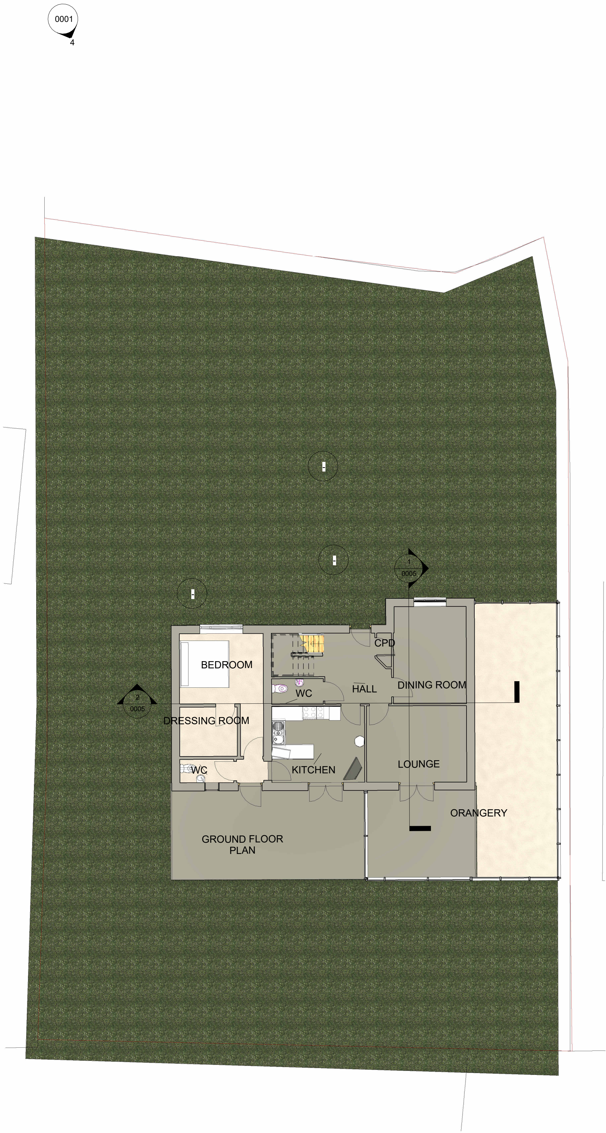
1 0 - Ground Floor Plan 1 : 100
