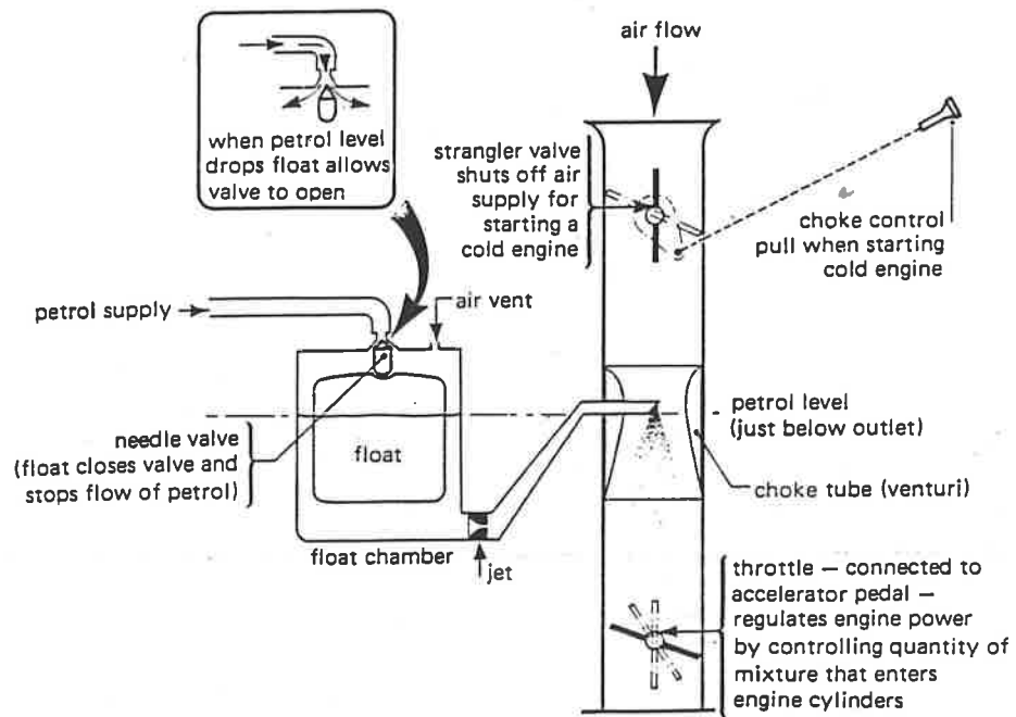
Layout of simple carburettor
