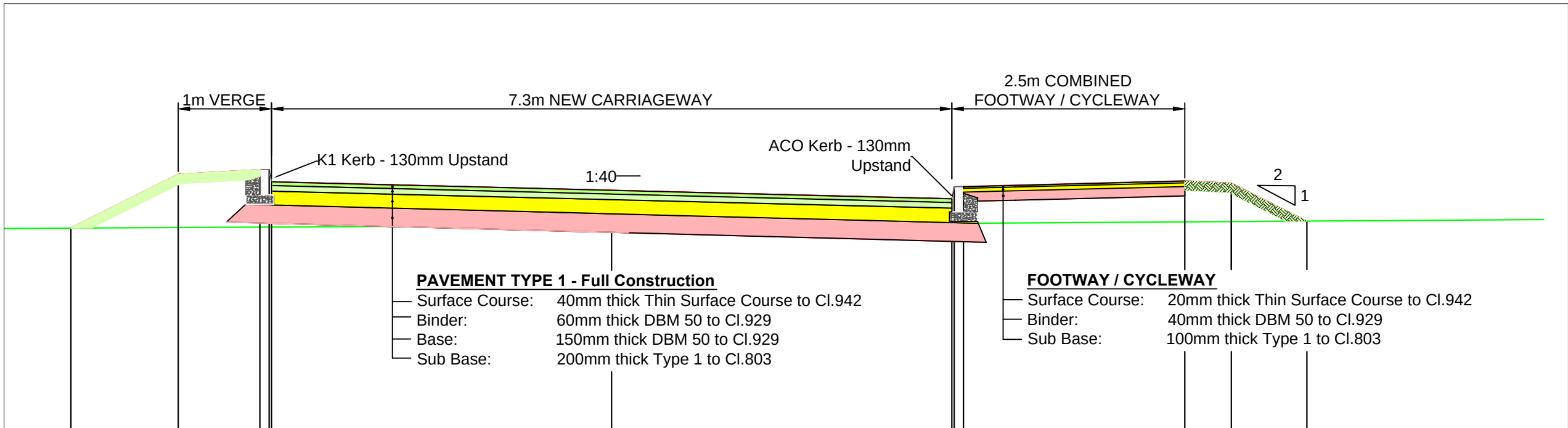
SECTION B-B
