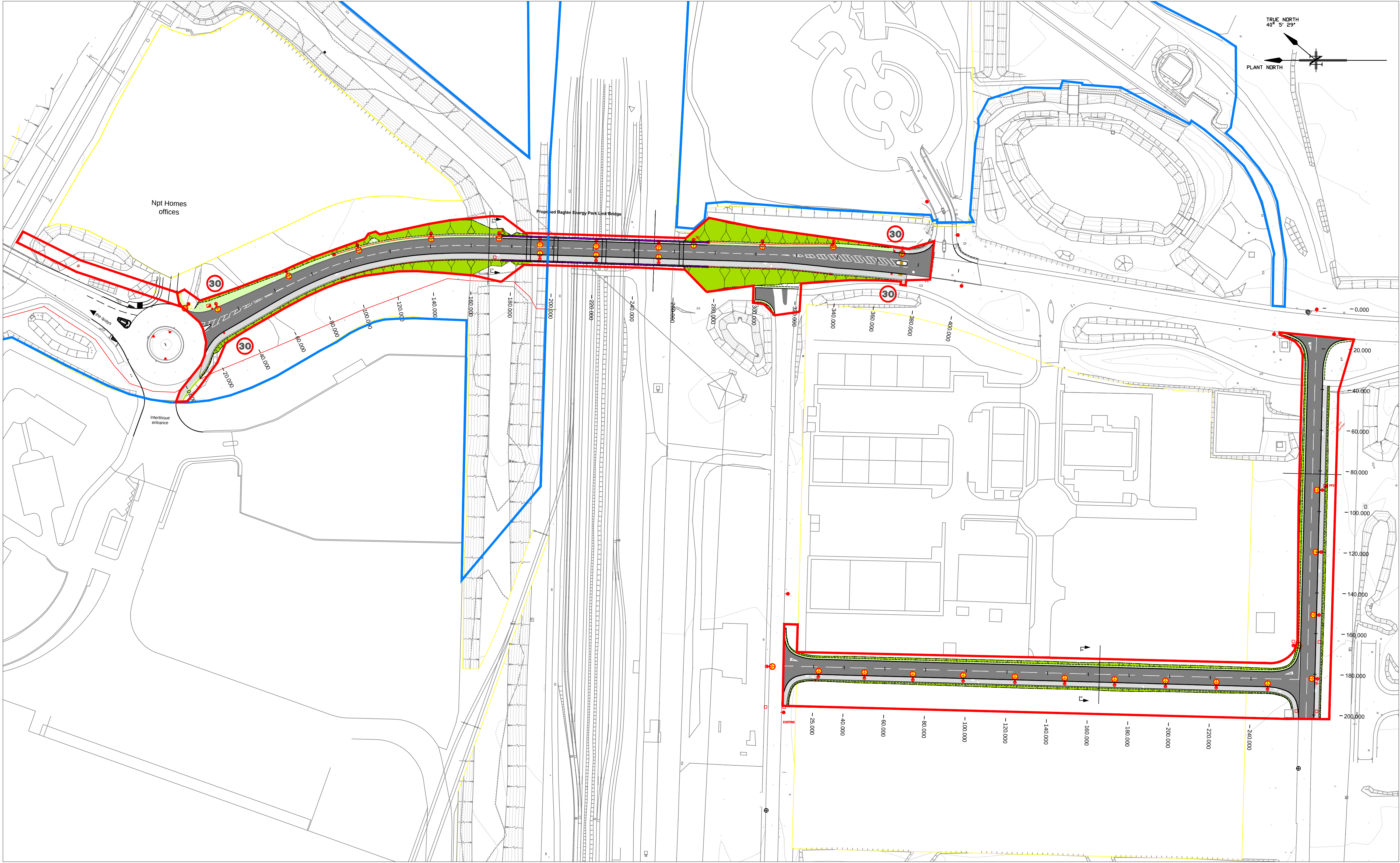
GENERAL ARRANGEMENT - BAGLAN LINK BRIDGE AND ROAD 3 TO 4 LINK ROAD Scale 1:1000
