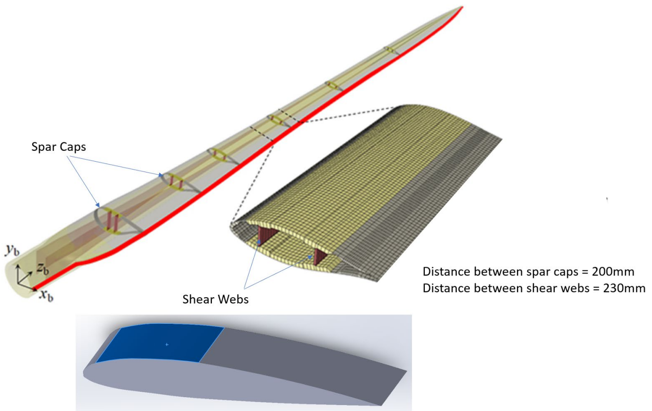
Figure 2: The construction of the wind turbine blade.
