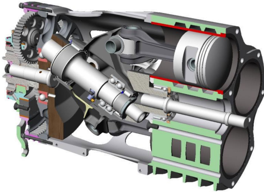
Figure 1, duke engine cutaway (ultimatemotorcycling 2019)
