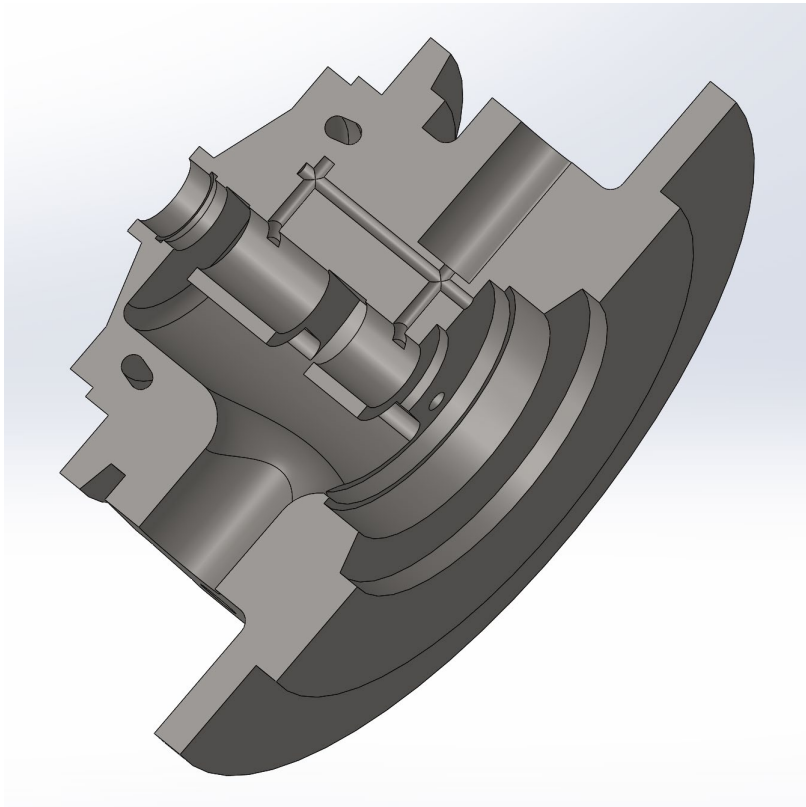
Figure 9, turbo insert cutaway cad model.
