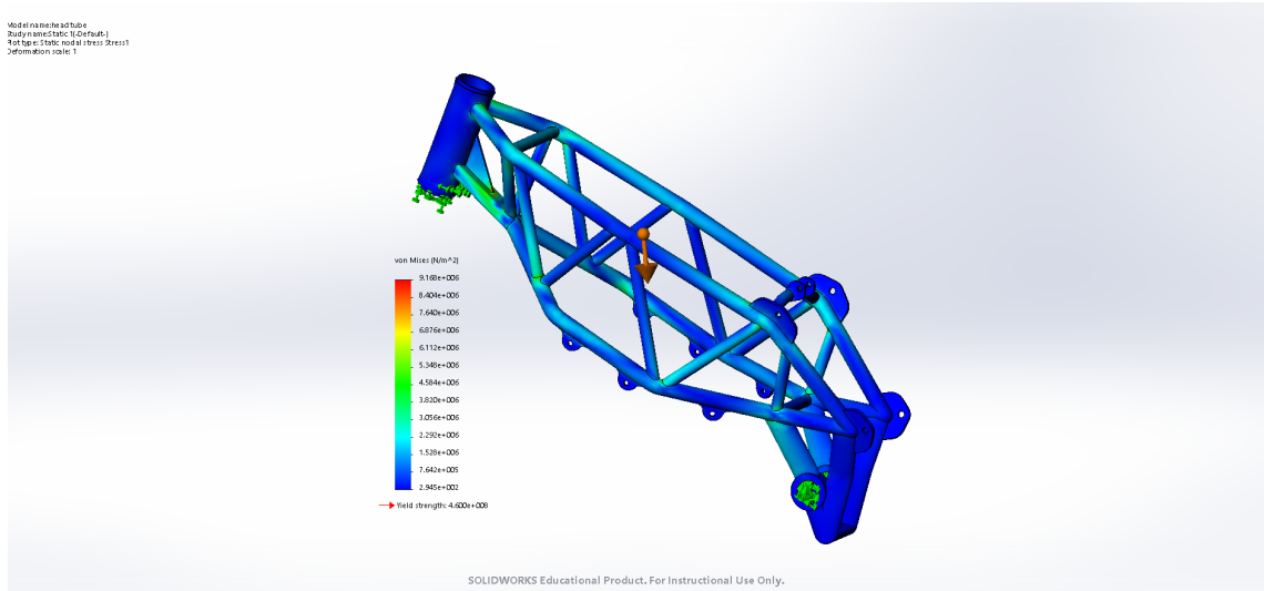
Figure 1, von mises stress evaluation
