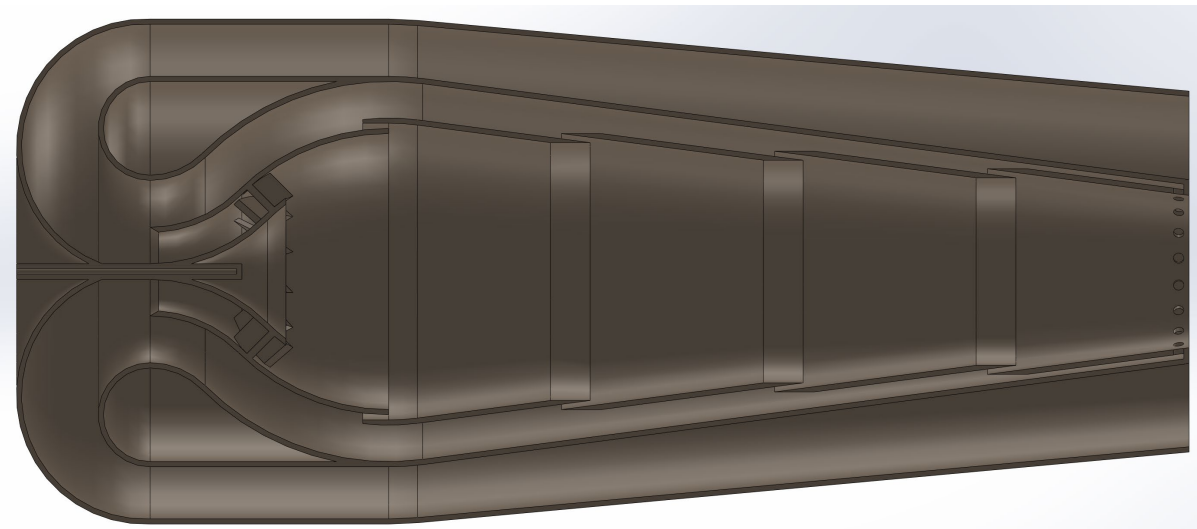
Figure 22, combustor internal features.
