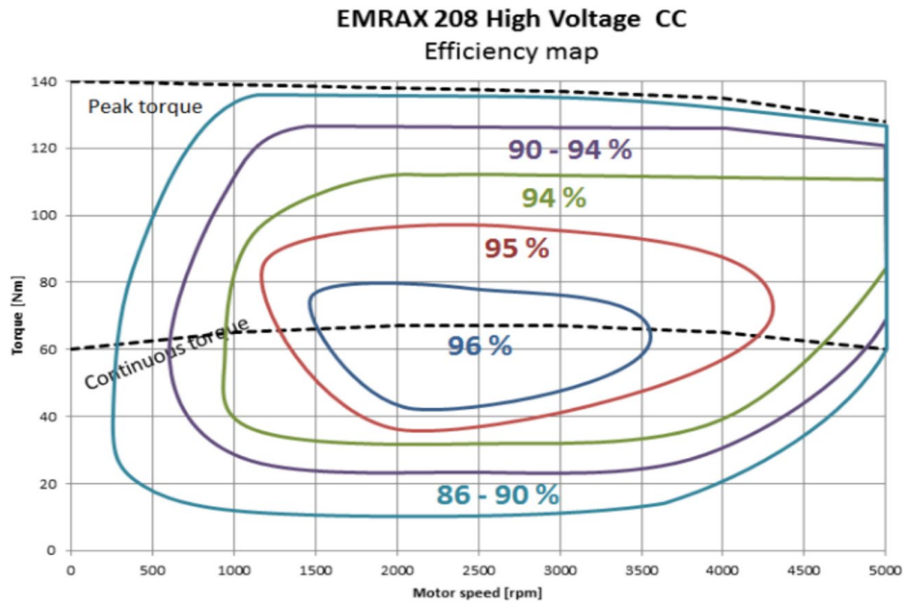
Figure 1, Emrax 208 efficiency
