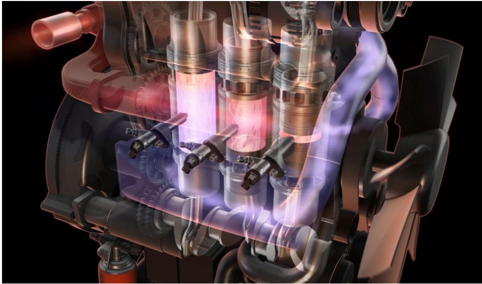
Figure 2, achates engine visualisation (Csere, 2018)
