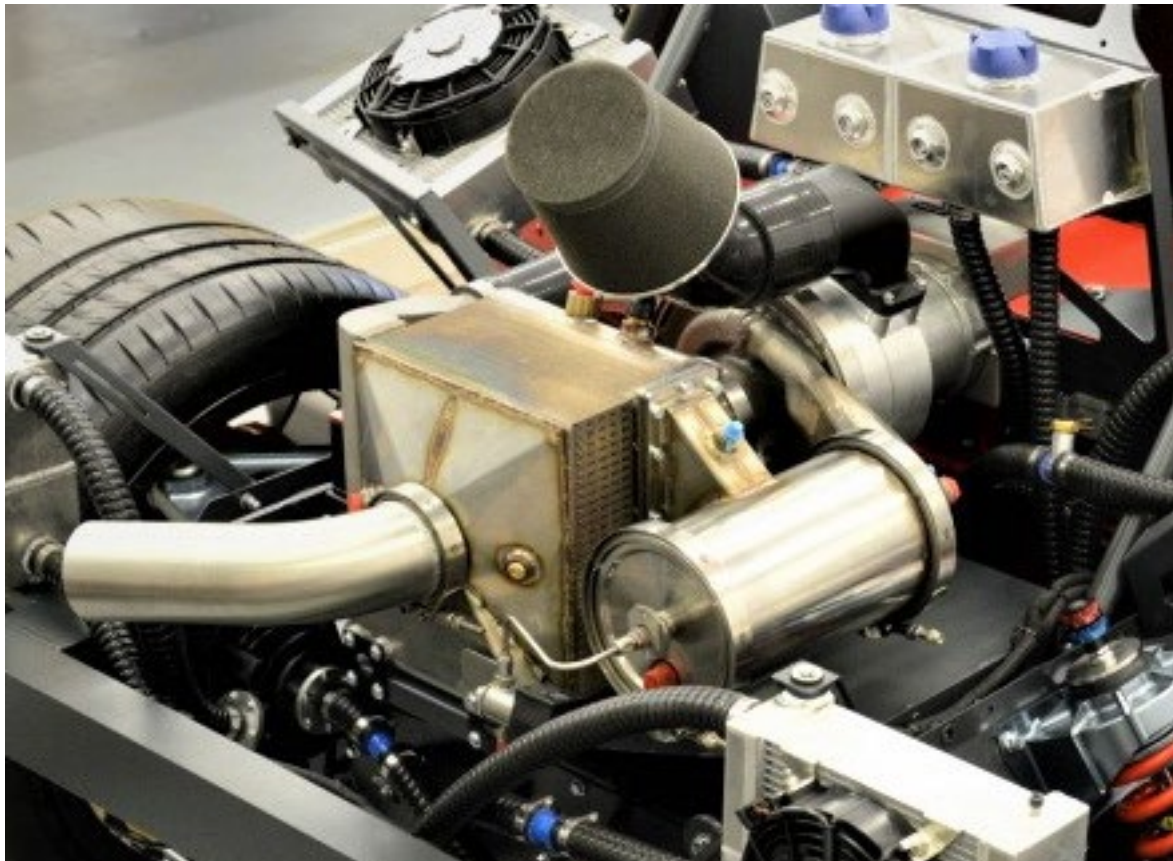
Figure 4, the Ariel Hipercar powerplant by Delta motorsport
