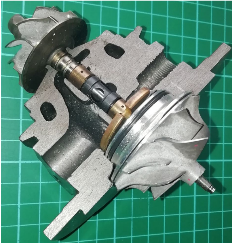
Figure 8, turbo insert cutaway view.
