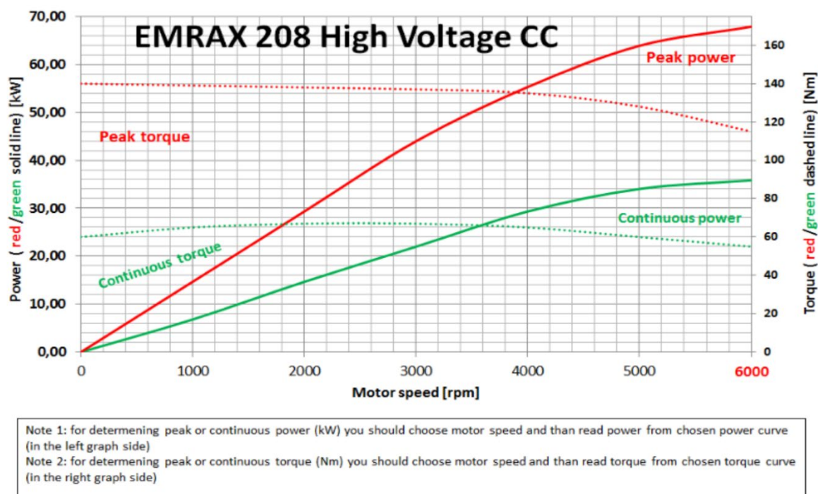
Figure 1, Emrax 208 statistics
