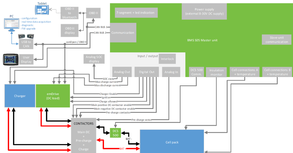
Figure 1, typical wiring system, Emsiso (2018)
