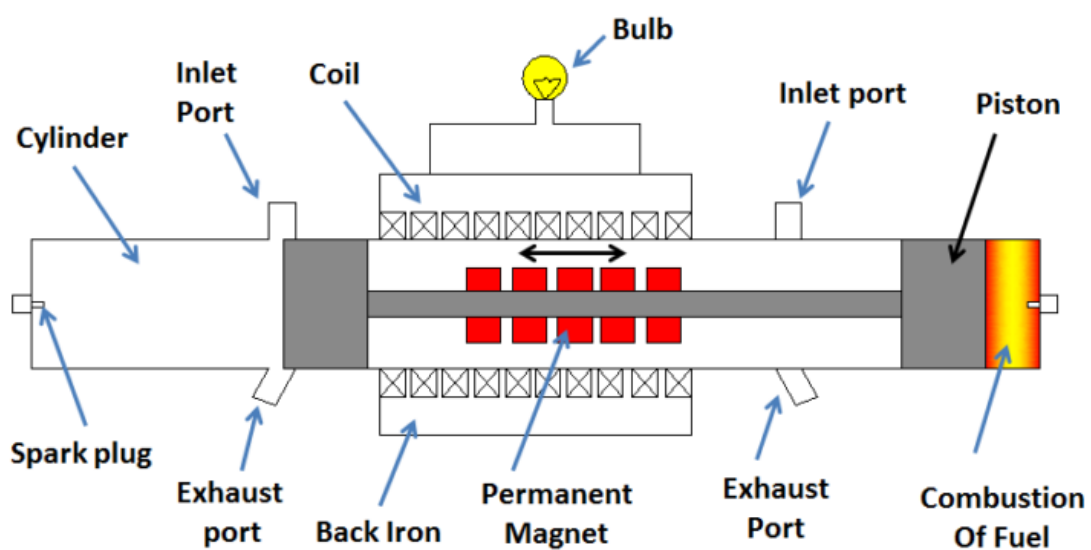
Figure 3, free piston engine detail (Mishra, 2017).
