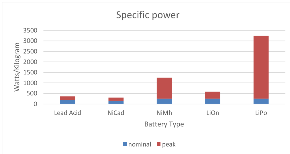
Figure 1, specific power, R Hughes, 2018
