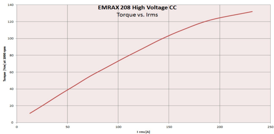
Figure 2, Emrax 208 motor torque to ampere's
