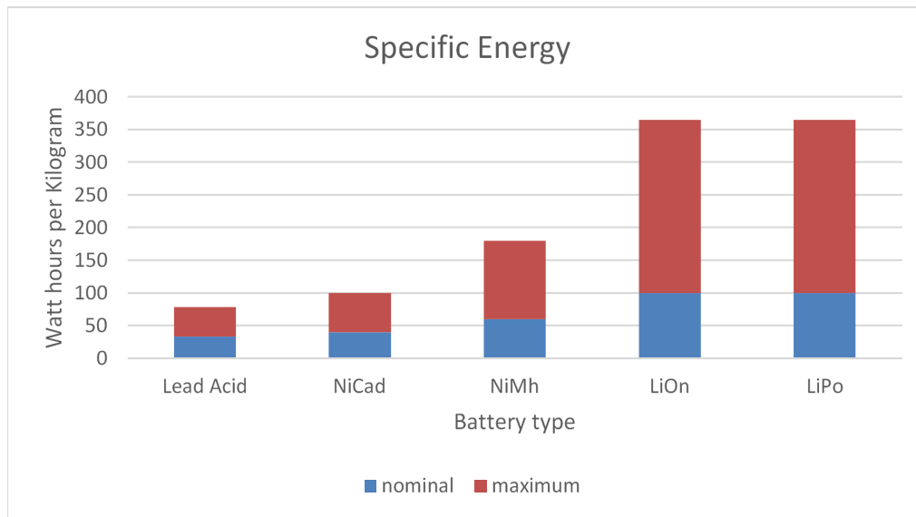
Figure 1, specific energy, R Hughes, 2018
