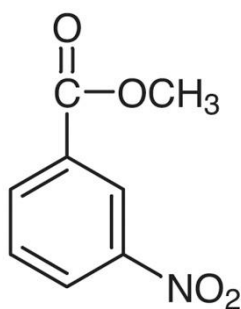
Figure 1 Methyl-3-Nitrobenzoate [9]
