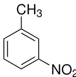
Figure 2 3-Nitrotoluene [8]
