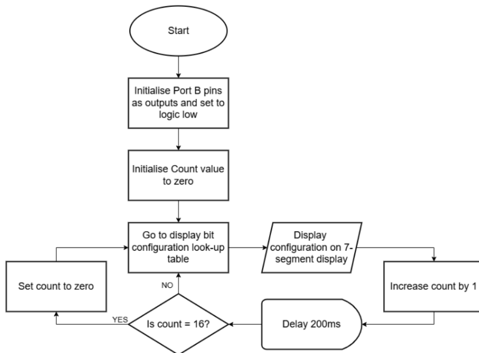
Figure 14. Flowchart illustrating the logical operation of the Counting on the 7-Segment display PIC assembly code.
