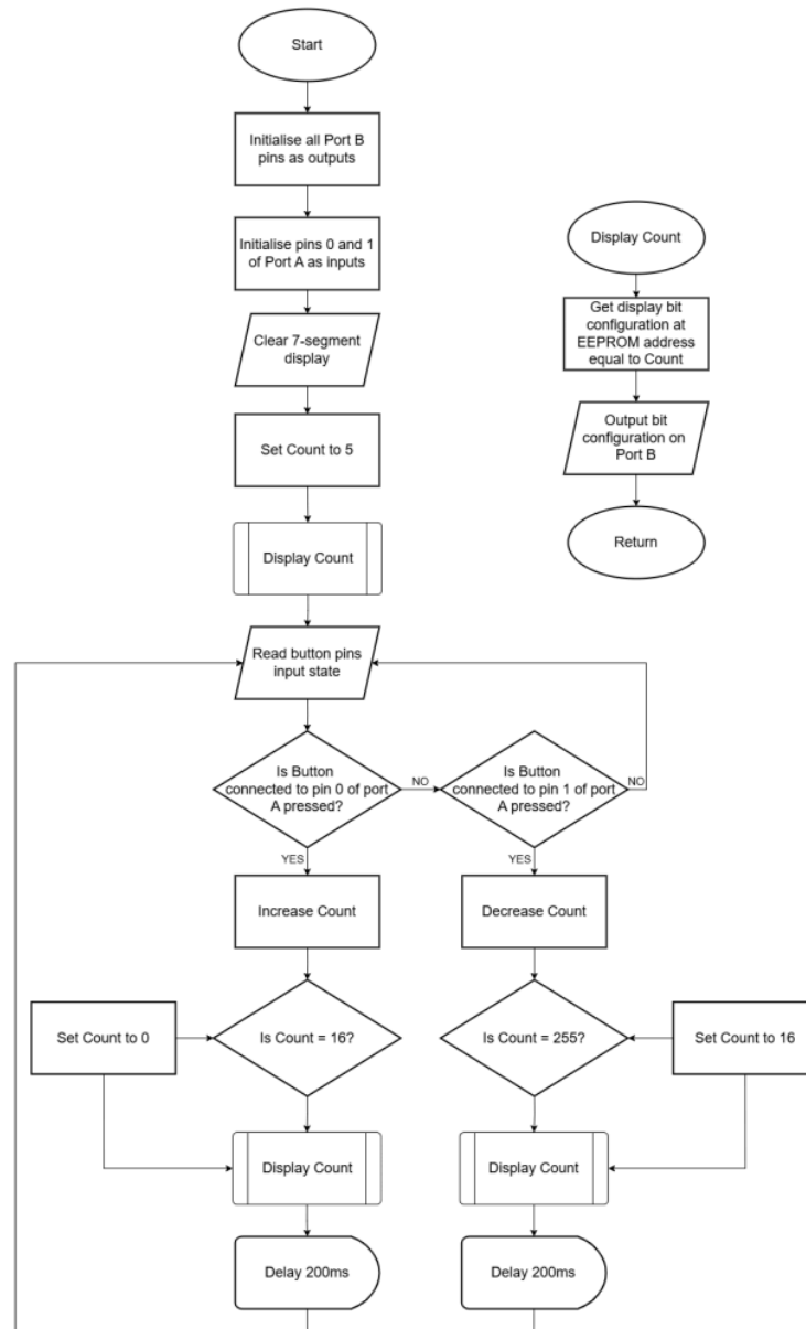
Figure 17. Flowchart illustrating the logical operation of the Counting with Button Inputs PIC assembly code.
