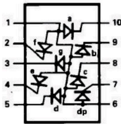
Figure 10. Internal circuit of the HDSP-7801 common anode seven segment display with decimal point [11].
