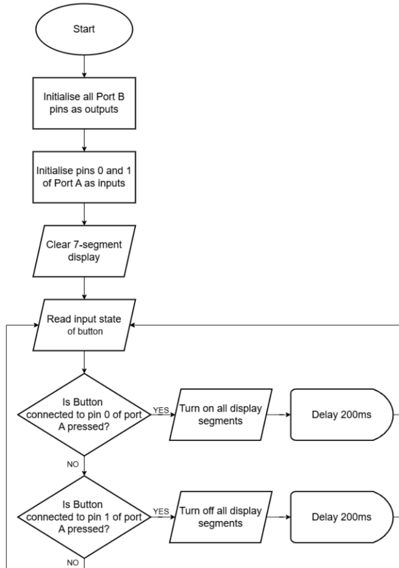
Figure 16. Flowchart illustrating the logical operation of the Counting on the Latching Button Inputs PIC assembly code.
