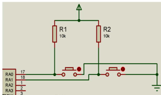
Figure 7. Input buttons connected to 2 pins of Port A of the PIC16F84A in the Assignment Board circuit with pull-up resistors connected to each button.
