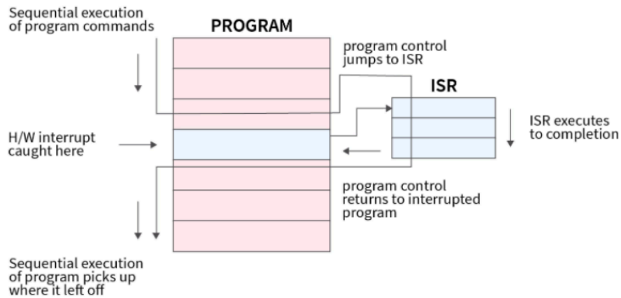
Figure 13. Program flow showing jump to a service routine following interrupt signal [16].
