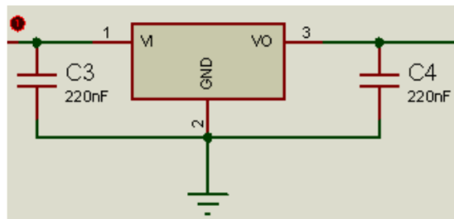
Figure 2. The 7805 regulator from the Assignment Board circuit with supporting capacitors on the input and output.
