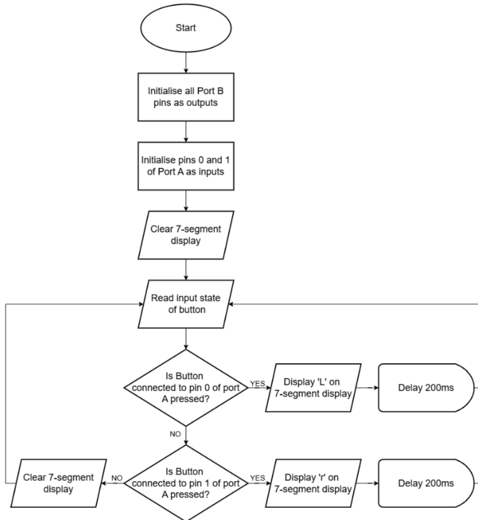
Figure 15. Flowchart illustrating the logical operation of the Using Button Inputs PIC assembly code.
