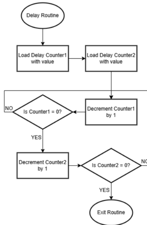
Figure 12. Flowchart showing the logical flow of the delay routine used to created delays on the PIC16F84A.
