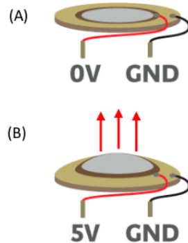
Figure 5. The internal components of a piezoelectric buzzer. (A) shows the state of the buzzer when no potential difference is experienced across the piezoelectric material, with it being undisturbed. (B) shows the result when 5V is applied, which causes the piezoelectric material to deform [15].
