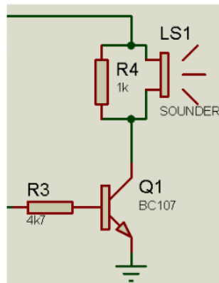
Figure 6. Piezoelectric buzzer with supporting circuitry used within the Assignment Board circuit.
