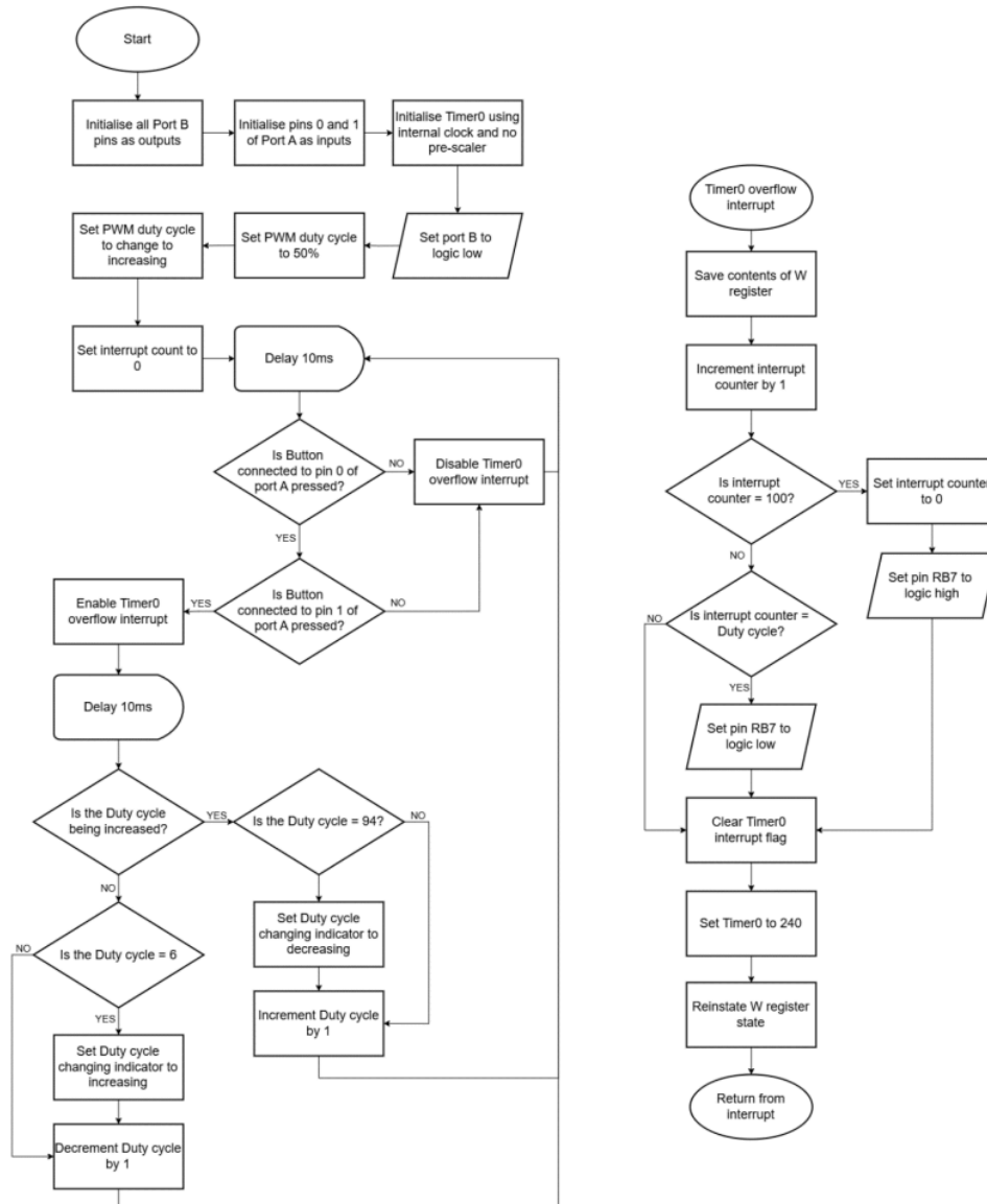
Figure 19. Flowchart illustrating the logical operation of the Changing the Sound of the Piezo Buzzer PIC assembly code.
