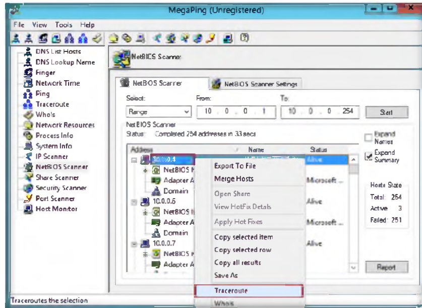
FIGURE 15.8: MegaPing Traceroute
