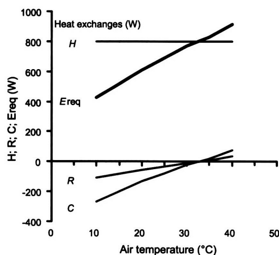
Figure 3 Evaporative requirement ( E_{\text{req}} ) in laboratory exercise. H is the exercise heat production; relative humidity 70%; radiant temperature = air temperature; air velocity = 2.0 m s -1 . R is the radiant heat transfer; C is the convective heat transfer; E_{\text{req}} is the required evaporative cooling; E_{\text{max}} is the environmental evaporative capacity. Negative values denote heat loss. Subject characteristics as for Fig. 1. Heat stress increases with increase in air temperature because of loss of convective cooling ( T_a < 35^\circ\text{C} ), or heat gain by convection ( T_a > 35^\circ\text{C} ), thus increasing requirement for cooling by sweat evaporation.
