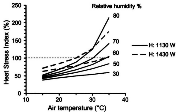
Figure 7 Heat stress index for free running at 4.5 \text{ m s}^{-1} ( 16 \text{ km h}^{-1} ). Effects of air temperature, humidity and running economy. Air velocity = running speed. HSI for H : 1430 W at 50 and 70% relative humidity. HSI 100% marks upper limit of prescriptive zone for thermoregulation. Subject details as in Fig. 2.
