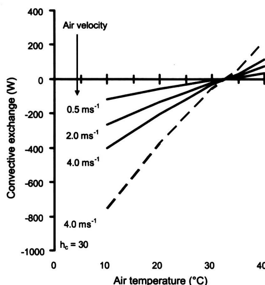
Figure 2 Convective heat exchange ( C ) in laboratory exercise; effects of air temperature and air velocity. Cycle ergometer; subject surface area 1.8 m 2 . Air velocities 0.5, 2.0 and 4.0 m s -1 . Negative values denote heat loss. The broken line denotes convective exchange for free running at 4.0 m s -1 calculated with convective coefficient h_c = 30 (see text). 39,40 Convective heat exchange is determined by the skin to air temperature gradient (Fig. 1A), and air velocity.
