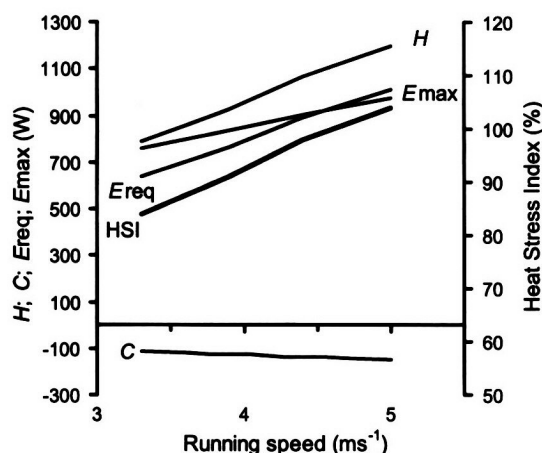
Figure 6 Heat exchanges in free running. Air temperature = 25°C; relative humidity = 70%; vapour pressure = 2.2 kPa; air velocity = running speed. Subject characteristics as for Fig. 2, details as for Figs. 3 and 5.
