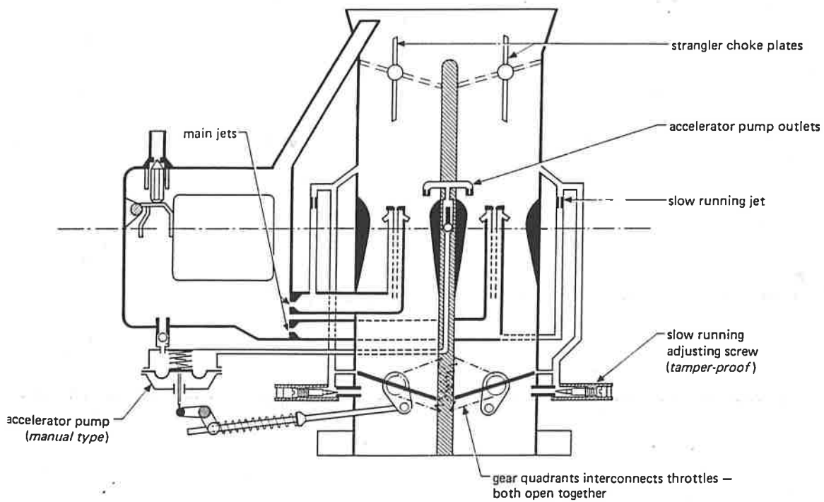
Twin-choke carburetter
