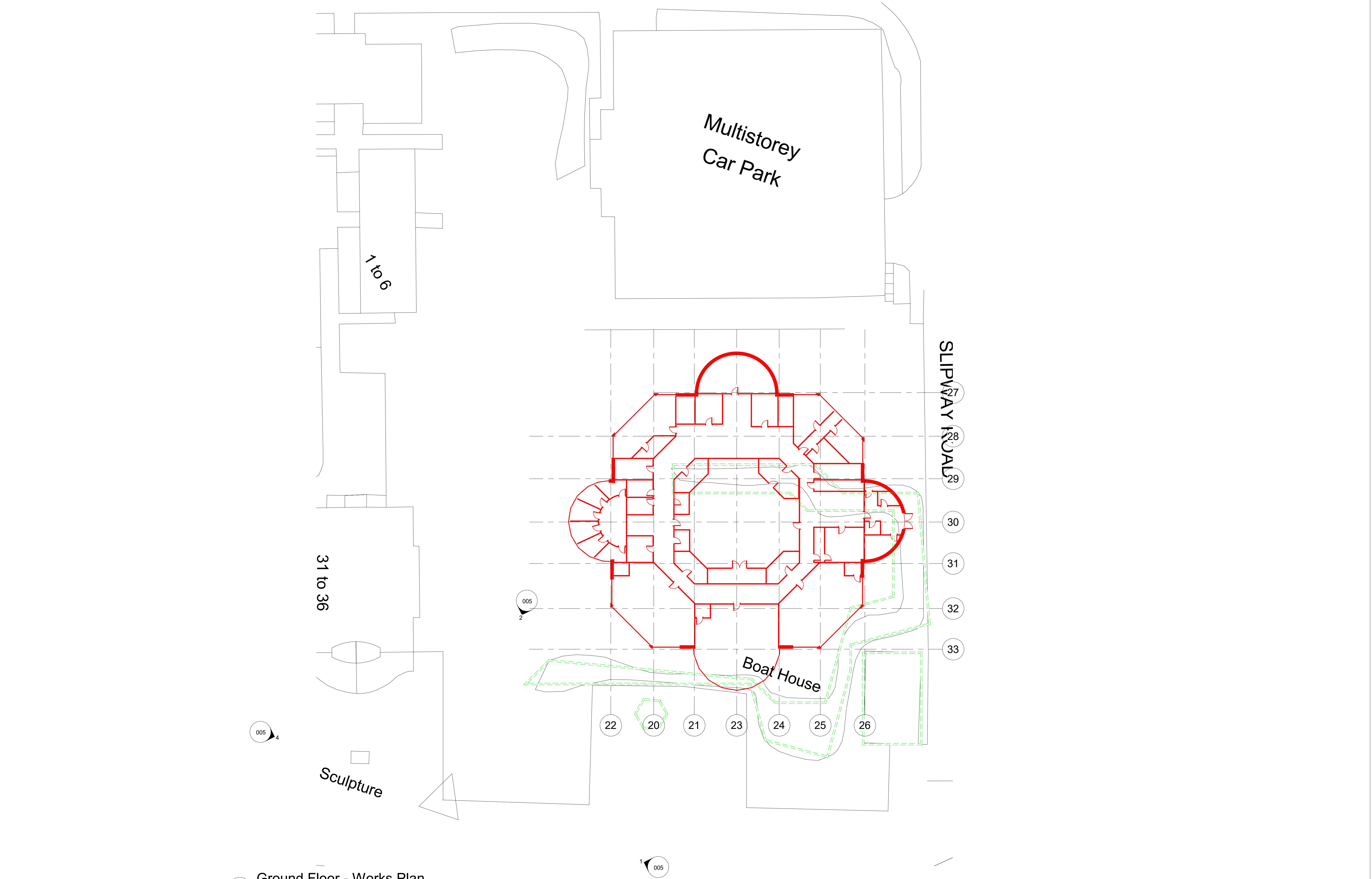
1 Ground Floor - Works Plan 1 : 200
