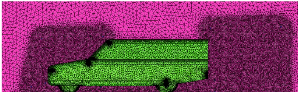
Figure 3 – Final mesh surrounding MIRAESTATE geometry
