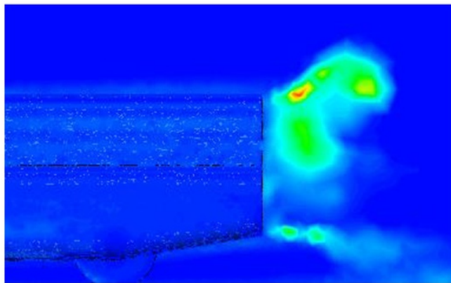
Figure 6 – Contour plot showing eddy current viscosity
