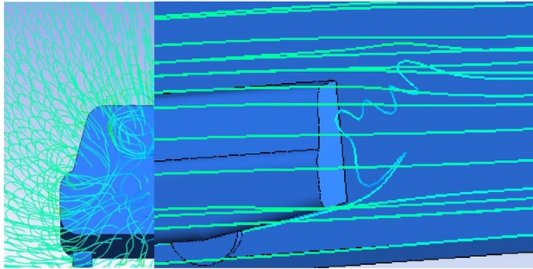
Figure 5 – Flow lines showing vortices
