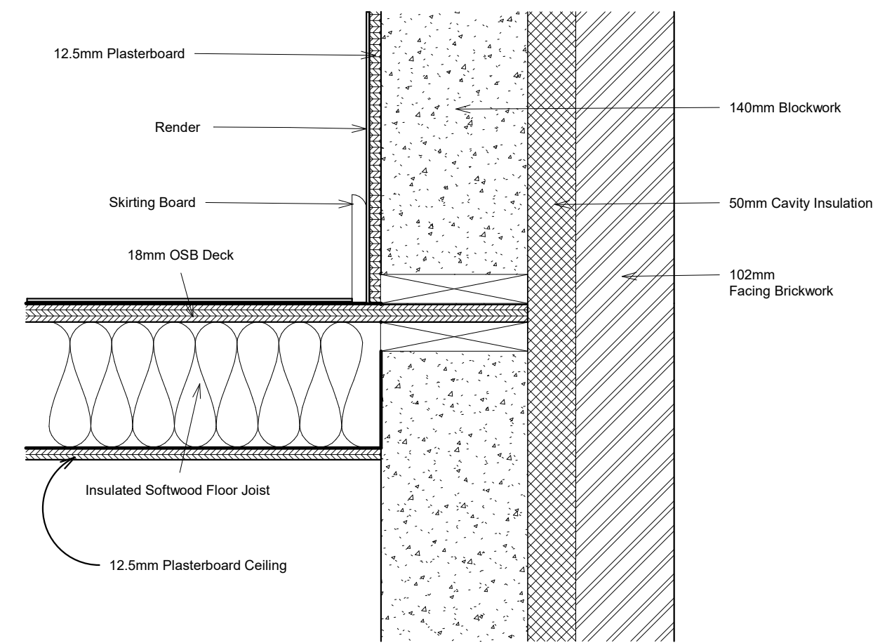
3 Wall to First Floor Detail 1 : 5
