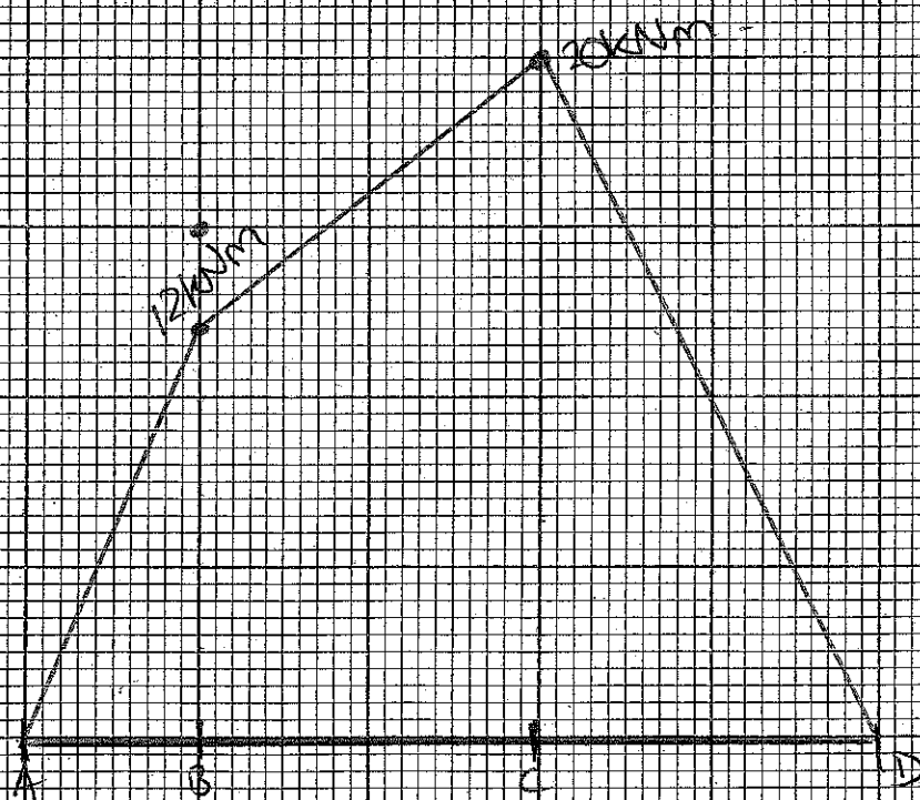
Bending Moment Diagram
