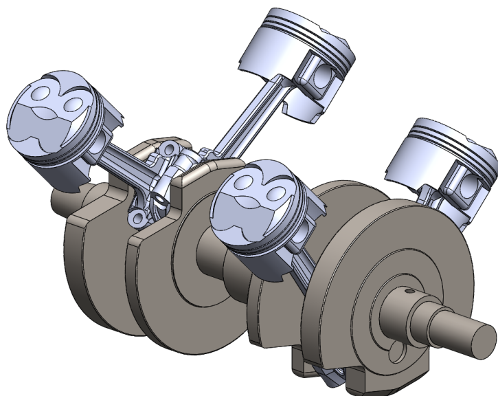
Figure 6 VFR400 CAD model
