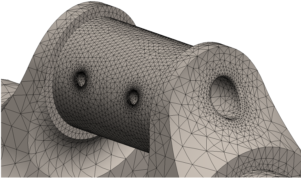
Figure 18 close view of big end journal and oil hole meshing
