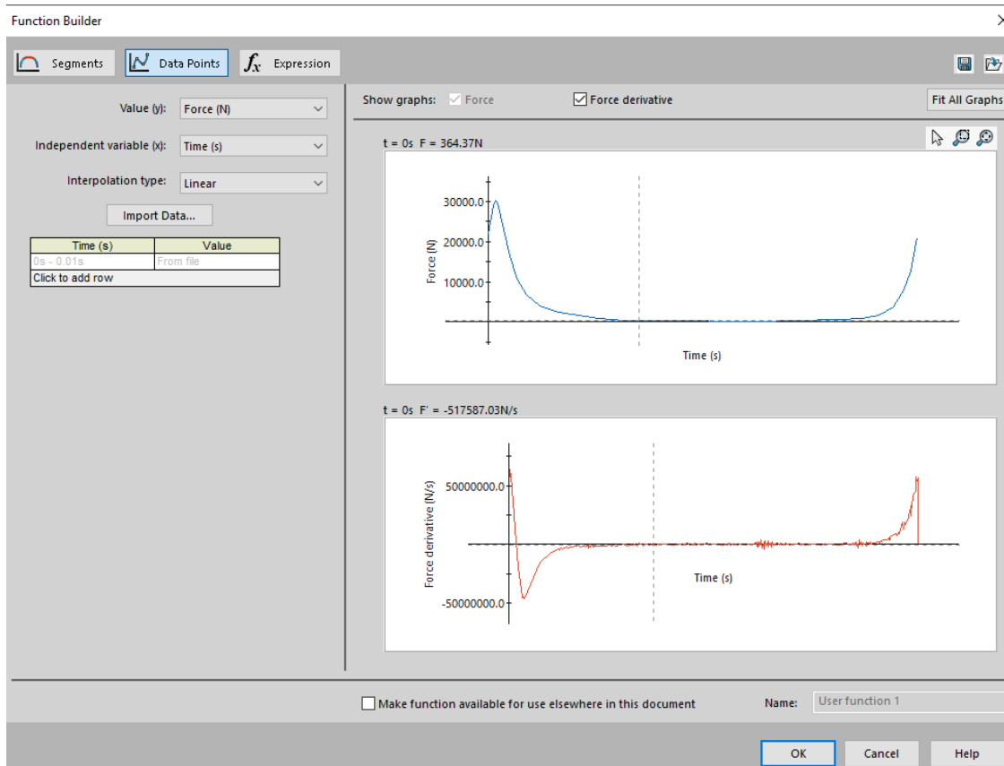
Figure 15 Cylinder 2 Solidworks data points plot
