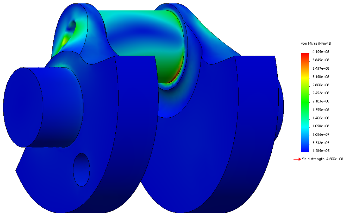
Figure 19 FEA stress concentration, compressive zone (von mises stress)
