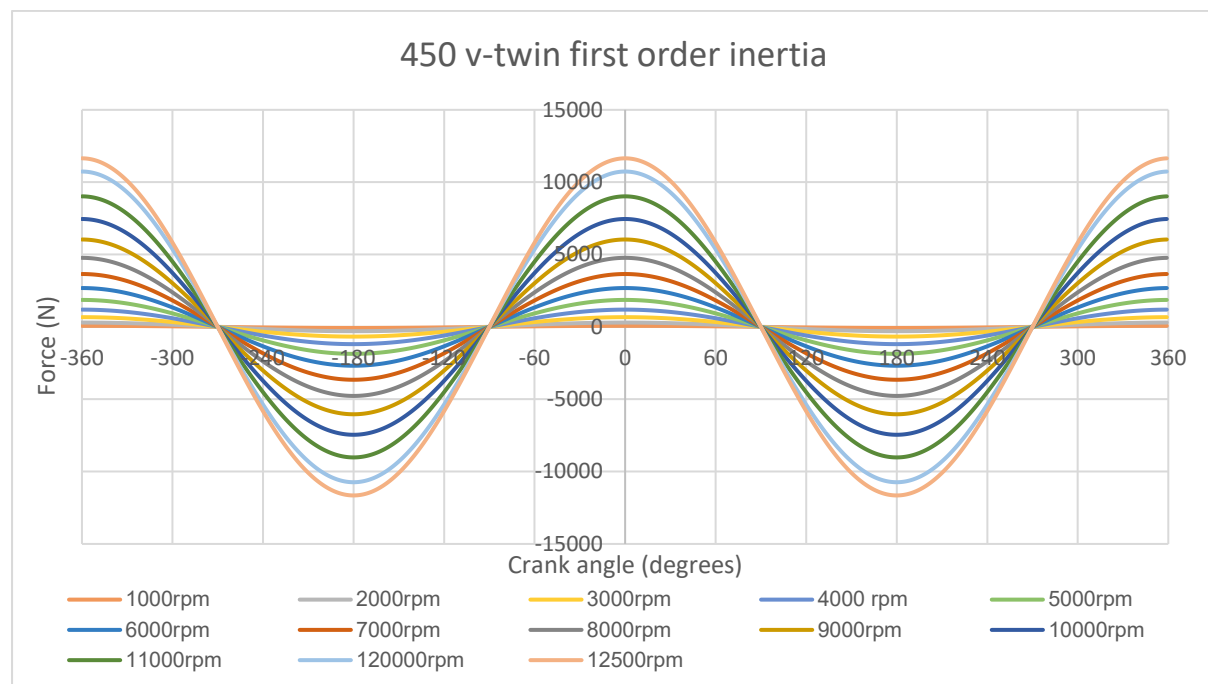
Figure 8 450 v-twin first order inertia
