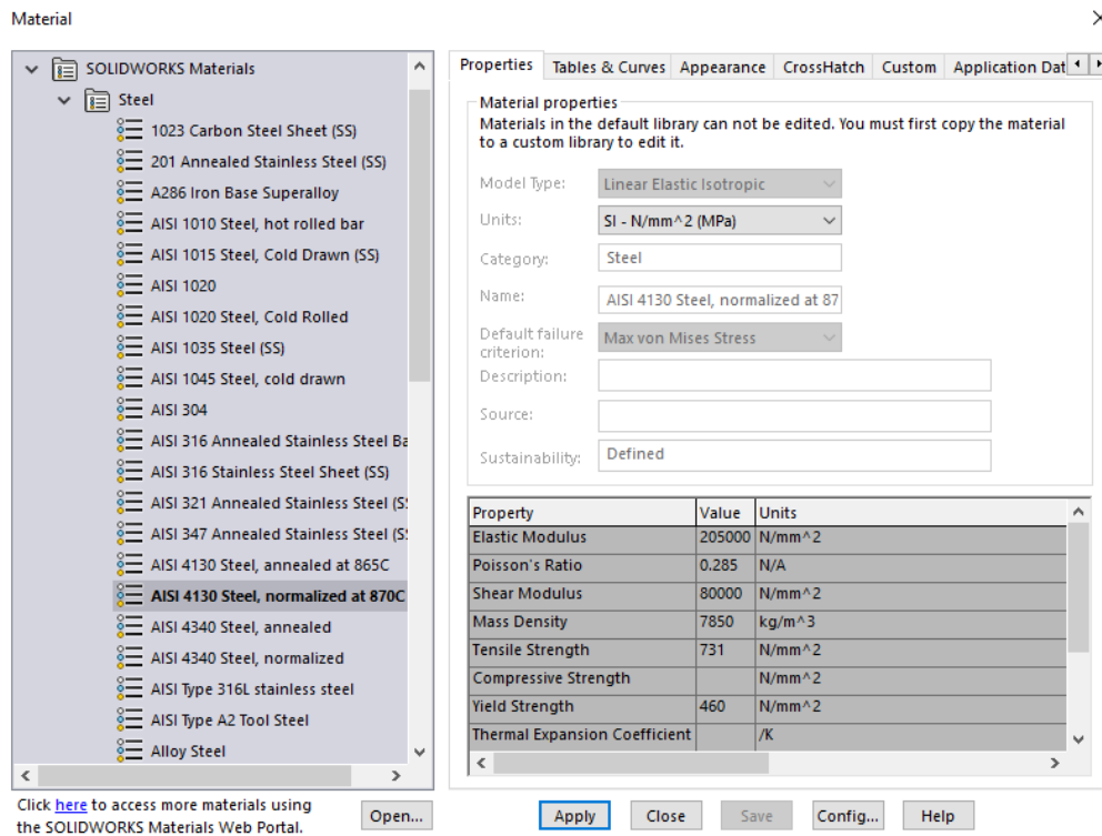
Figure 20 4130 steel material selection in Solidworks
