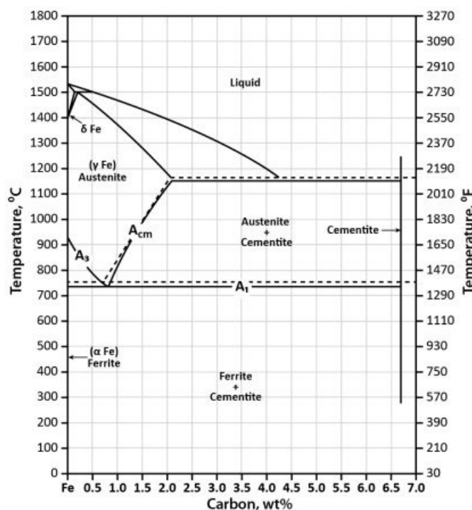
Figure 31 steel phase diagram (Industrial Metallurgists LLC, 2019)
