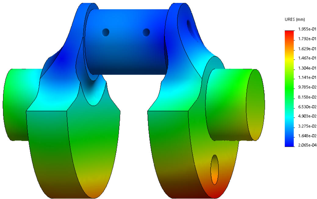
Figure 25 FEA Displacement
