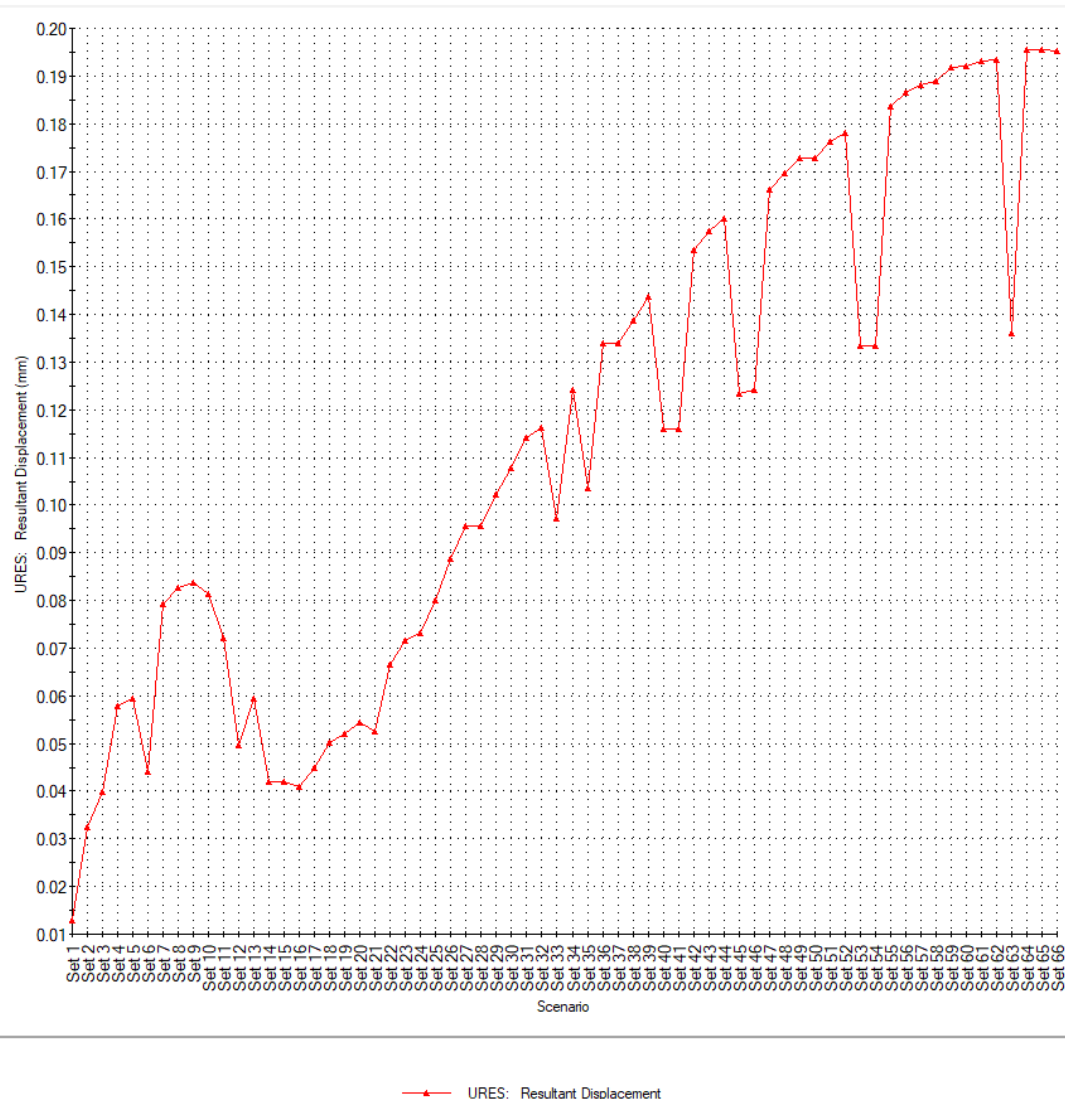
Figure 26 Displacement plot
