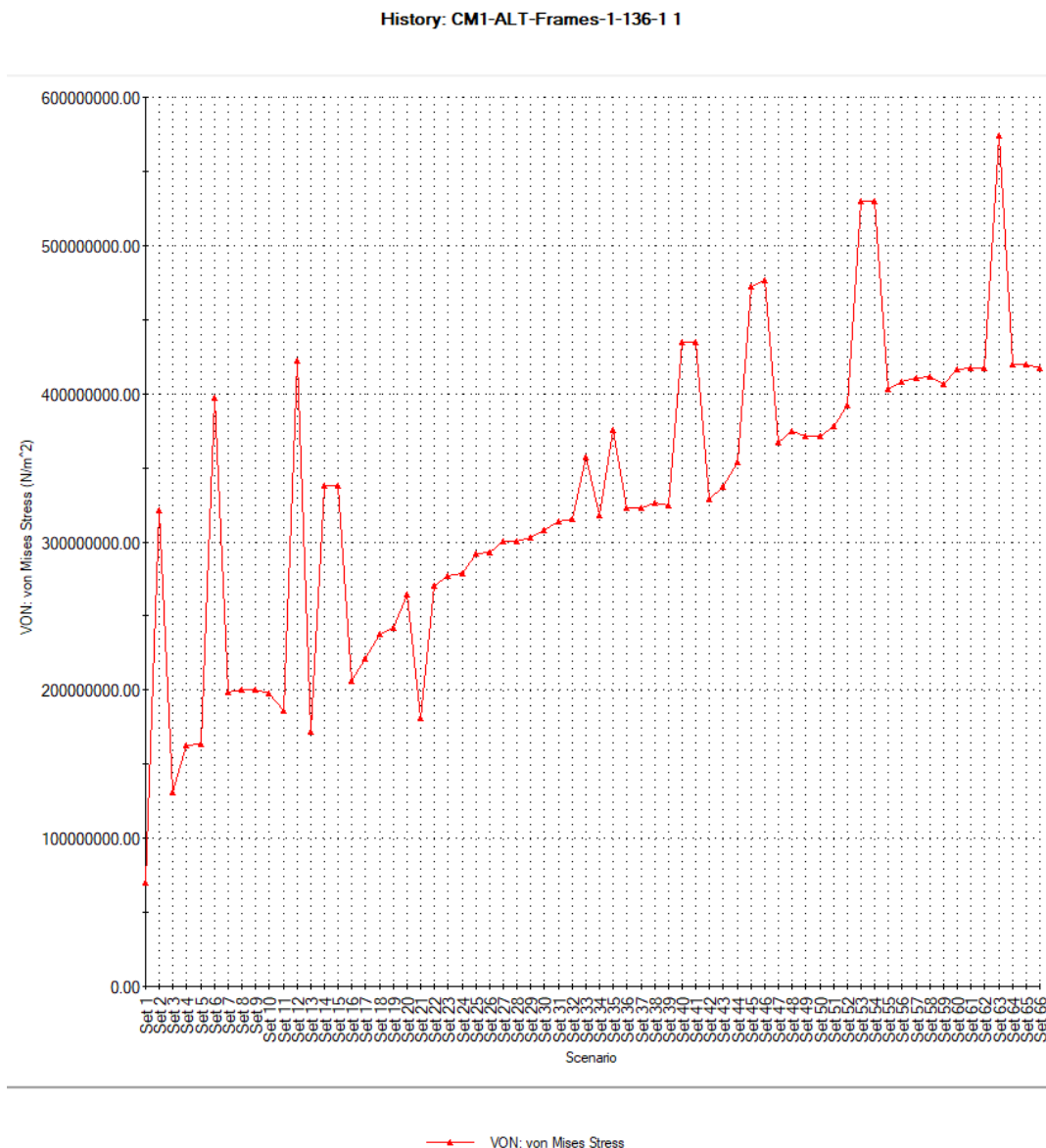
Figure 22 Von Mises stress plot
