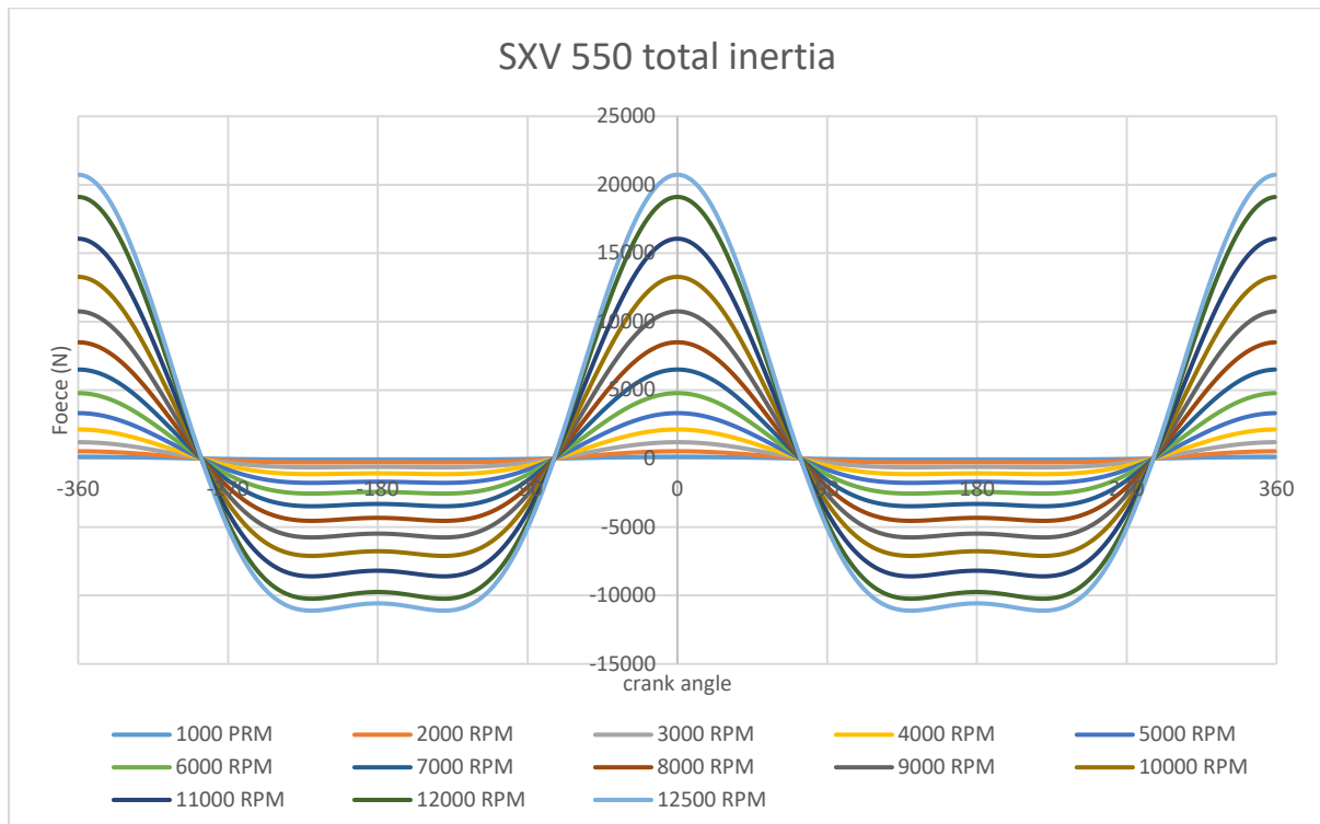
Figure 11 SXV550 total inertia
