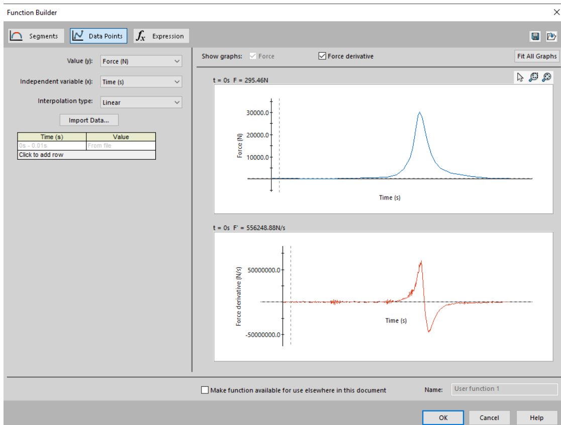
Figure 16 Cylinder 1 Solidworks data points plot
