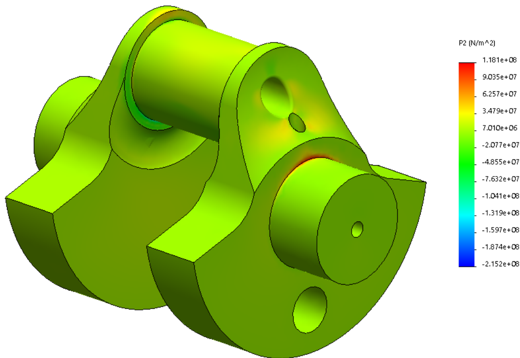
Figure 23 FEA stress concentration, tensile zone (2 nd principal stress)
