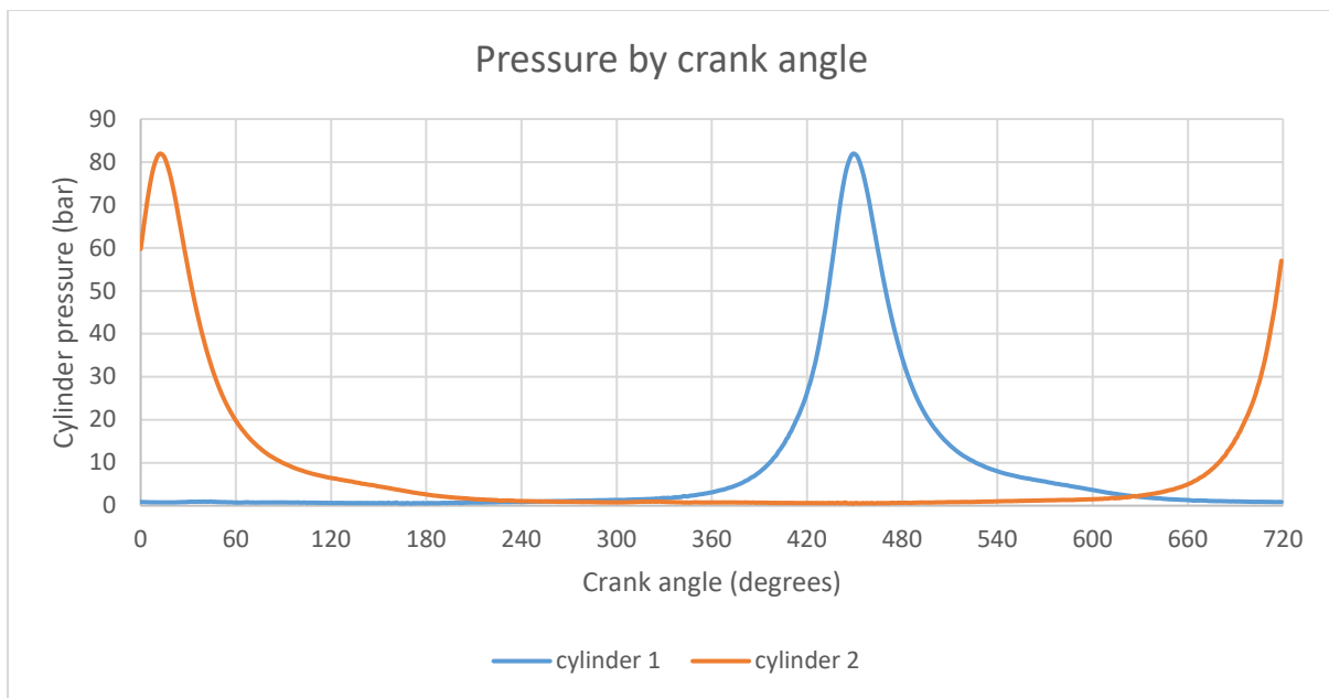
Figure 14 Pressure by crank angle
