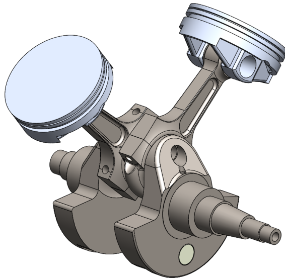
Figure 4 SXV550 CAD model
