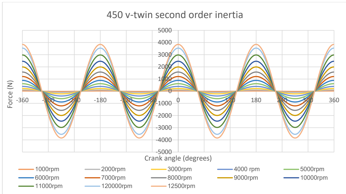
Figure 9 450 v-twin second order inertia
