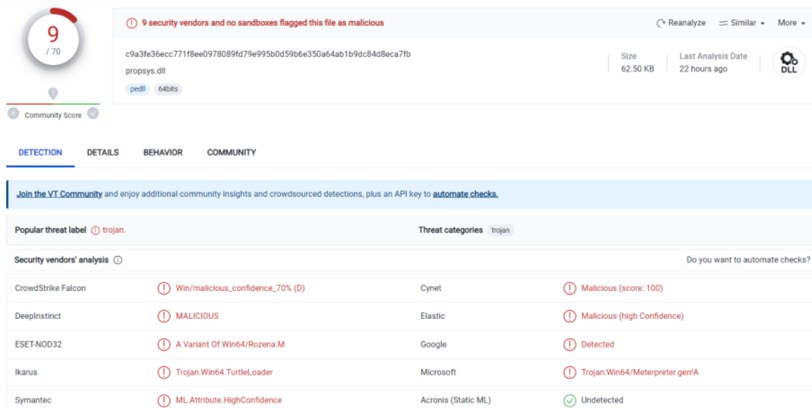
Fig. 47. VirusTotal.com results of the infected .dll file.
