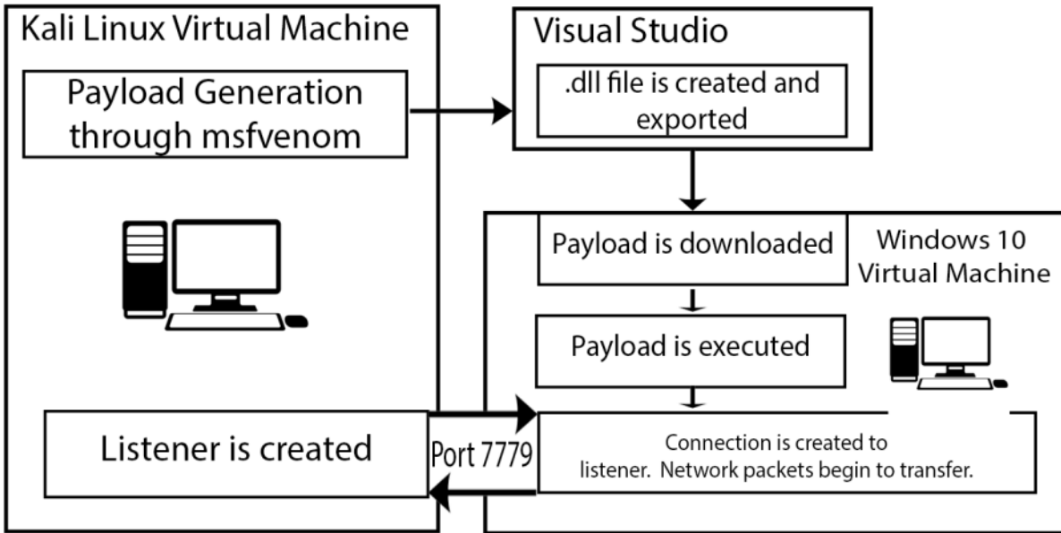
Fig. 19. Structure of data flow and network traffic.
