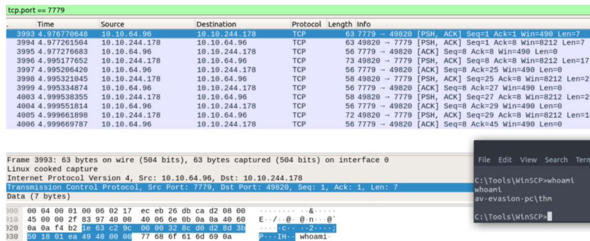
Fig. 50. Packets being sent and recieved through the reverse shell connection after a whoami command, displayed with Wireshark.
