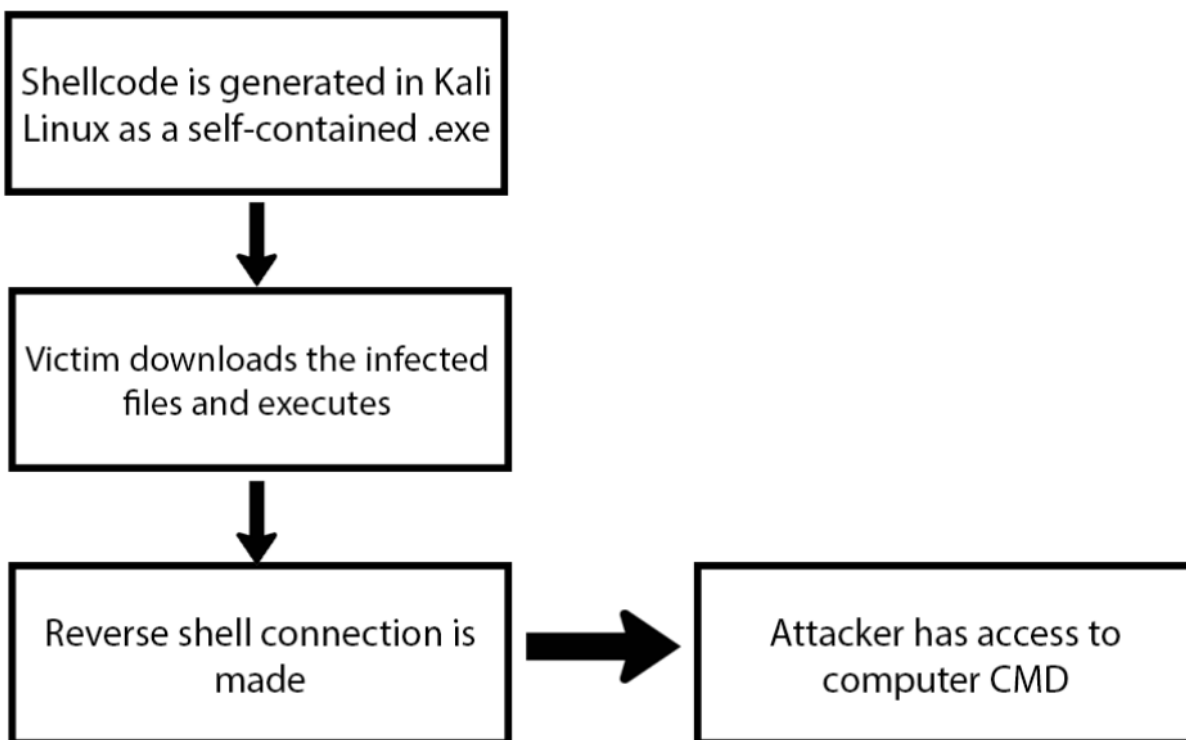
Fig. 6. Block diagram of how an encrypted shellcode reverse shell virus will operate.
