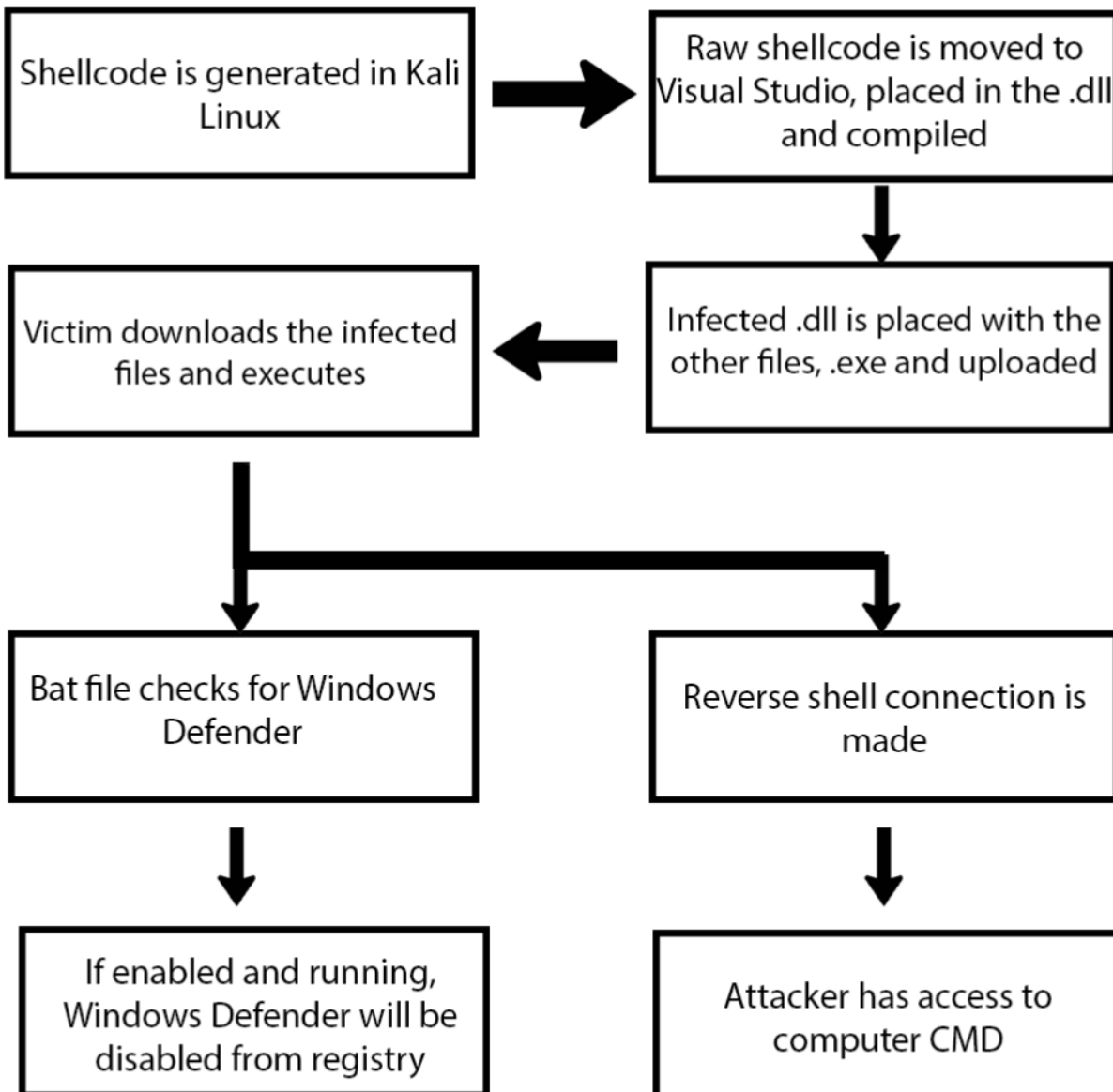
Fig. 5. Block diagram of how a .dll infected virus will operate.
