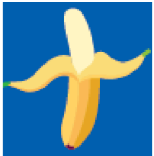
banana
