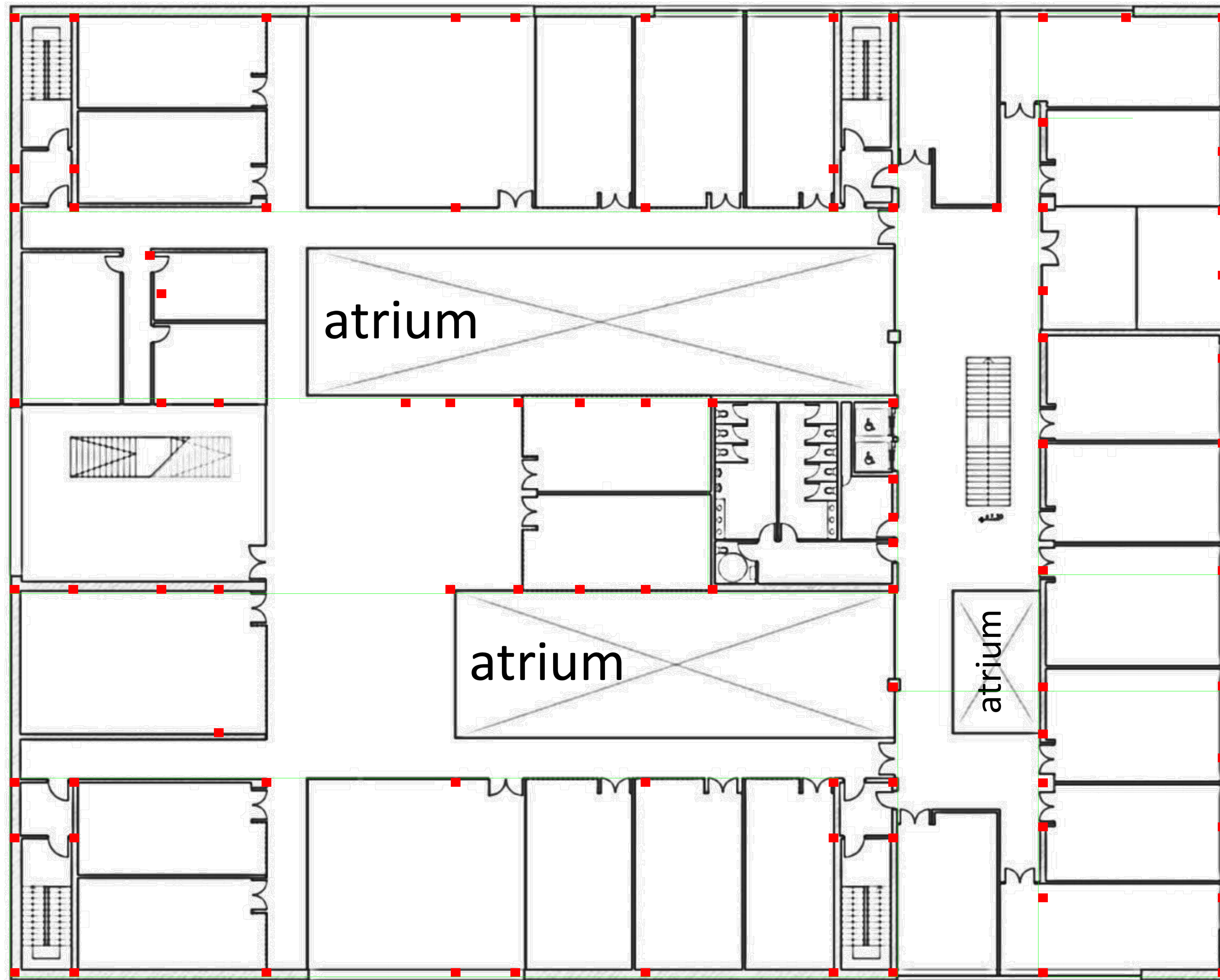
Second Floor Plan 1:500 approx
