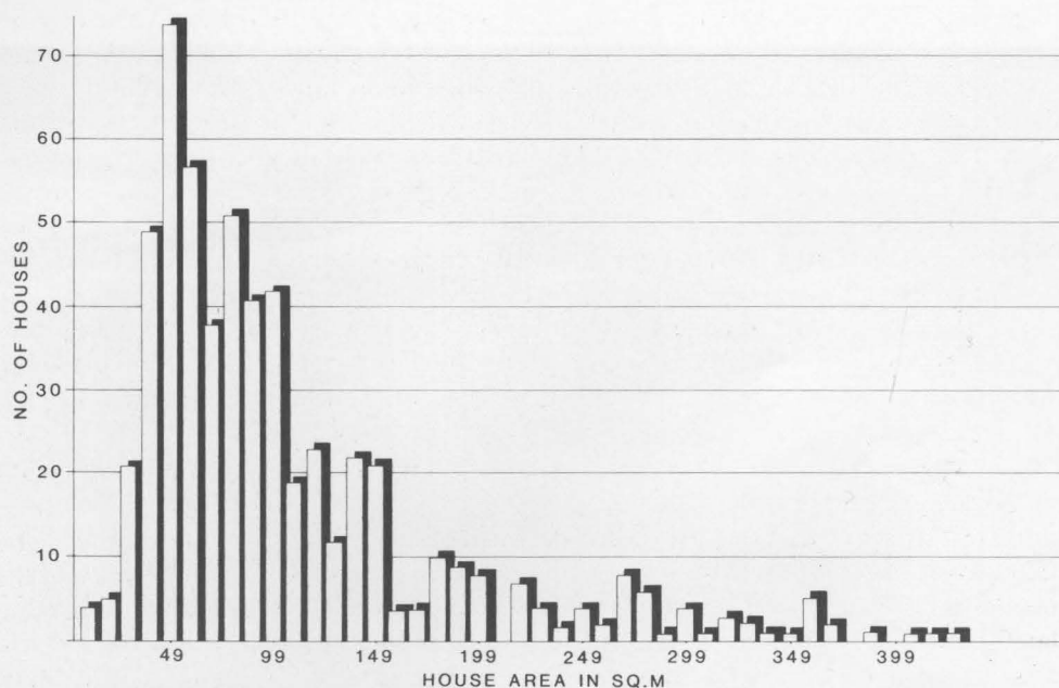
Figure 101 Bar-chart showing the frequencies of houses of varying sizes within the Main City at Amarna. House sizes are given in steps of 10 sq. metres. The regularity of the curve of distribution is striking. After Piers Crocker, unpublished dissertation, University of Cambridge, and cf. 'Status symbols in the architecture of El-'Amarna', Journal of Egyptian Archaeology 71 (1985), 52-65.
