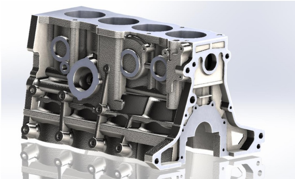
Figure 3-21 7A-FE block modelled using 4A-GE dimensions
