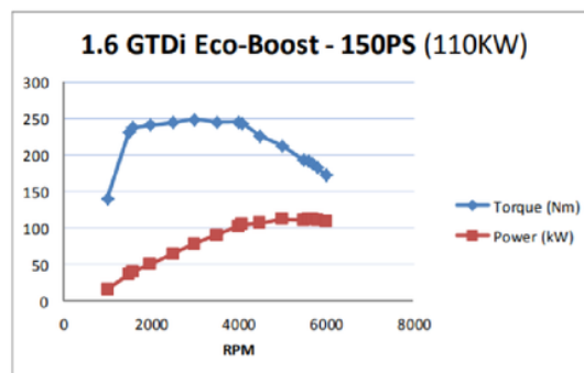
Figure 2-1 Power & Torque curve of EcoBoost (Ford-Uk, 2017)
