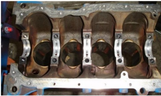
Figure 3-14 7A-FE crankcase, note the machined areas at the base of the bores for the conrods to clear.
