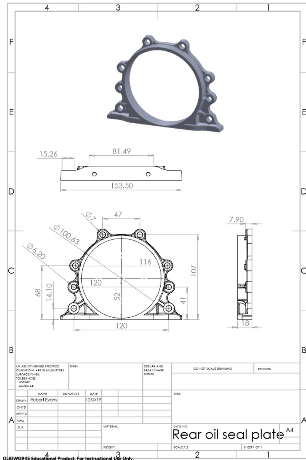
Figure 8-9 Rear oil seal plate to fit larger diameter Ecoboost crankshaft oil seal on flywheel flange (Evans, 2019)
