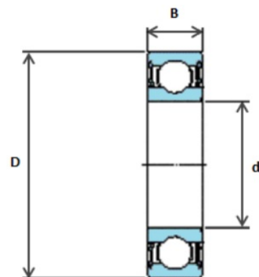
Figure 4-7 Bearing dimension guide, (bearingboys.co.uk, 2019)
