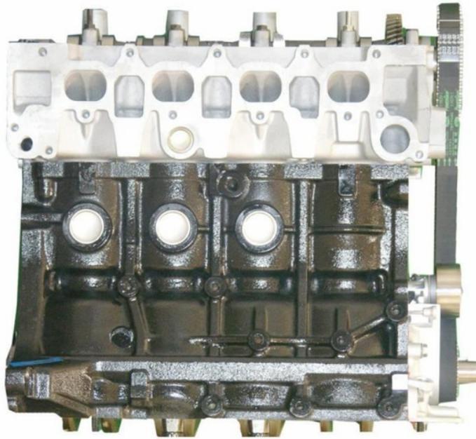
Figure 8-6 Toyota 7A-FE 1.8l engine block & cylinder head
