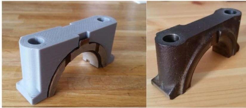
Figure 4-9 3d printed modified centre main bearing cap to allow for thrust washers to fit Ecoboost crank & original 4A-GE (Evans, 2019)
