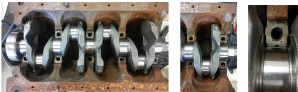
Figure 3-13 Ecoboost crank sitting in 4A-GE Block. notice clearance issue on centre image. image on left shows centre main where thrust washer seats need machining to suit crank
