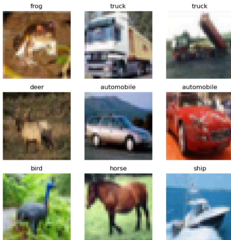
Figure 2: Dataset Classes
