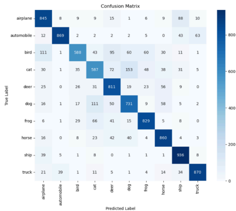
Figure 8: Confusion Matrix
