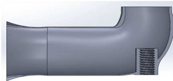
FIGURE 119: PORT 4 REDUCED SHORT TURN RADIUS
