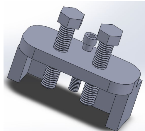
FIGURE 28: TOP VIEW OF CAD VALVE OPENING TOOL
