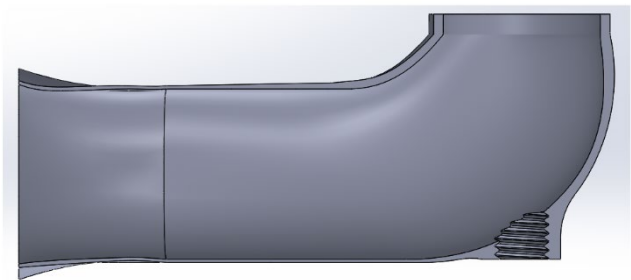
FIGURE 123: PORT 8, INCREASED SHORT RAD, INCREASED LONG RAD AND SMOOTHED GUIDE
