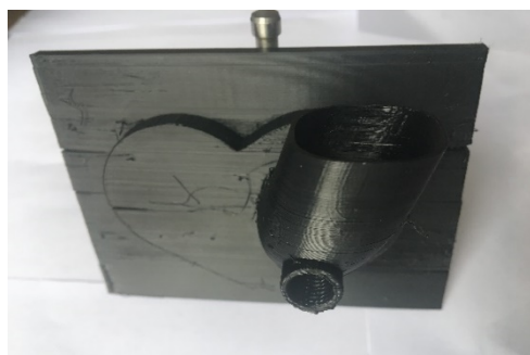
FIGURE 110: PRINT OF PHASE 3 DESIGN
