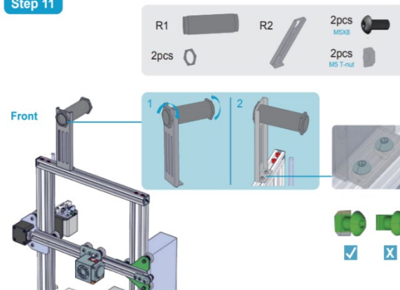
FIGURE 92: CREATILTY ENDER 3 ASSEMBLY GUIDE PART 11
