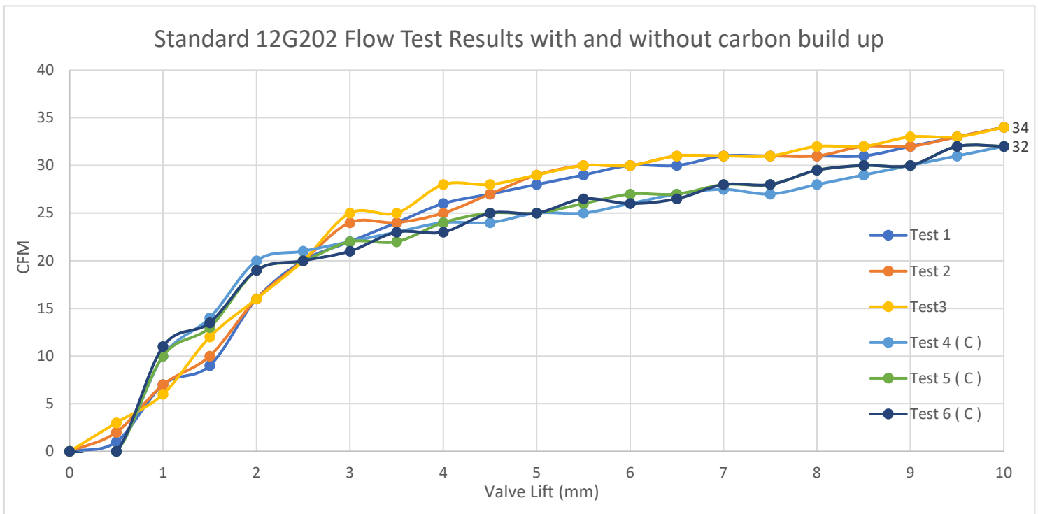
FIGURE 60: STANDARD FLOW TEST RESULTS WITH CARBON BUILD UP
