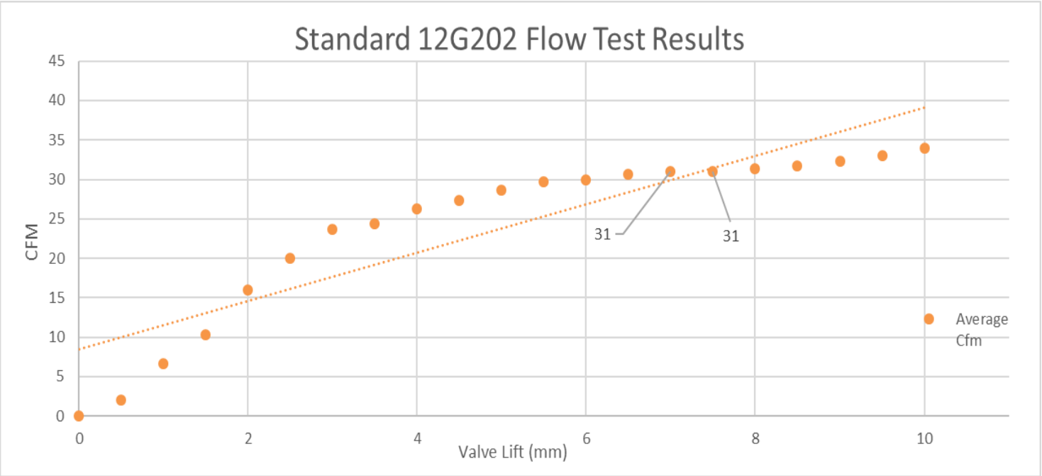
FIGURE 58: AVERAGE STANDARD FLOW TEST RESULTS
