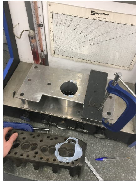
FIGURE 46: CYLINDER HEAD AND CLAMP
