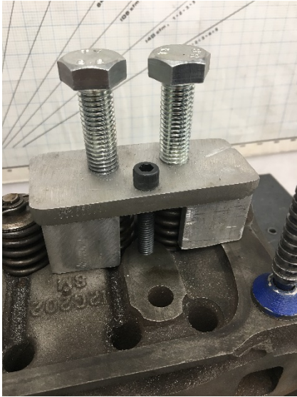
FIGURE 49: BOLTING ON VALVE OPENING TOOL
