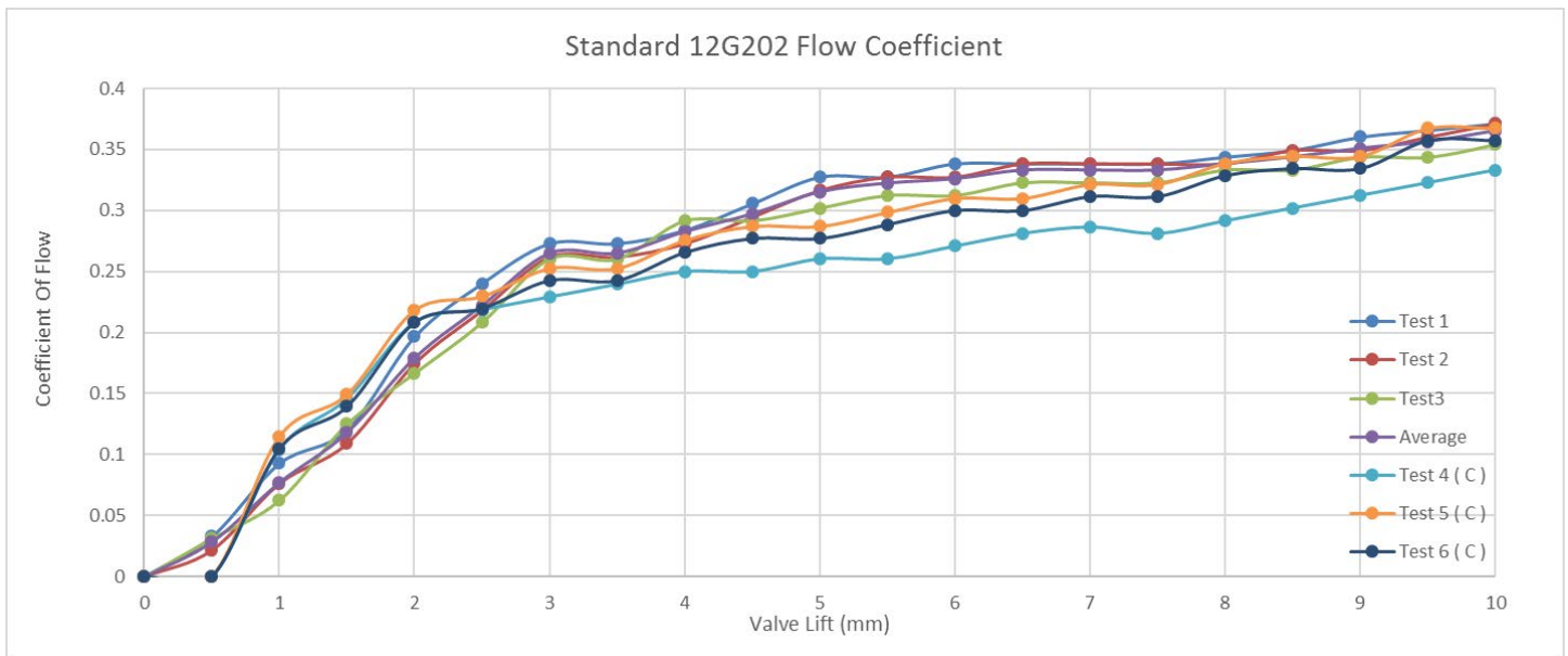
FIGURE 61: STANDARD FLOW COEFFICIENT RESULTS WITH CARBON BUILD UP
