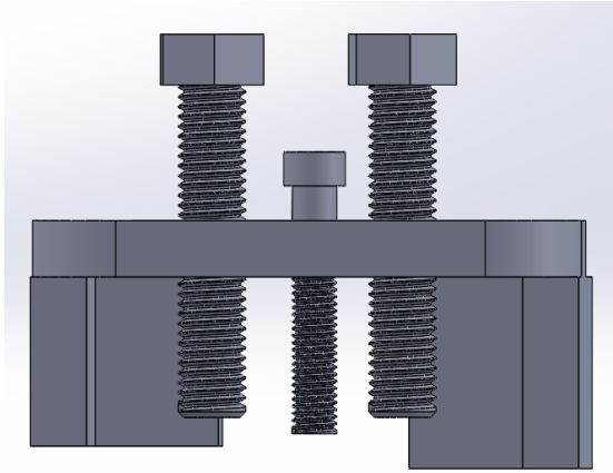
FIGURE 26: FRONT VIEW OF CAD VALVE OPENING TOOL
