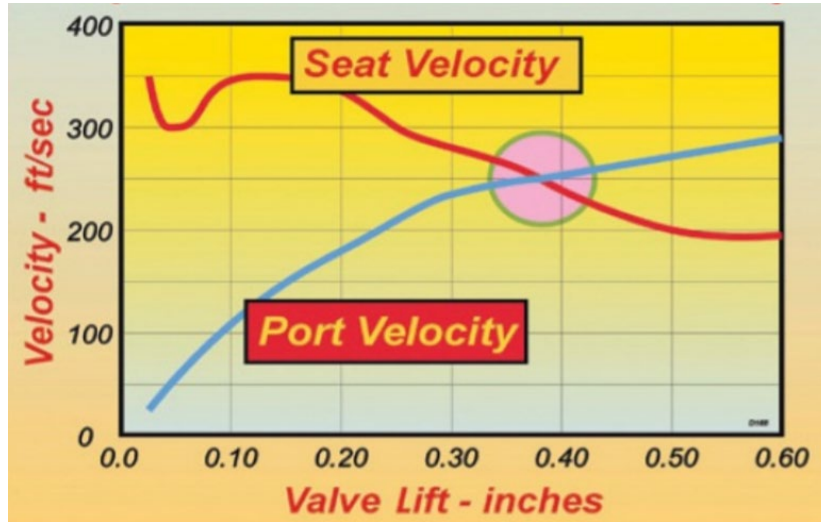
FIGURE 9: [5] SEAT AND PORT VELOCITY AS VALVE LIFT INCREASES
