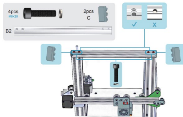
FIGURE 91: CREATILTY ENDER 3 ASSEMBLY GUIDE PART 10
