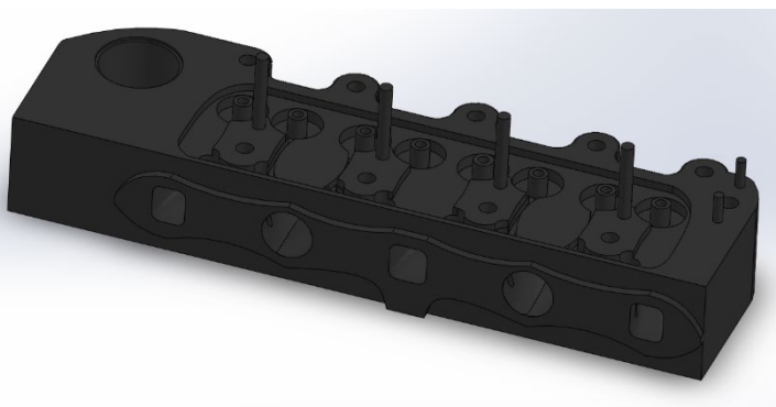
FIGURE 31: REAR VIEW OF 12G202 CYLINDER HEAD
