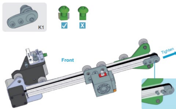
FIGURE 89: CREATILTY ENDER 3 ASSEMBLY GUIDE PART 8
