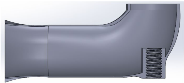
FIGURE 122: PORT 7 INCREASED SHORT TURN RAD AND LONG TURN RADIUS
