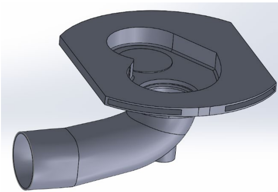
FIGURE 109: SIDE VIEW OF THE PHASE 3 PORT
