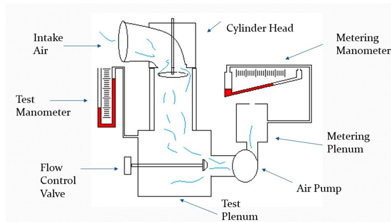
FIGURE 43: SIMPLIFIED DRAWING OF A FLOW BENCH
