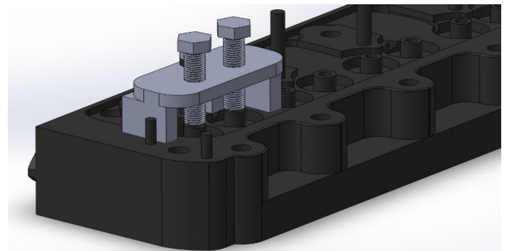
FIGURE 37: SIDE VIEW OF CAD CYLINDER HEAD WITH ADDED VALVE OPENING TOOL
