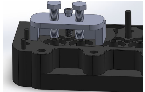
FIGURE 35 TOP FRONT VIEW OF CAD CYLINDER HEAD WITH ADDED VALVE OPENING TOOL
