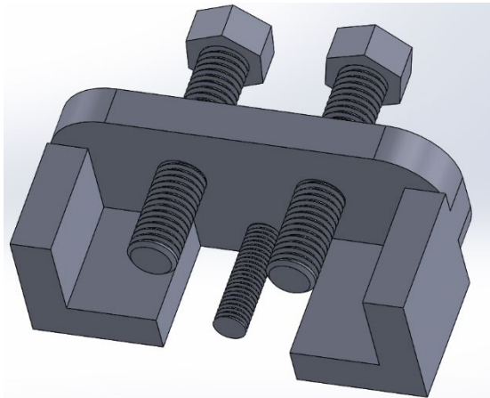
FIGURE 29: BOTTOM VIEW OF CAD VALVE OPENING TOOL
