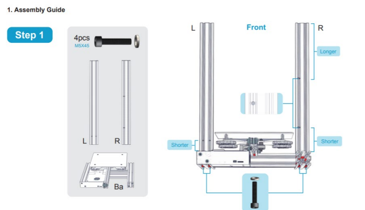
FIGURE 82: CREATILITY ENDER 3 ASSEMBLY GUIDE PART 1
