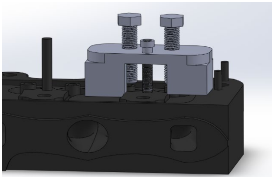
FIGURE 36: REAR VIEW OF CAD CYLINDER HEAD WITH ADDED VALVE OPENING TOOL
