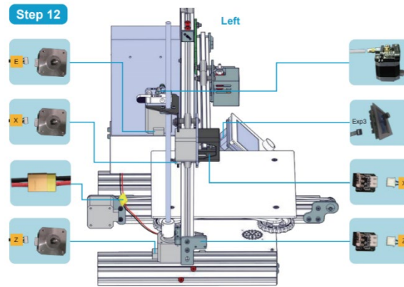
FIGURE 93: CREATILTY ENDER 3 ASSEMBLY GUIDE PART 12
