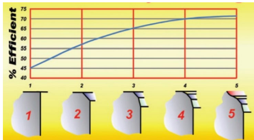
FIGURE 10: [5] FLOW EFFICIENCY INCREASE AS VALVE SEAT CURVATURE INCREASES
