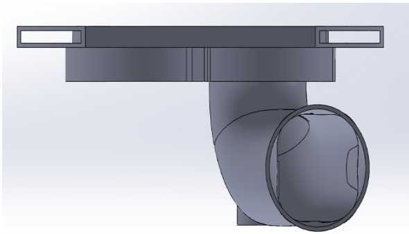
FIGURE 107: FRONT VIEW OF THE PHASE 3 PORT
