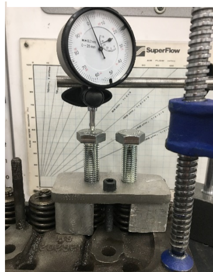
FIGURE 51: CLOSE UP OF DTI GAUGE
