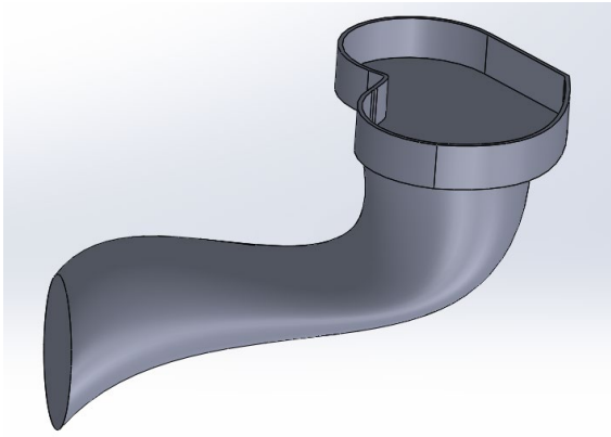
FIGURE 67: MINI PORT WITH CURVED FLOOR AND CEILING
