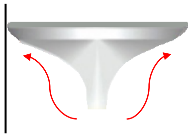
FIGURE 12: SIMPLIFIED EXAMPLE OF POOR VALVE SHROUDING
