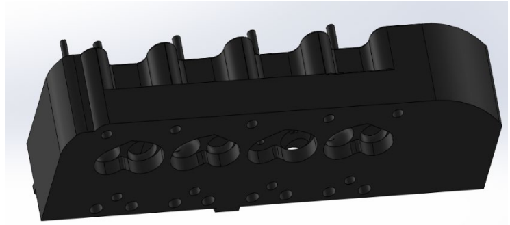
FIGURE 33: VIEW OF BOTTOM AND REAR OF CAD CYLINDER HEAD
