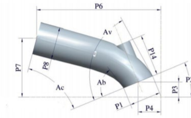
FIGURE 6: [3] STRUCTURAL PARAMETERS OF AN INLET PORT
