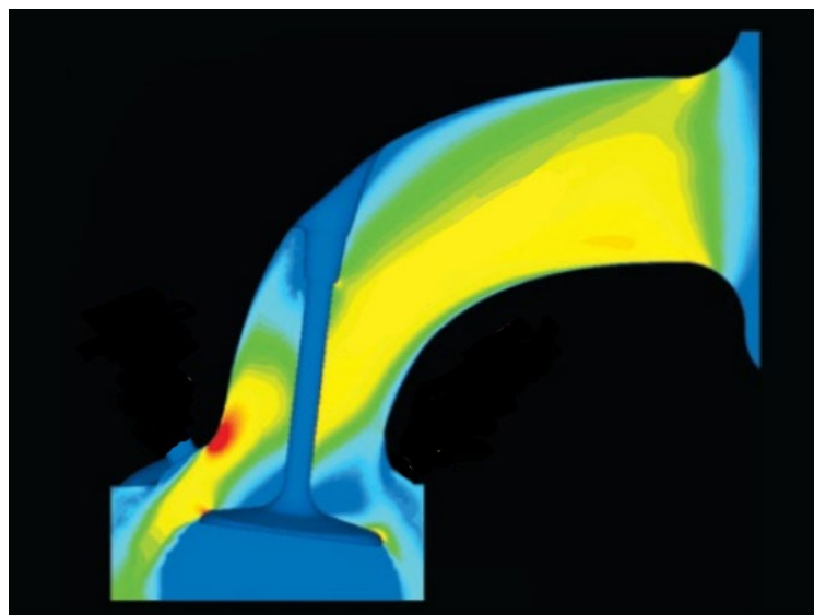
FIGURE 8: [5] CFD IMAGE OF AIR FLOW THROUGH INLET PORT
