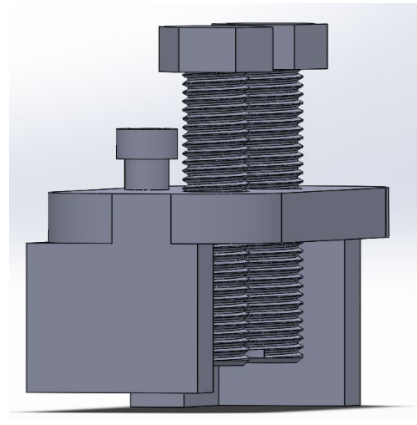
FIGURE 27: SIDE VIEW OF CAD VALVE OPENING TOOL
