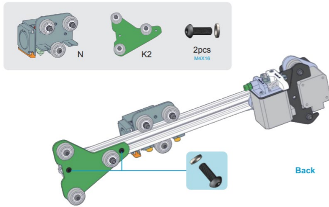
FIGURE 87: CREATILTY ENDER 3 ASSEMBLY GUIDE PART 6
