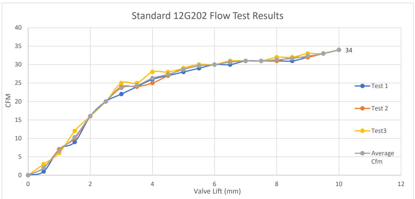
FIGURE 57: STANDARD FLOW TEST RESULTS
