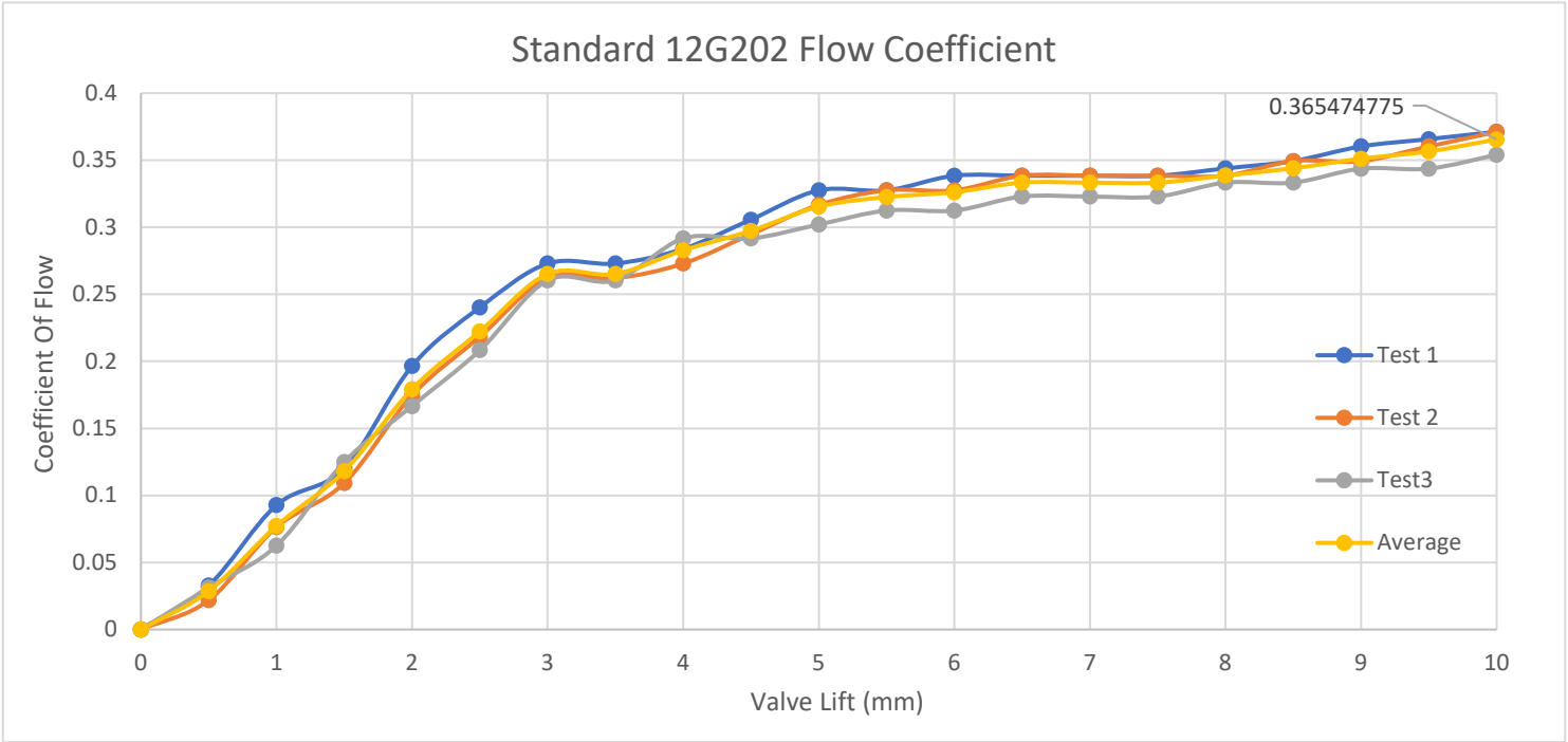
FIGURE 59: STANDARD FLOW TEST COEFFICIENT RESULTS
