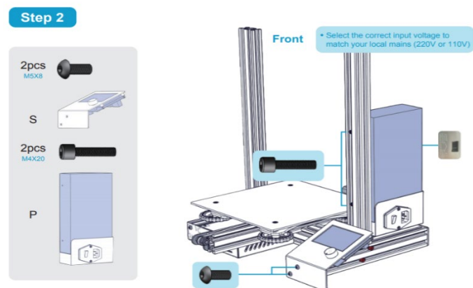
FIGURE 83: CREATILITY ENDER 3 ASSEMBLY GUIDE PART 2
