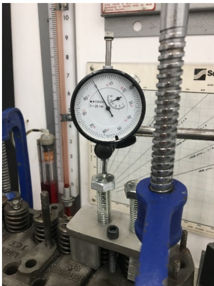
FIGURE 53: DTI WITH VALVE CLOSED
