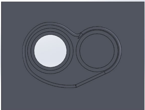
FIGURE 127: COMBUSTION CHAMBER 2 , REDUCED SHROUD 2
