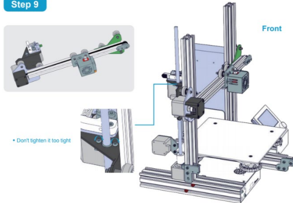
FIGURE 90: CREATILTY ENDER 3 ASSEMBLY GUIDE PART 9
