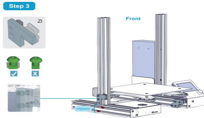
FIGURE 84: CREATILITY ENDER 3 ASSEMBLY GUIDE PART 3
