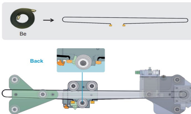
FIGURE 88: CREATILTY ENDER 3 ASSEMBLY GUIDE PART 7
