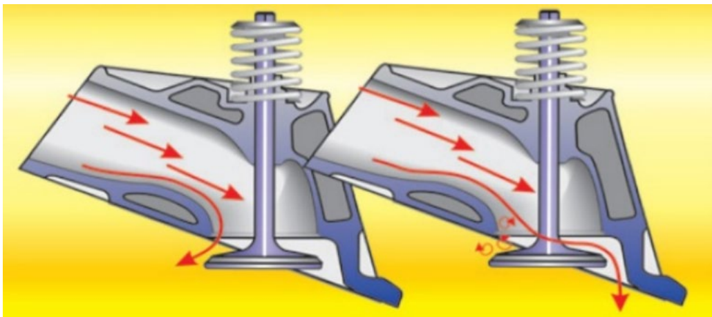
FIGURE 7: [5] AIR PASSING OVER SHORT AND LONG TURN RADIUS
