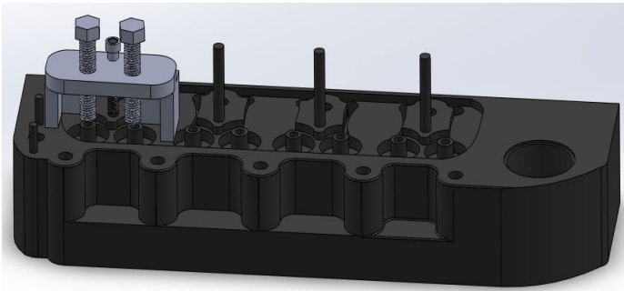
FIGURE 32: VIEW OF BOTTOM OF CAD CYLINDER HEAD
