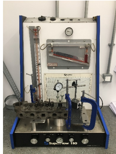
FIGURE 55: FINAL SETUP OF TEST EQUIPMENT
