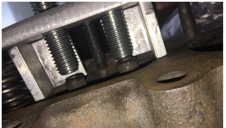
FIGURE 42: VALVE TOOL SAT ON TOP OF VALVE GUIDES
