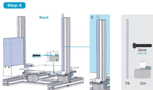
FIGURE 85: CREATILITY ENDER 3 ASSEMBLY GUIDE PART 4
