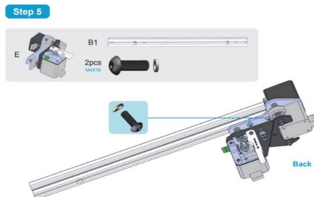
FIGURE 86: CREATILITY ENDER 3 ASSEMBLY GUIDE PART 5
