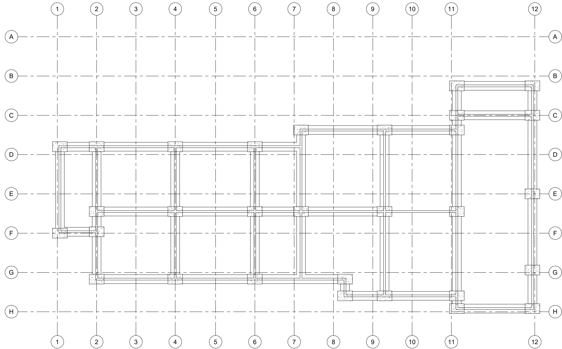
1 Foundations Plan 1 : 100
