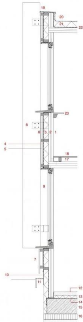
FACADE DETAIL
