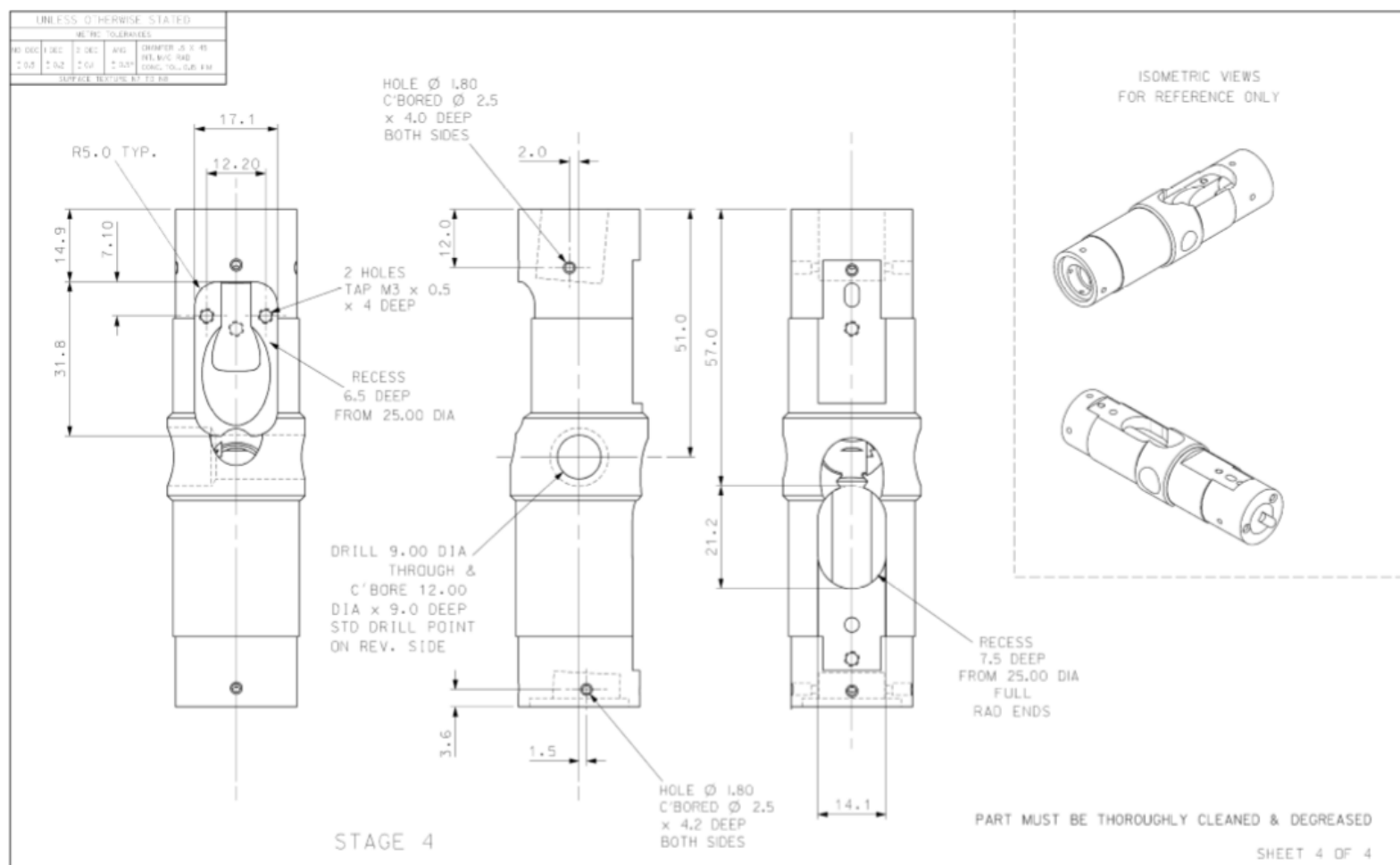
Figure 19 Drawing 4 of Z fold (PerkinElmer, 2018)
