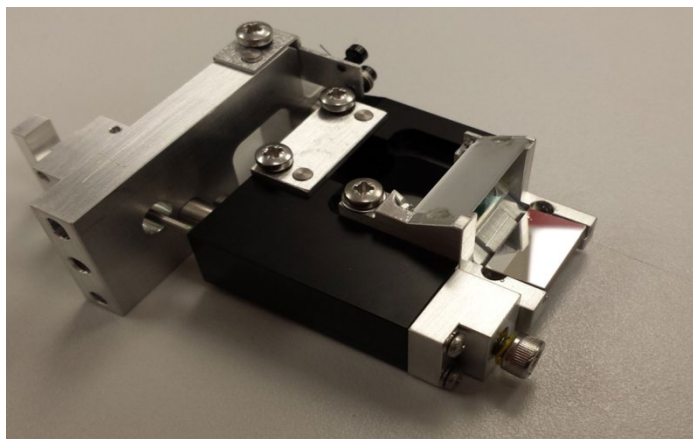
Figure 12 - 0292 Subassembly (PerkinElmer, 2018)
