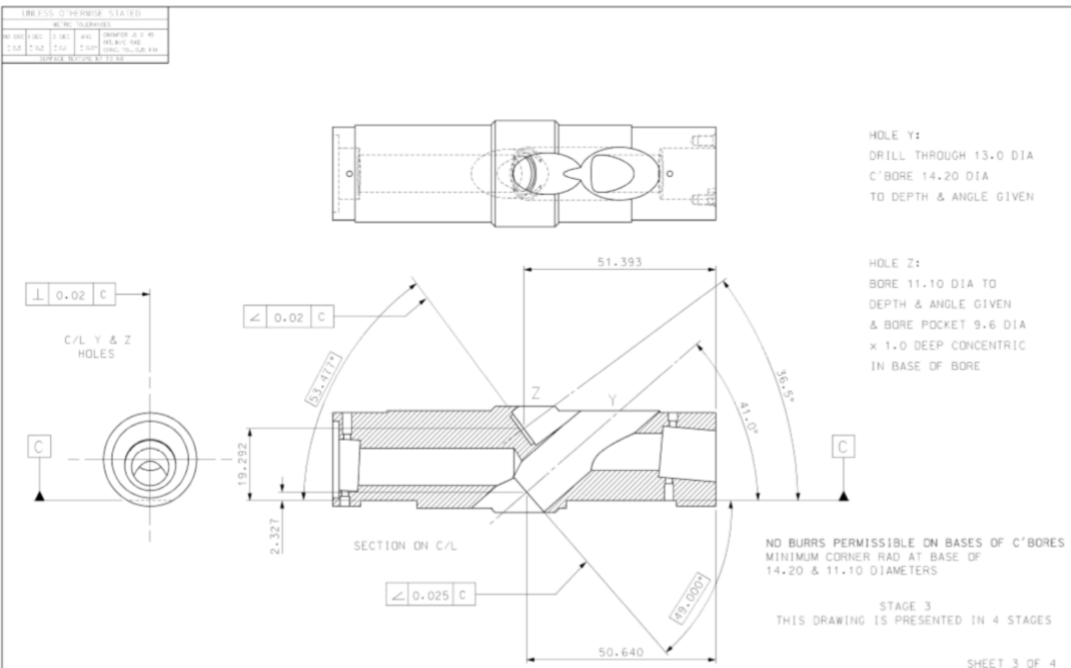
Figure 17 Drawing 3 of Z fold (PerkinElmer, 2018)
