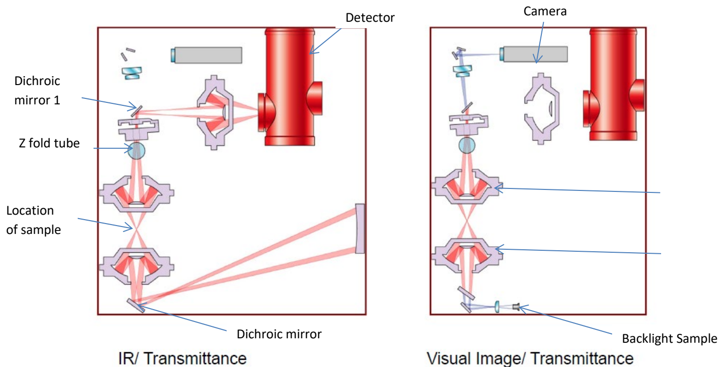
Figure 8 Optical system Within a Spotlight 400 on Transmittance Mode (Suzanne McFarlane, 2009)
