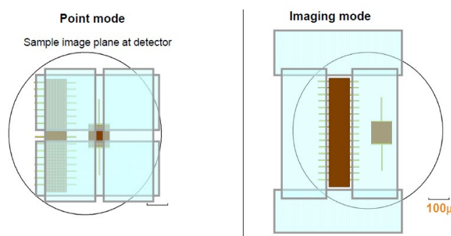
Figure 7: Detector mode selection (Wita, 2014)
