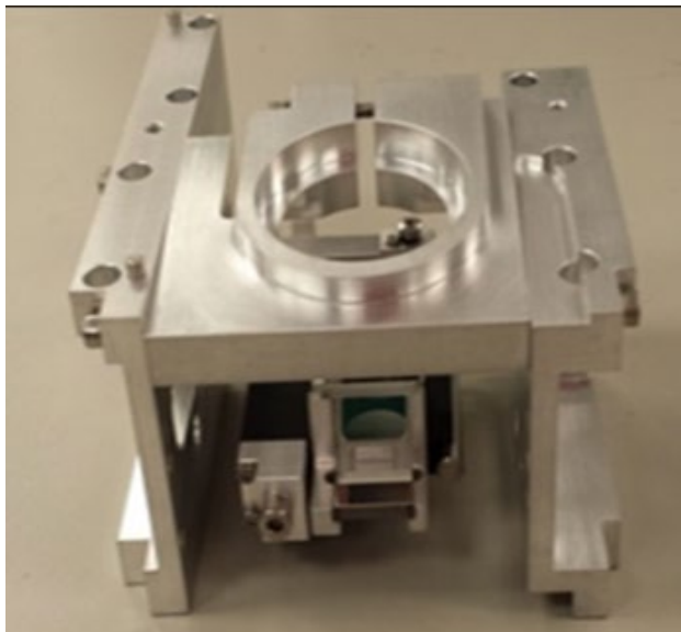
Figure 13 - Subassembly 0309 (PerkinElmer, 2018)
