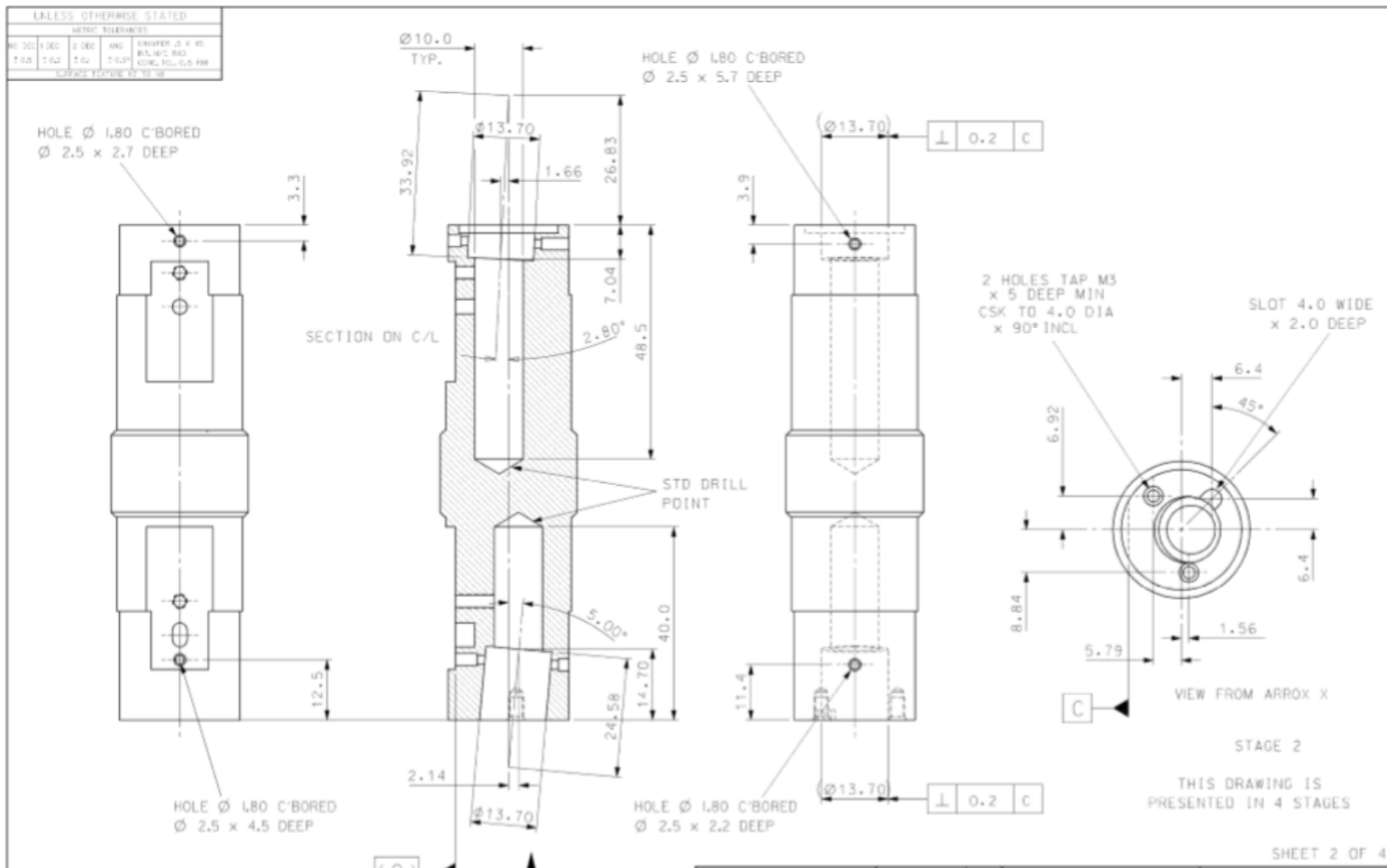
Figure 16 Drawing 2 of Z fold (PerkinElmer, 2018)
