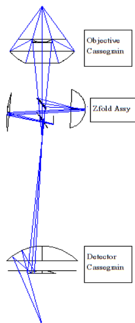
Figure 21 Instrument Light Path
