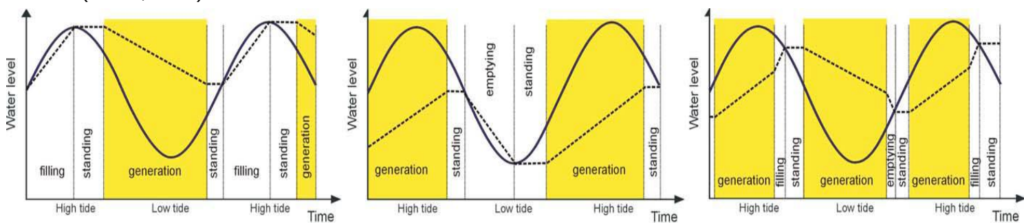
Figure 8--Ebb Production (left), Flow production (centre), Bidirectional production (right). Solid curve is sea water level, dotted line is basin water level. (Bae, et al., 2010)
