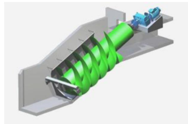
Figure 16-Archimedes Screw for Power Generation. (Waters & Aggidis, 2016)
