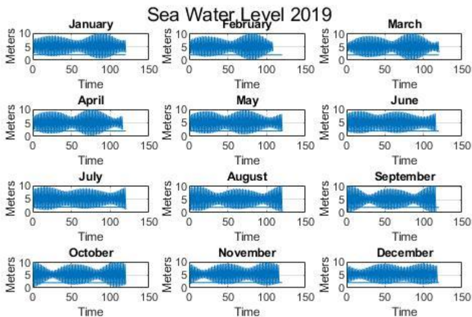
Figure 38-Sea Water Level 2019. Line at y=2 to show losses from elevated basin
