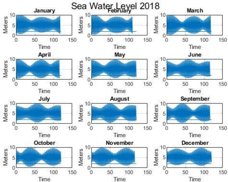
Figure 37-Sea Water Level 2018. Line at y=2 to show losses from elevated basin
