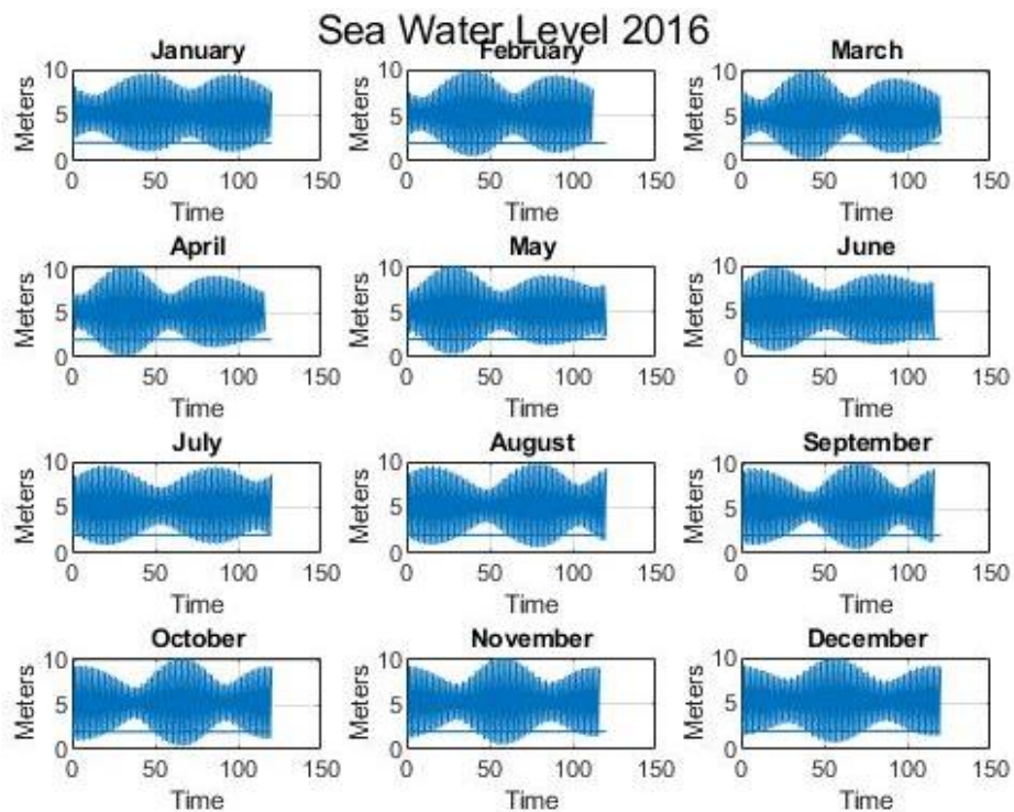
Figure 35-Sea Water Level 2016. Line at y=2 to show losses from elevated basin
