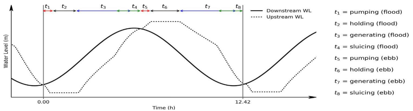
Figure 9-optimised generation output from tidal range scheme using pumping. (Angeloudis, et al., 2018)
