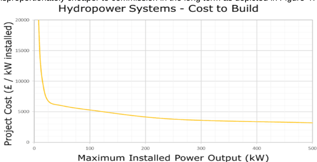
Figure 47- Hydropower build cost by size. (Renewables First, 2015)
