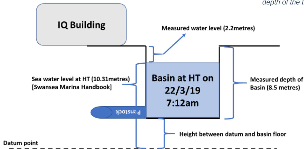
Figure 31- Apparatus used to measure the depth of the tidal basin
