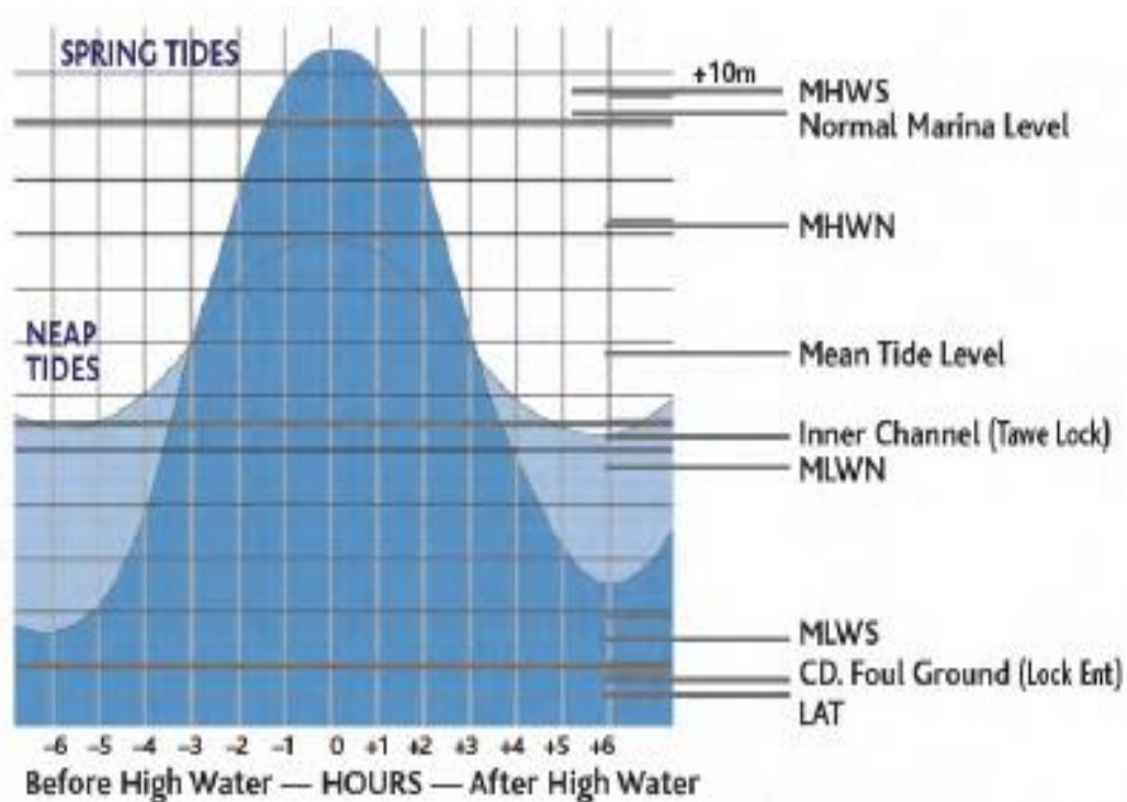
Figure 27- Datum Point is at LAT (Lowest Astronomical Tide). Swansea Marina Handbook 2015
