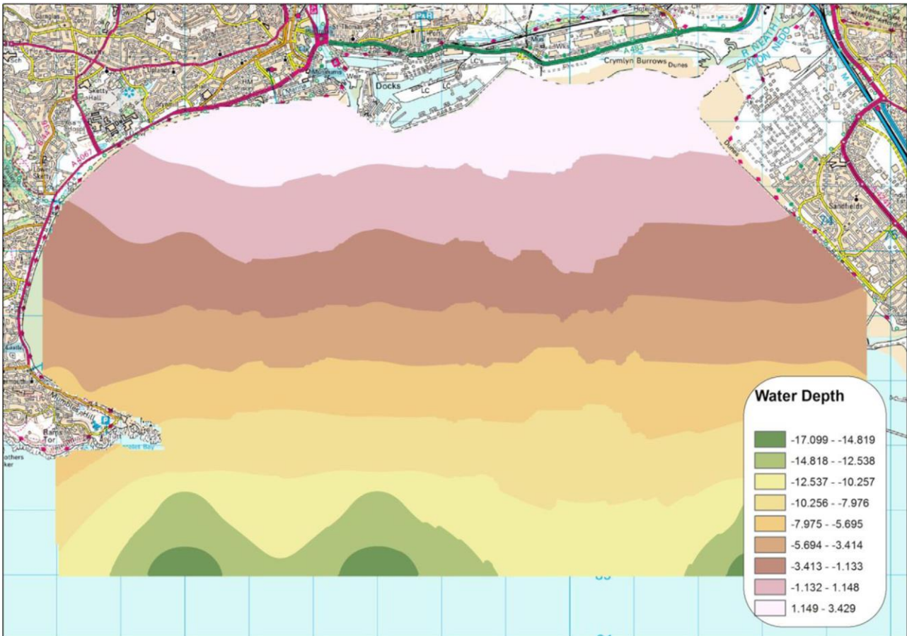
Figure 33- Inverse Distance Weighting surface at mean sea level (metres). (Petley & Aggidis, 2016)
