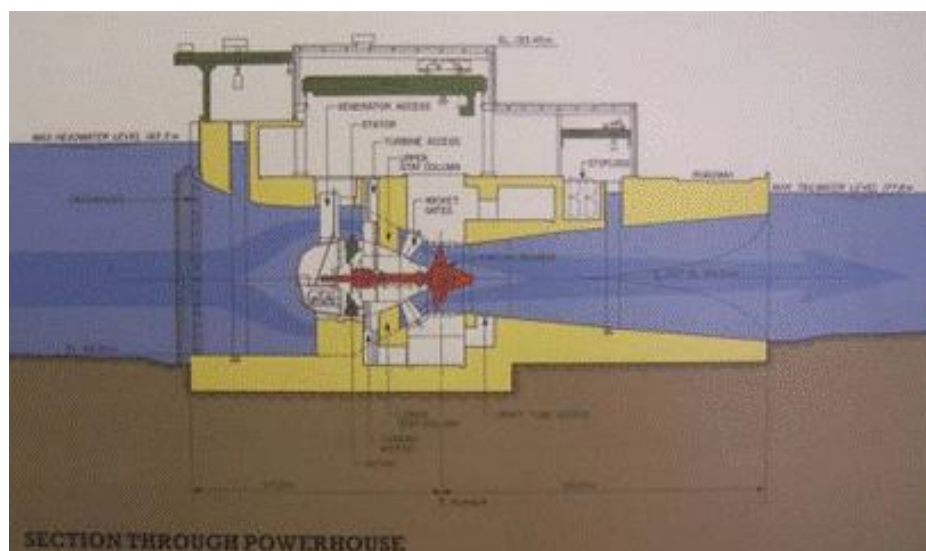
Figure 17- Kaplan Bulb turbine. (Renewables First, 2015)
