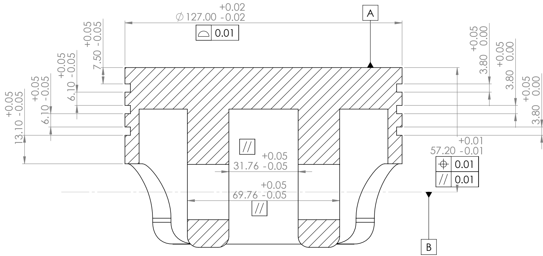
SECTION C-C
