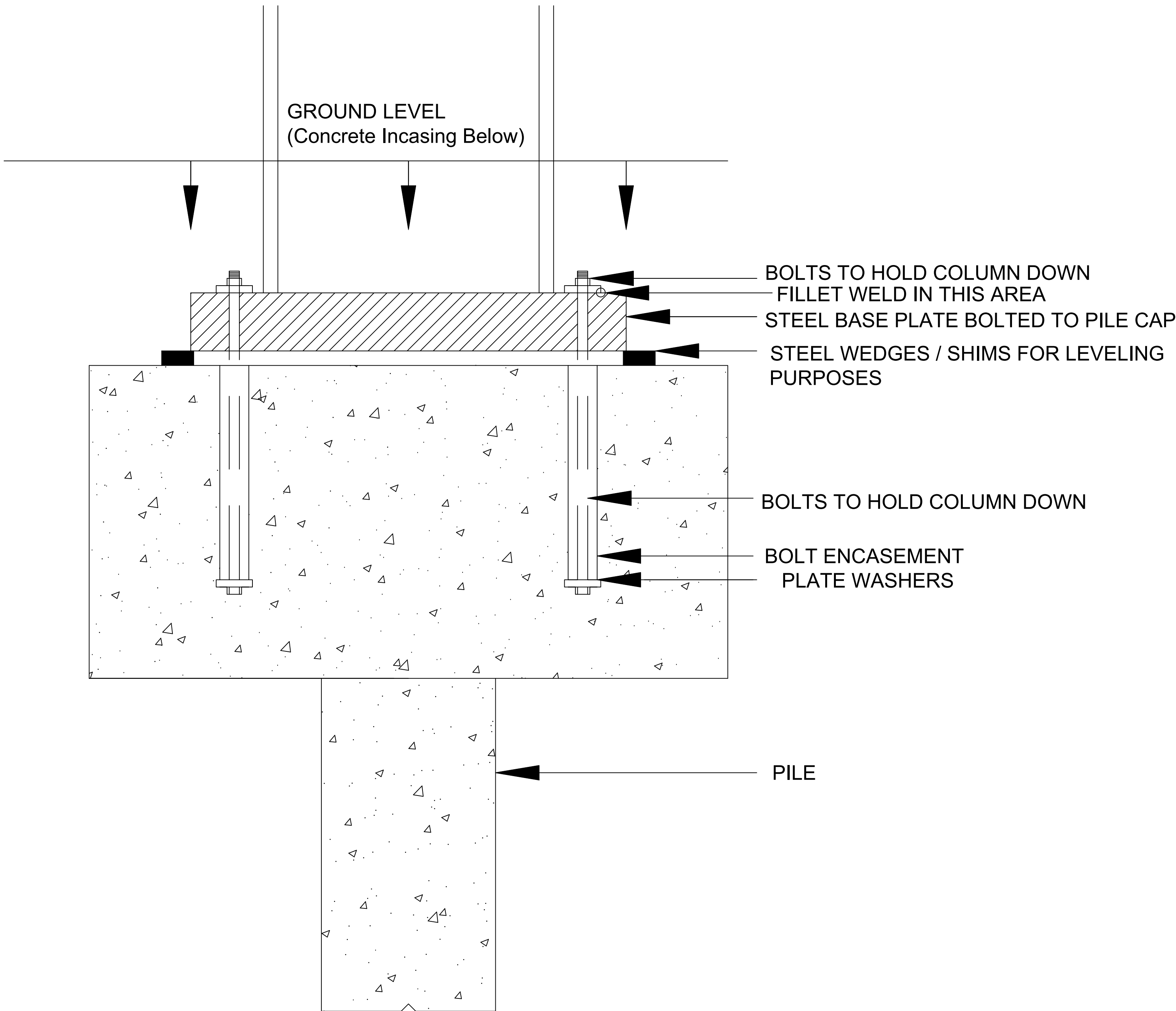
STEEL COLUMN TO PILE FOUNDATION CONNECTION
